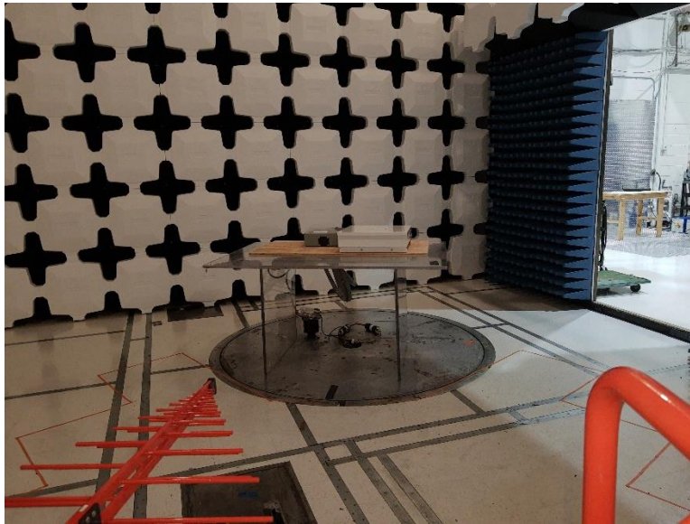
Photograph 2. REE Test Setup, 30-1000 MHz
