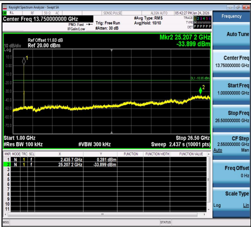
11AX20SISO-Ant1-2437-1000~26500-PASS
