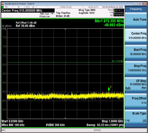
11AX20SISO-Ant1-2412-30~1000-PASS
