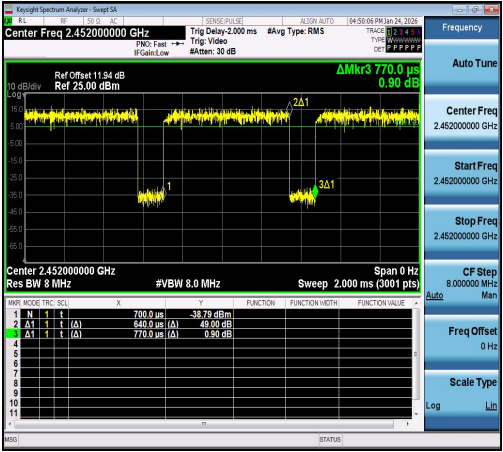
NTNV-11N40SISO-Ant1-2452
