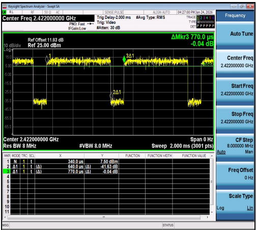
NTNV-11N40SISO-Ant1-2422
