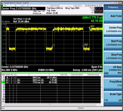
NTNV-11N40SISO-Ant1-2437
