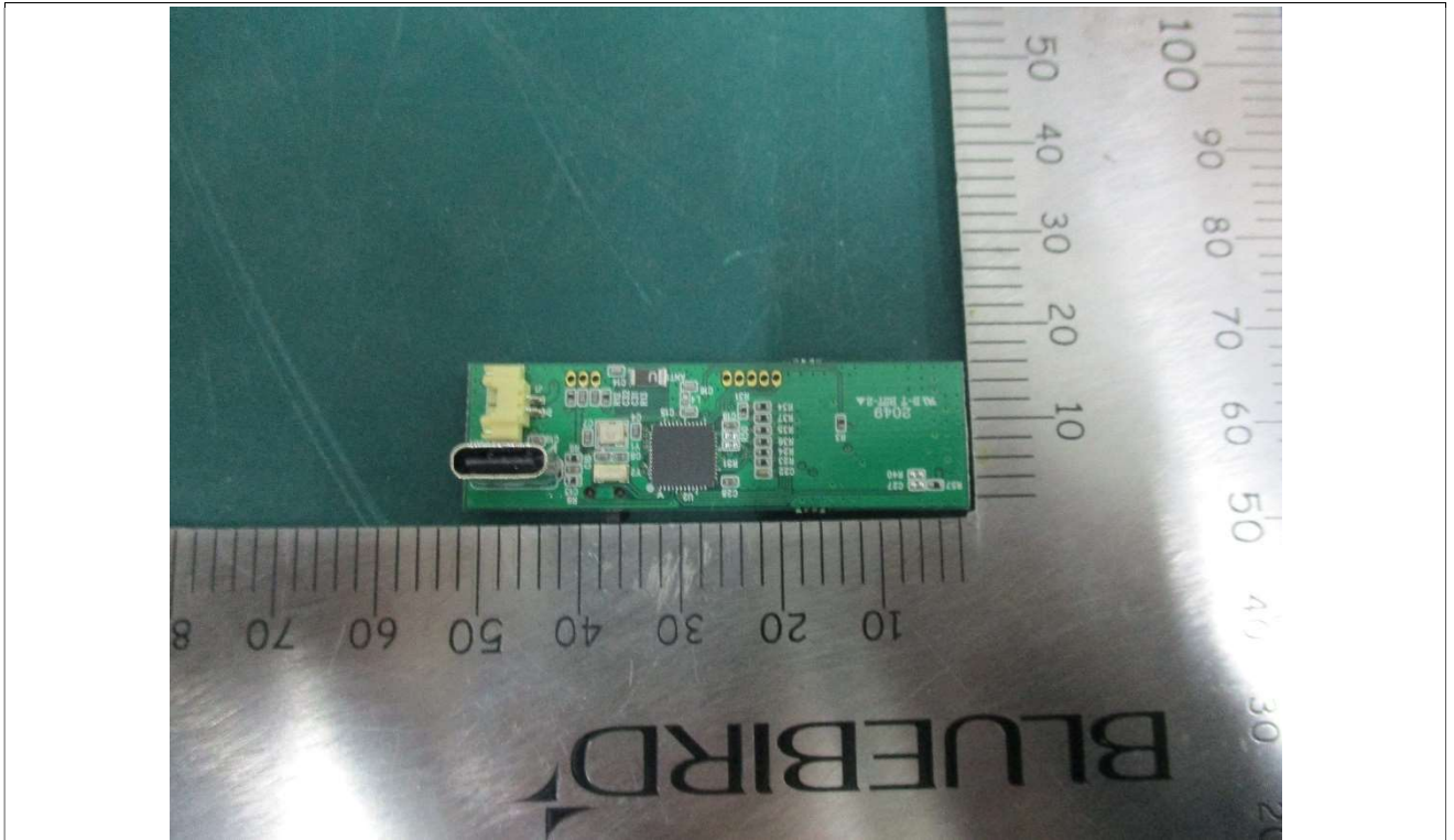
Main Board_Rear
