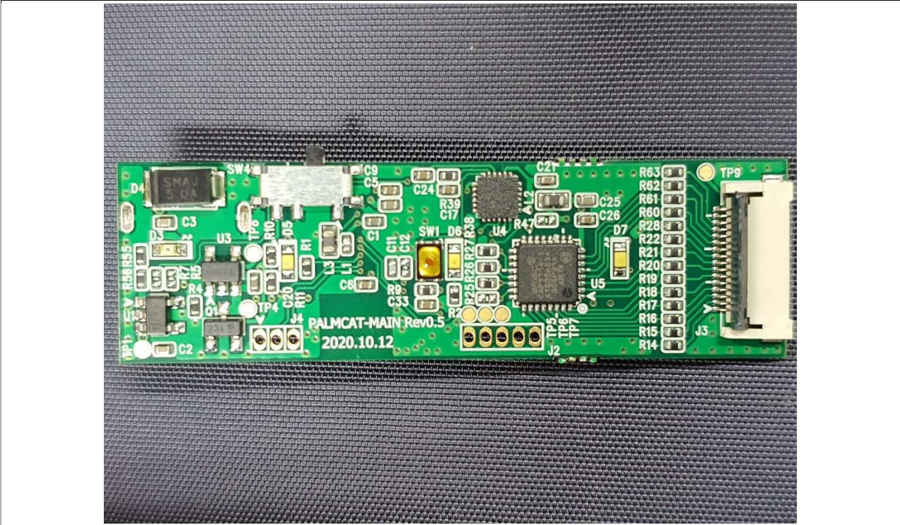
Main Board_Front
