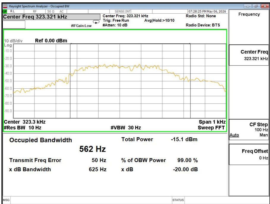
323-328KHz Coil Antenna 3
