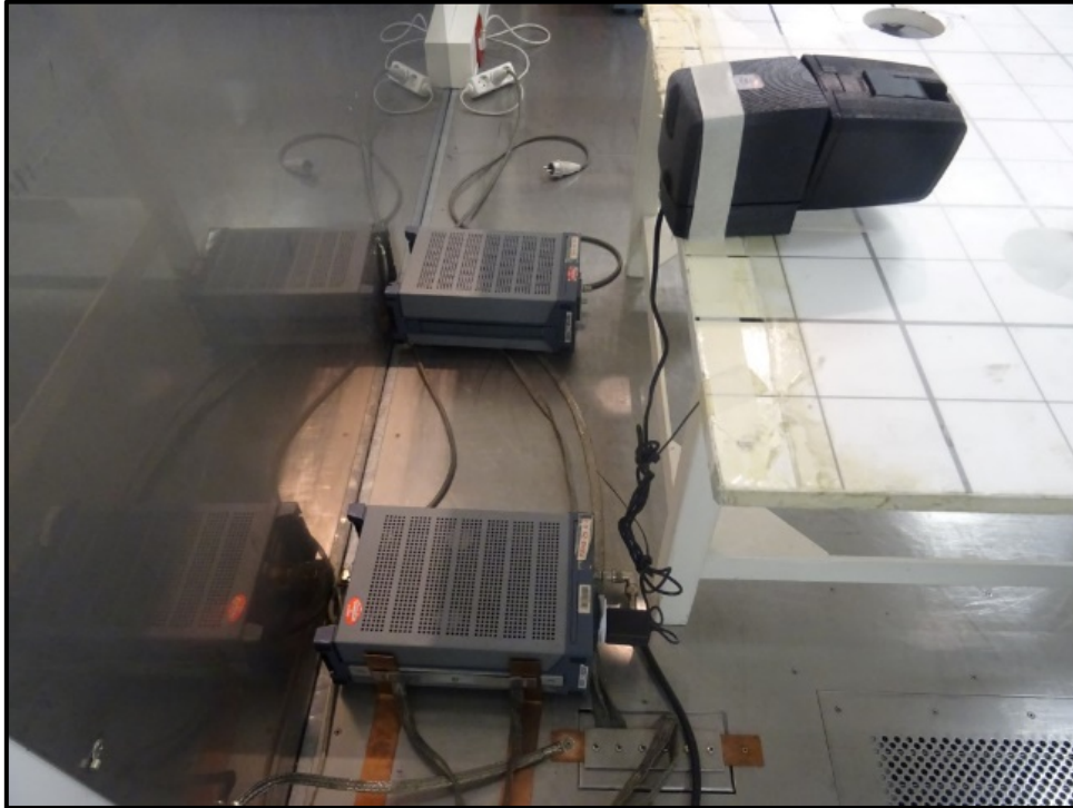
Photo 1: Conducted Test Setup from 150 kHz to 30 MHz
