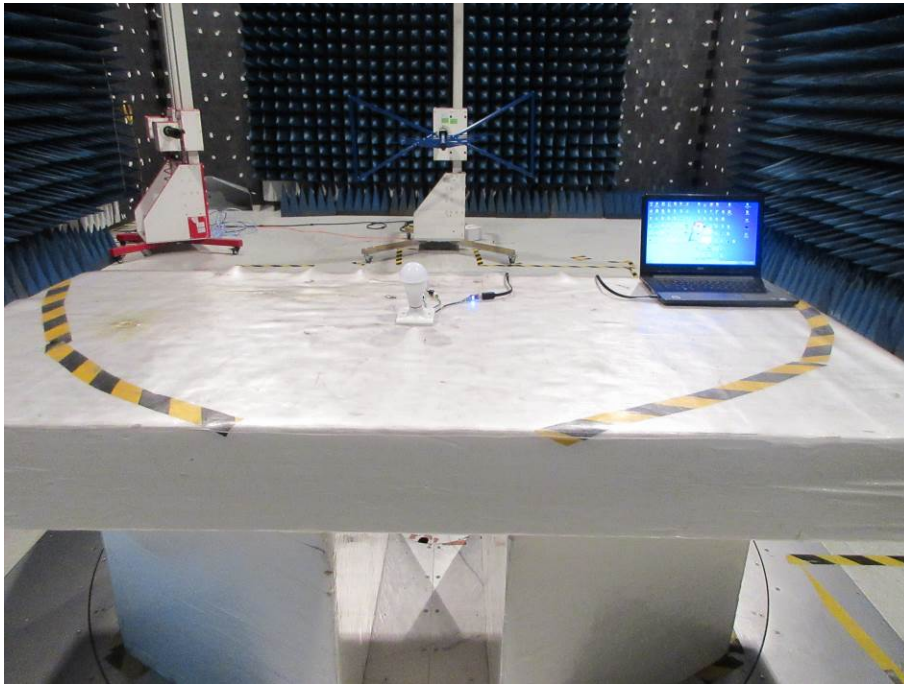
Radiated Spurious Emission 30MHz ~ 1000MHz
