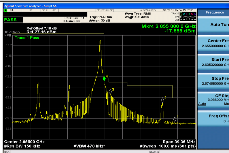
Band41-15MHz-QPSK-41165-1RB#74
