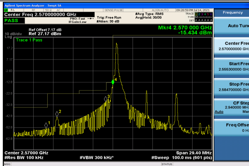
Band38-10MHz-16QAM-37800-1RB#0
