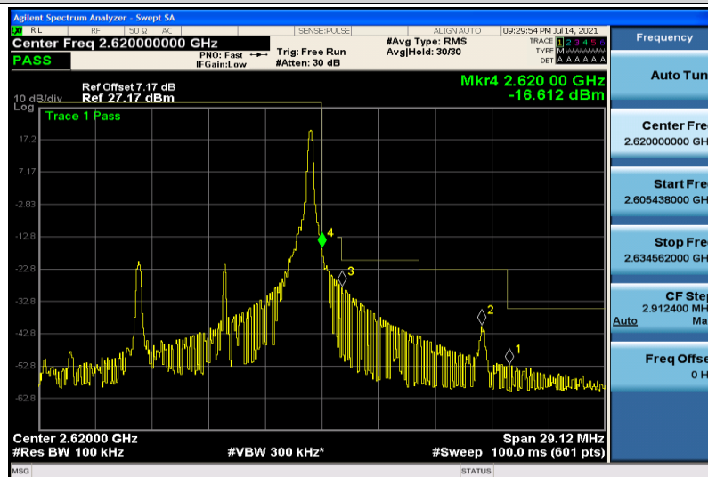
Band38-10MHz-16QAM-38200-1RB#49
