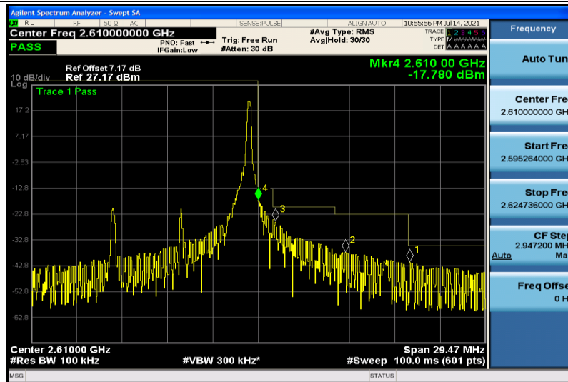
Band41-10MHz-QPSK-40740-1RB#49
