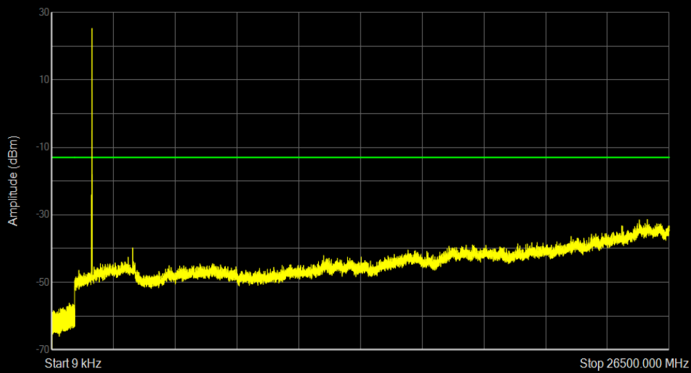
Band66 QAM16 BW=3MHz Channel=132322 RB Size=15 Position=#0
