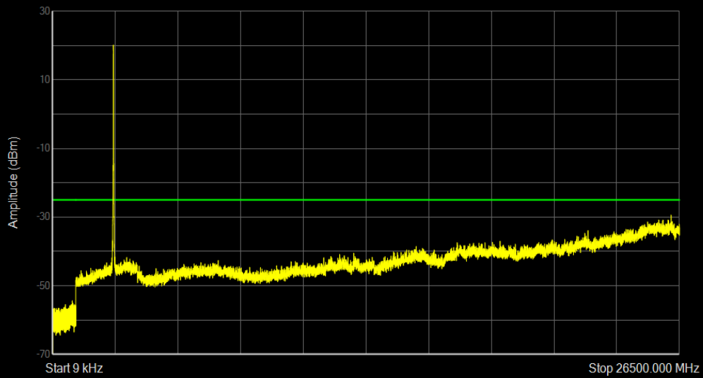
Band41 QAM16 BW=15MHz Channel=40620 RB Size=75 Position=#0
