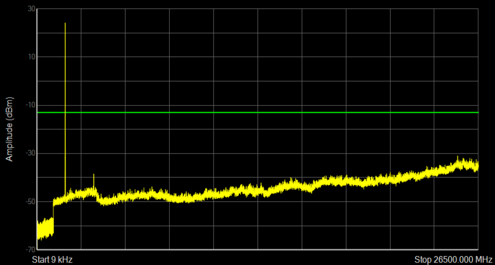
Band66 QAM16 BW=5MHz Channel=131997 RB Size=25 Position=#0
