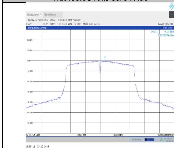
11ac40SISO-Ant9-5795-PASS
