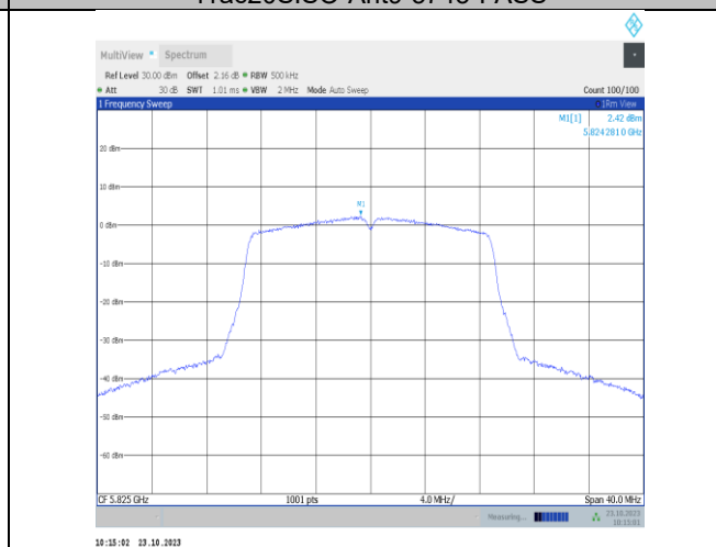
11ac20SISO-Ant9-5825-PASS
