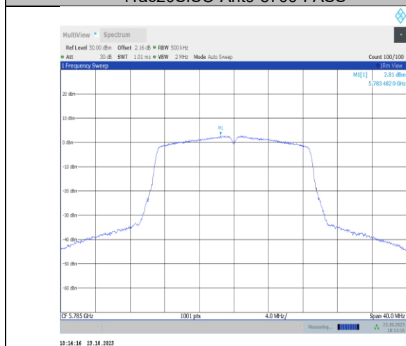
11ac20SISO-Ant9-5785-PASS
