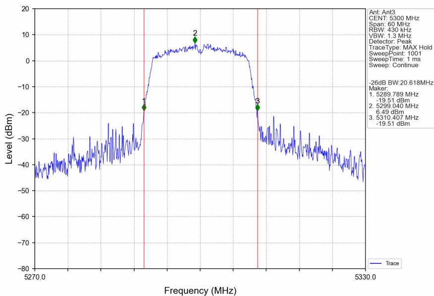
802.11ac(VHT20)_MCH_5300MHz_Ant3_NTNV
