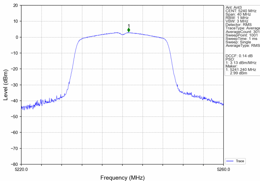
802.11n(HT20)_HCH_5240MHz_Ant3_NTNV
