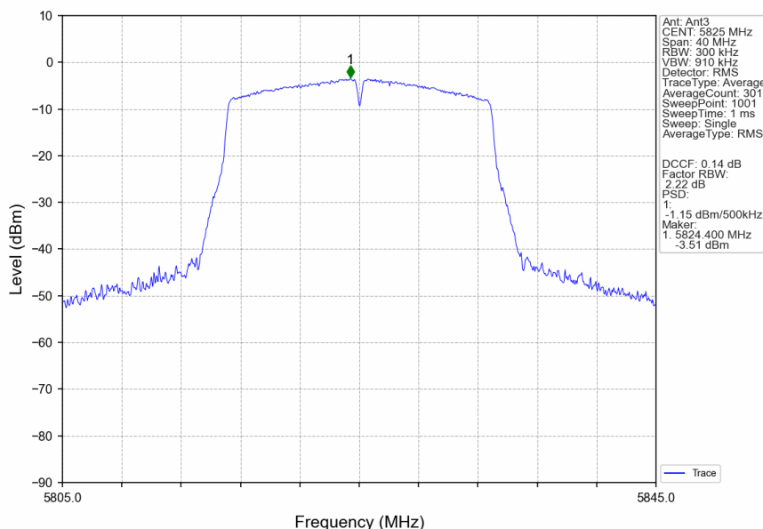
802.11n(HT20)_HCH_5825MHz_Ant3_NTNV
