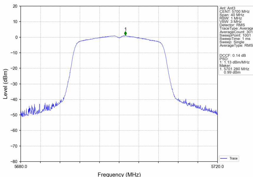
802.11n(HT20)_HCH_5700MHz_Ant3_NTNV
