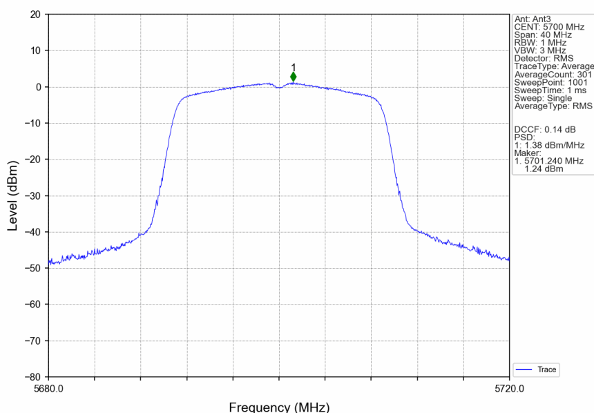
802.11ac(VHT20)_HCH_5700MHz_Ant3_NTNV
