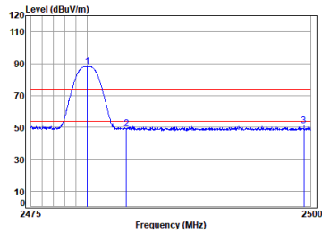
BLE_1M_TX_CH_39_Horizontal
