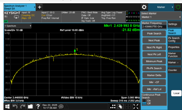
GFSK (BLE 2Mbps) MIDDLE CHANNEL
