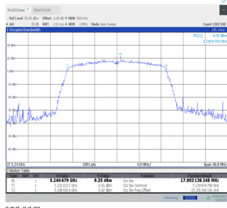
11ac20SISO-Ant11-5240
