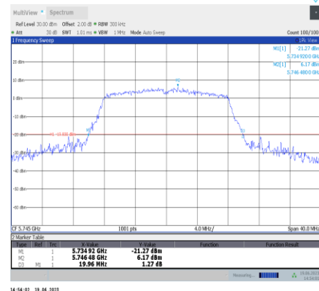
11a-Ant11-5745
