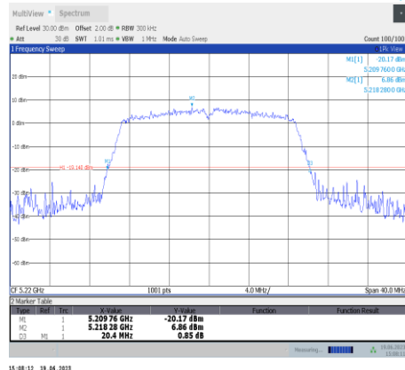
11ac20SISO-Ant11-5220
