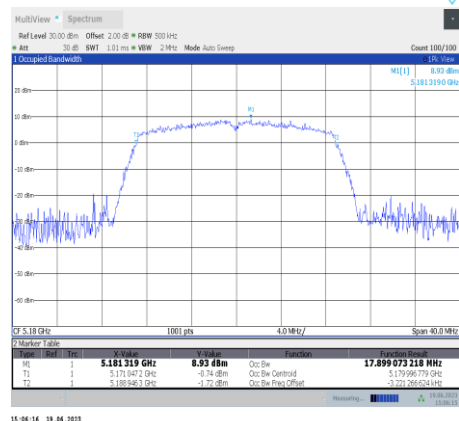
11ac20SISO-Ant11-5180
