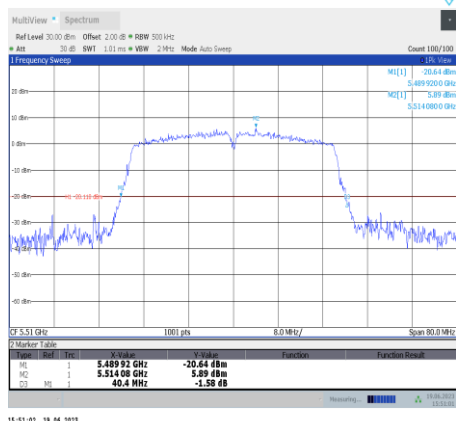
11ac40SISO-Ant11-5510
