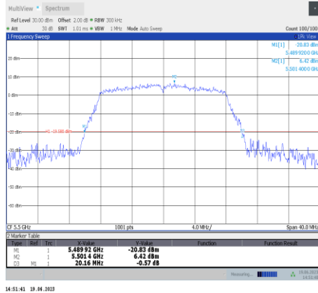
11a-Ant11-5500
