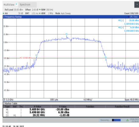
11ac20SISO-Ant11-5500
