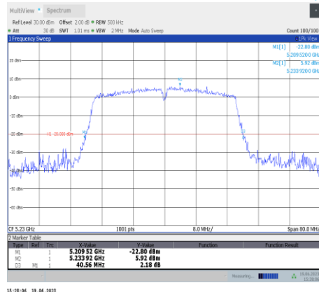
11ac40SISO-Ant11-5230
