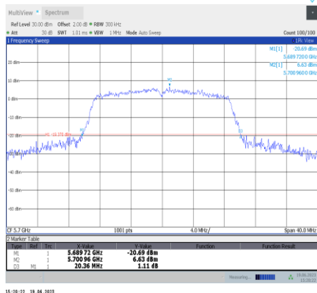
11ac20SISO-Ant11-5700
