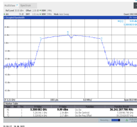
11ac40SISO-Ant11-5310
