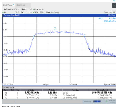
11ac20SISO-Ant11-5785
