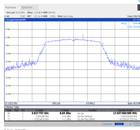
11a-Ant11-5825
