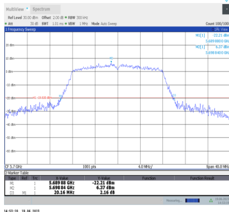
11a-Ant11-5700
