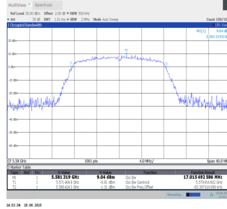
11a-Ant11-5580
