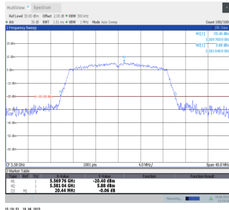
11ac20SISO-Ant11-5580
