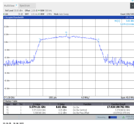
11ac20SISO-Ant11-5580
