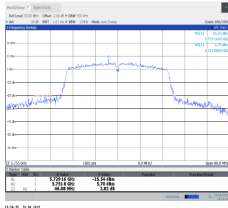
11ac40SISO-Ant11-5755
