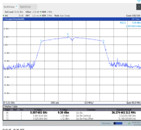
11ac40SISO-Ant11-5510
