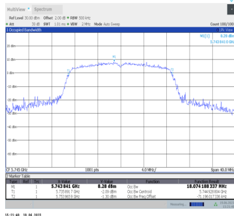
11ac20SISO-Ant11-5745
