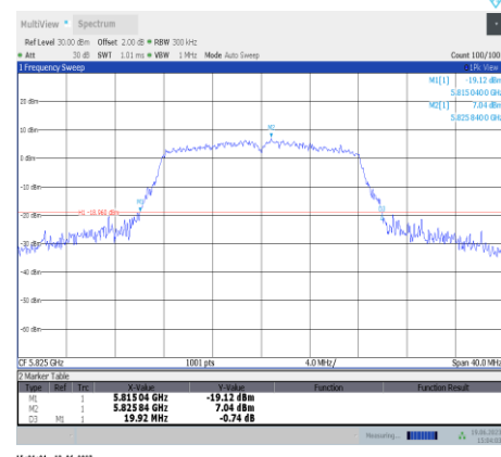
11a-Ant11-5825
