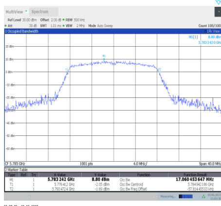
11a-Ant11-5785
