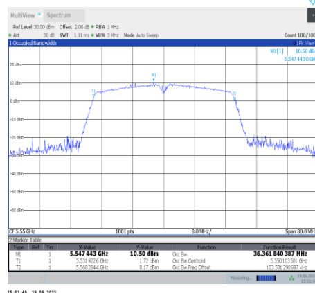
11ac40SISO-Ant11-5550
