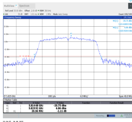
11ac20SISO-Ant11-5825
