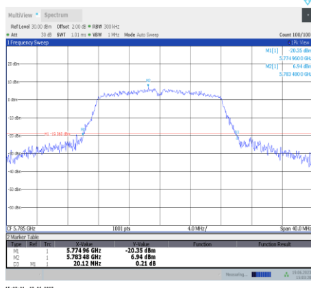
11a-Ant11-5785
