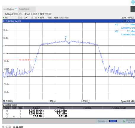
11ac20SISO-Ant11-5300
