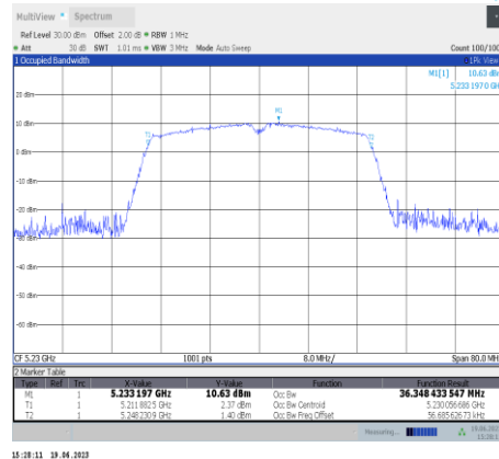
11ac40SISO-Ant11-5230
