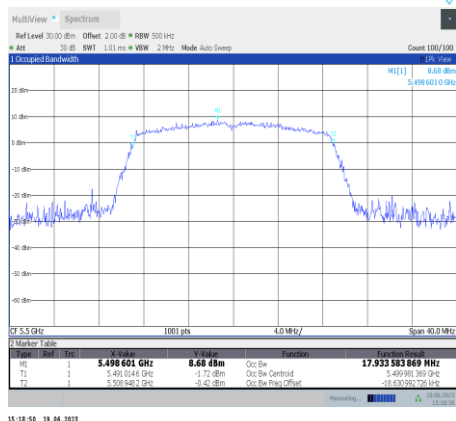
11ac20SISO-Ant11-5500
