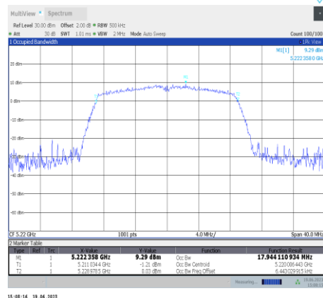
11ac20SISO-Ant11-5220
