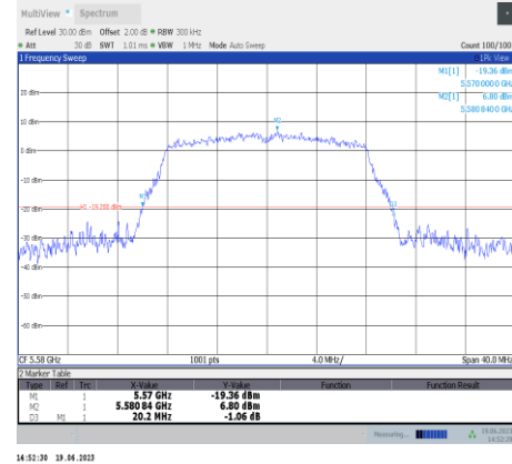
11a-Ant11-5580
