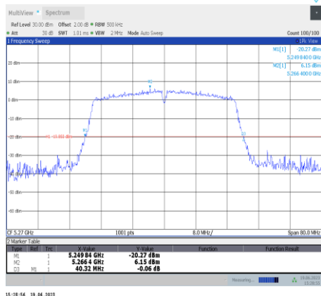
11ac40SISO-Ant11-5270
