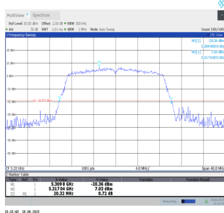
11ac20SISO-Ant11-5320
