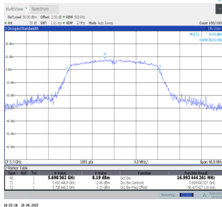
11a-Ant11-5700
