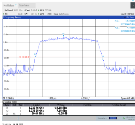
11ac20SISO-Ant11-5240
