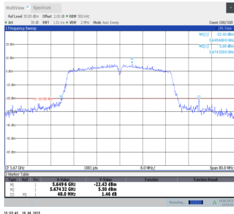
11ac40SISO-Ant11-5670
