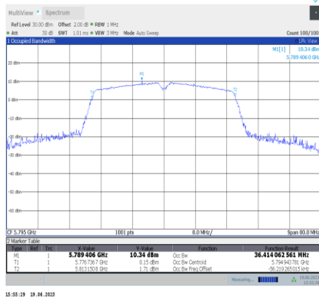
11ac40SISO-Ant11-5795
