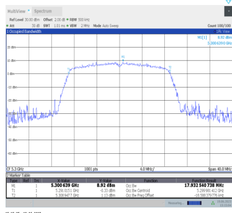
11ac20SISO-Ant11-5300
