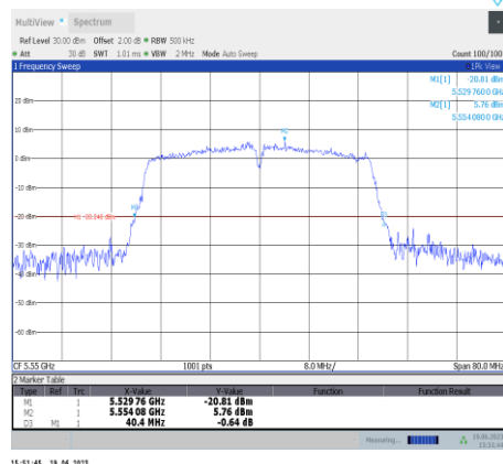
11ac40SISO-Ant11-5550
