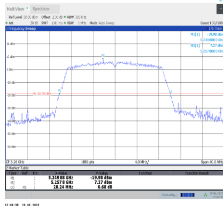
11ac20SISO-Ant11-5260
