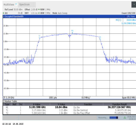
11ac40SISO-Ant11-5190
