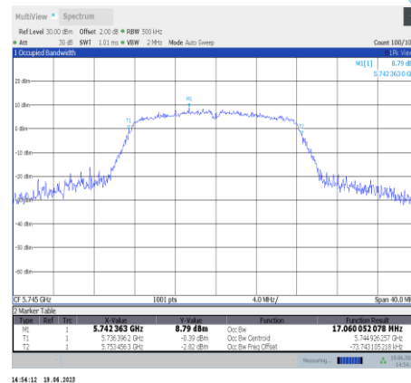
11a-Ant11-5745
