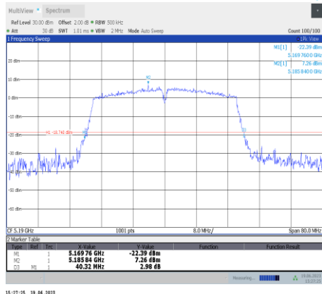
11ac40SISO-Ant11-5190
