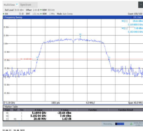
11ac20SISO-Ant11-5180
