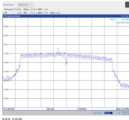
11n20SISO-Ant9-2462
