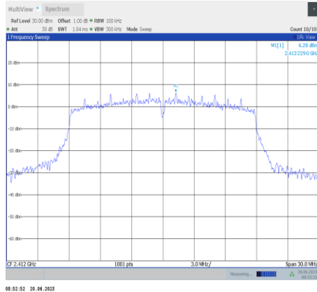
11n20SISO-Ant9-2412-0~Reference
