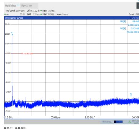
11b-Ant9-2437-1000~26500
