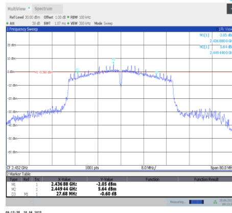
11n40SISO-Ant9-2452
