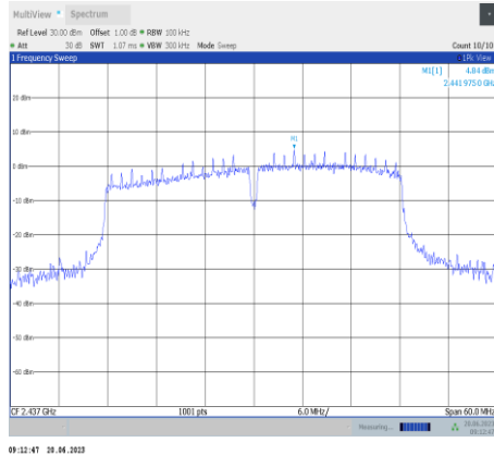
11n40SISO-Ant9-2437-0~Reference
