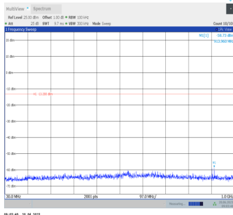
11n20SISO-Ant9-2437-30~1000
