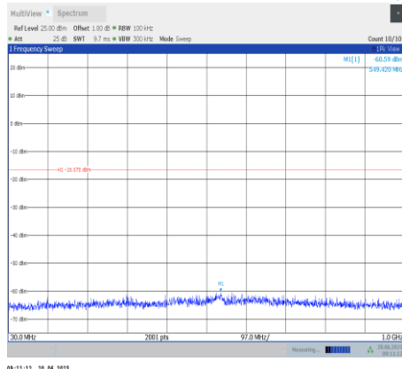
11n40SISO-Ant9-2422-30~1000
