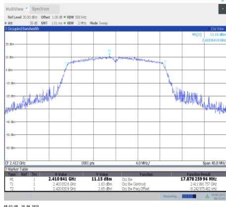
11n20SISO-Ant9-2412
