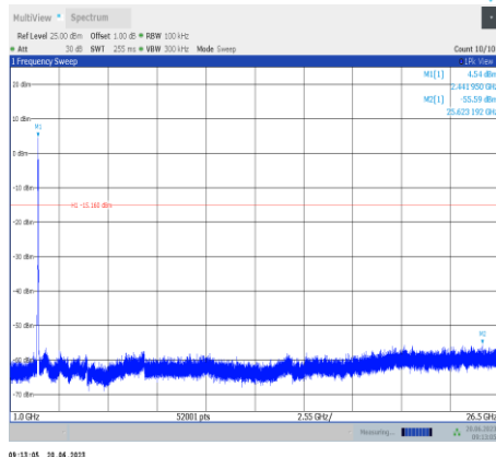
11n40SISO-Ant9-2437-1000~26500
