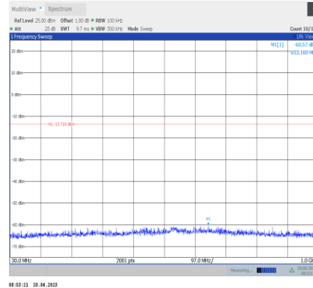
11n20SISO-Ant9-2412-30~1000
