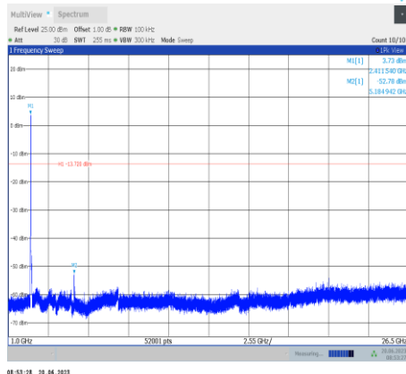
11n20SISO-Ant9-2412-1000~26500
