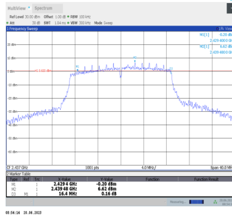
11n20SISO-Ant9-2437
