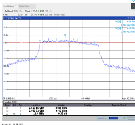
11n20SISO-Ant9-2462
