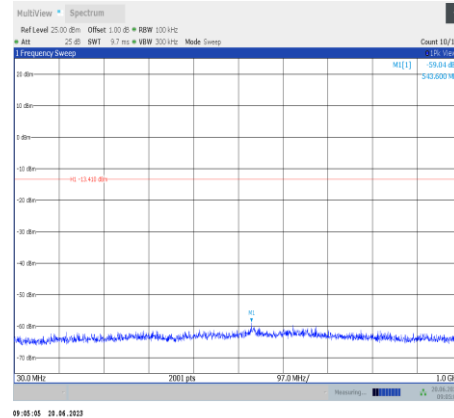
11n20SISO-Ant9-2462-30~1000
