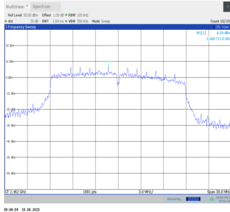
11n20SISO-Ant9-2462-0~Reference
