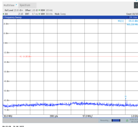
11n40SISO-Ant9-2452-30~1000
