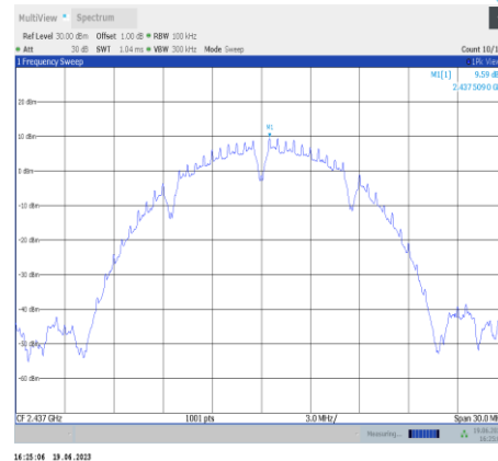
11b-Ant9-2437-0~Reference
