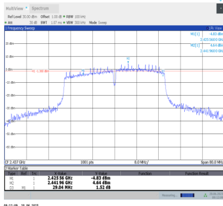
11n40SISO-Ant9-2437
