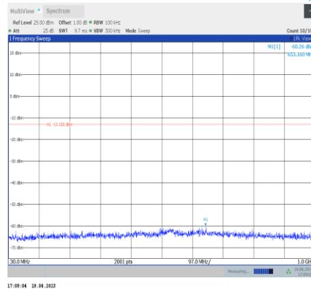
11g-Ant9-2437-30~1000
