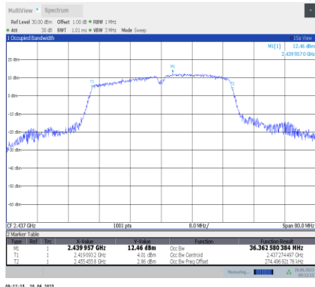
11n40SISO-Ant9-2437
