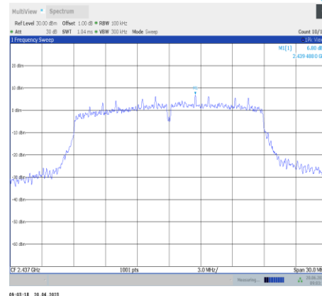
11n20SISO-Ant9-2437-0~Reference
