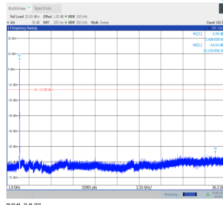
11n20SISO-Ant9-2437-1000~26500
