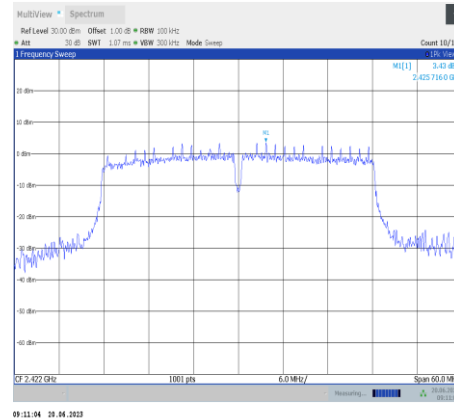
11n40SISO-Ant9-2422-0~Reference
