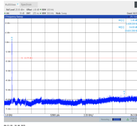
11n40SISO-Ant9-2422-1000~26500
