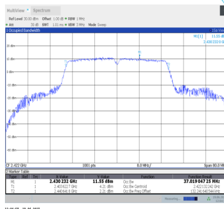
11n40SISO-Ant9-2422
