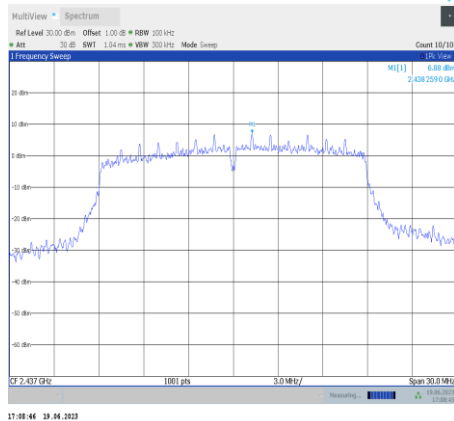
11g-Ant9-2437-0~Reference
