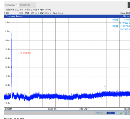
11n40SISO-Ant9-2452-1000~26500
