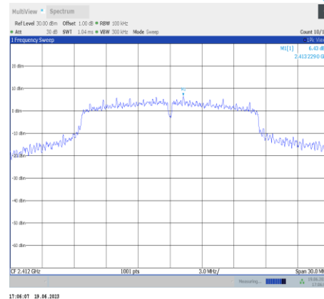
11g-Ant9-2412-0~Reference
