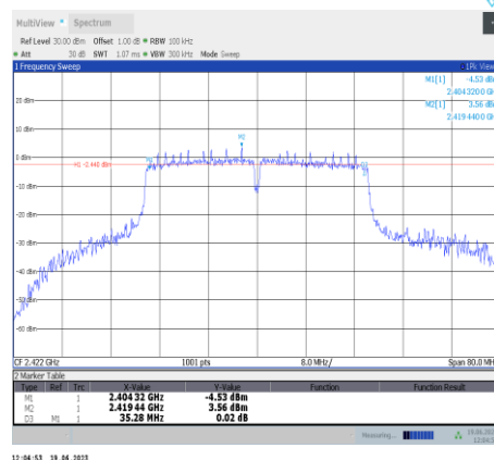
11n40SISO-Ant9-2422
