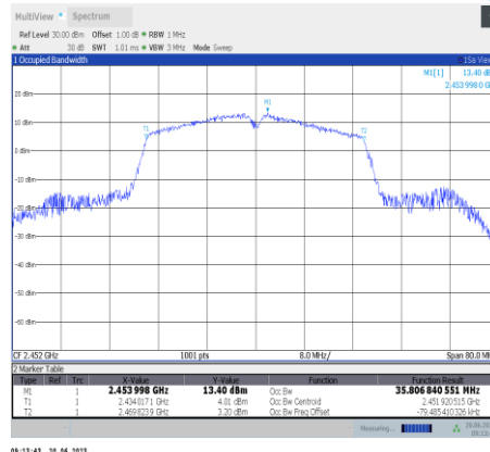
11n40SISO-Ant9-2452
