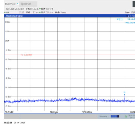
11n40SISO-Ant9-2437-30~1000
