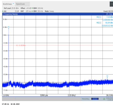
11g-Ant9-2437-1000~26500
