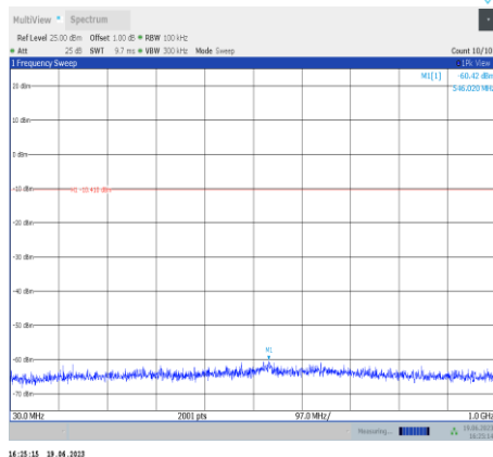
11b-Ant9-2437-30~1000
