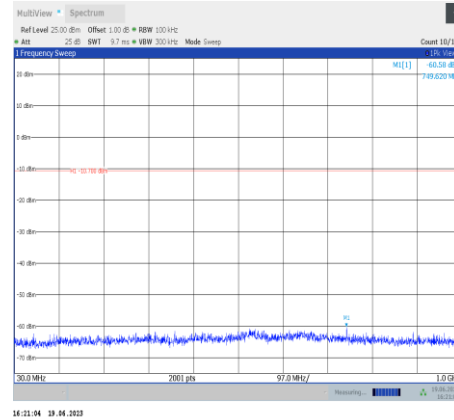
11b-Ant9-2412-30~1000
