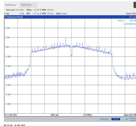
11n40SISO-Ant9-2452-0~Reference
