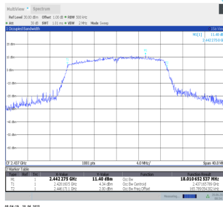
11n20SISO-Ant9-2437
