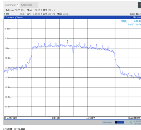
11g-Ant9-2462-0~Reference
