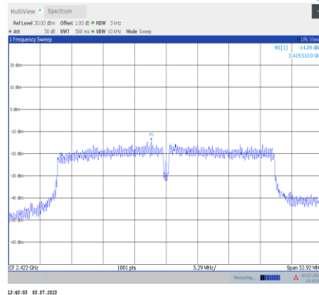
11n40SISO-Ant9-2422
