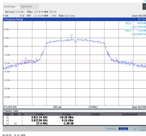
11a-Ant2-5825
