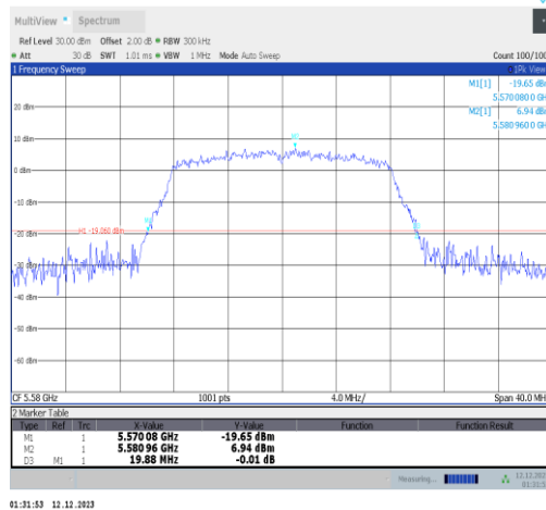
11a-Ant2-5580
