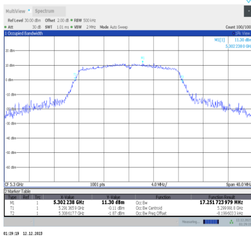
11a-Ant2-5300
