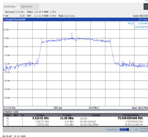
11ac80ISO-Ant2-5530
