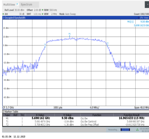
11a-Ant2-5700
