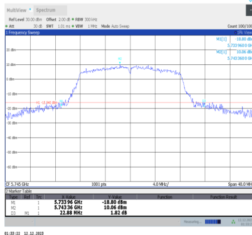
11a-Ant2-5745
