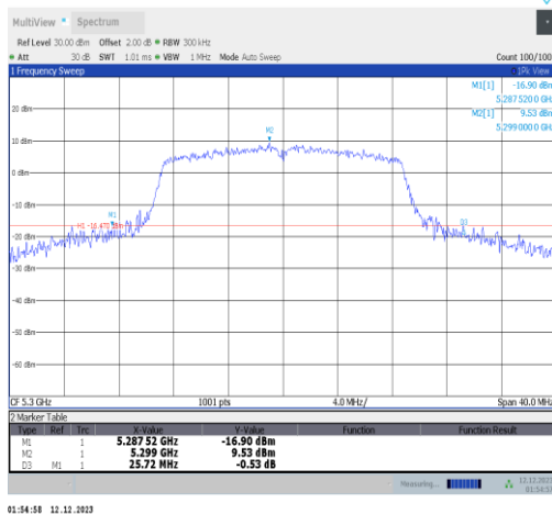
11n20SISO-Ant2-5300
