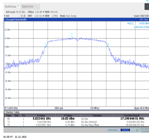
11a-Ant2-5825
