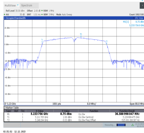
11n40SISO-Ant2-5230
