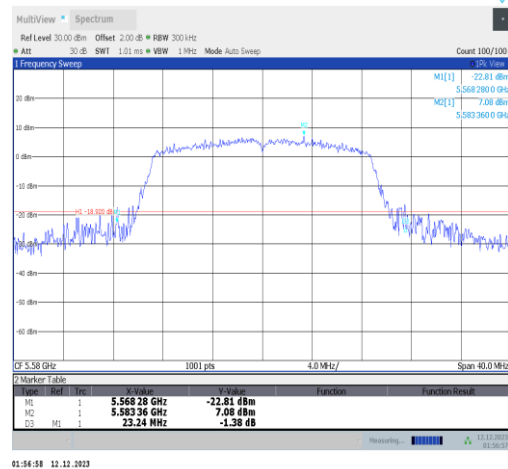
11n20SISO-Ant2-5580
