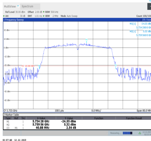
11n40SISO-Ant2-5755
