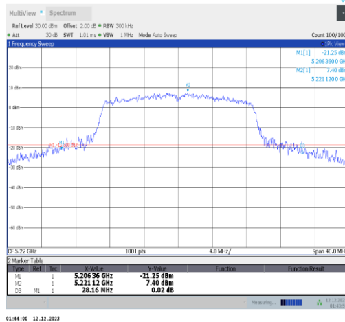
11n20SISO-Ant2-5220
