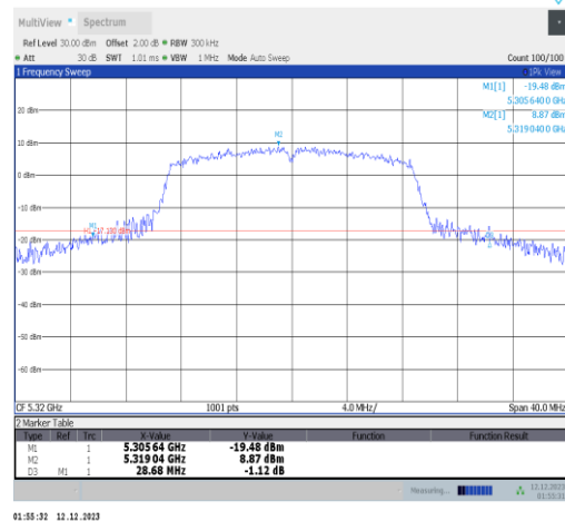
11n20SISO-Ant2-5320
