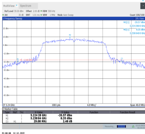
11n20SISO-Ant2-5240
