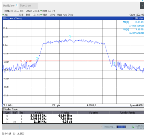
11n20SISO-Ant2-5500
