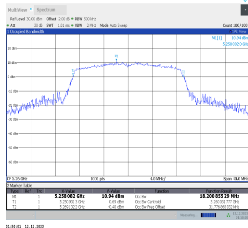
11n20SISO-Ant2-5260
