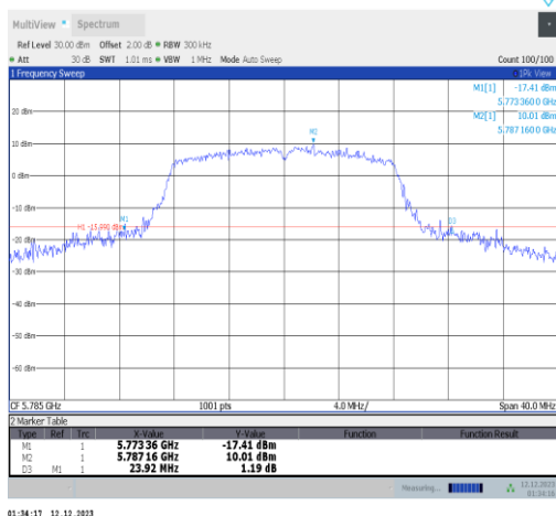
11a-Ant2-5785
