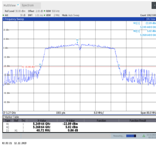
11n40SISO-Ant2-5270
