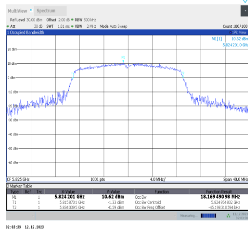
11n20SISO-Ant2-5825
