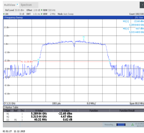
11n40SISO-Ant2-5310
