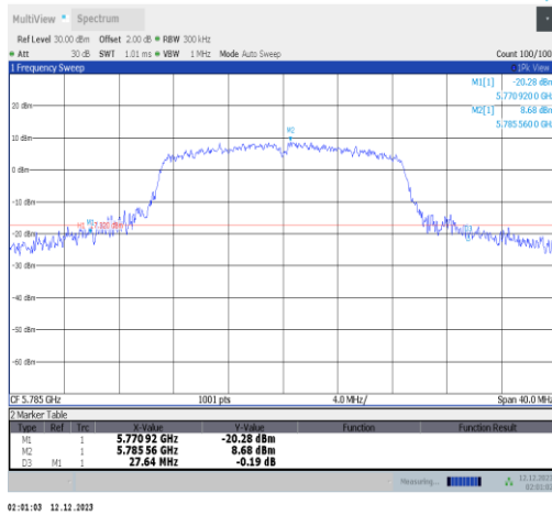
11n20SISO-Ant2-5785
