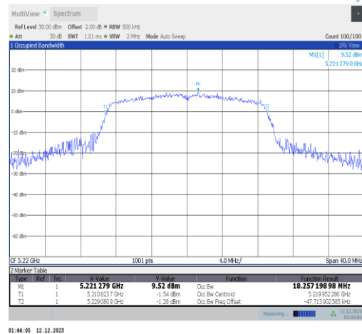
11n20SISO-Ant2-5220
