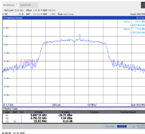
11n20SISO-Ant2-5700
