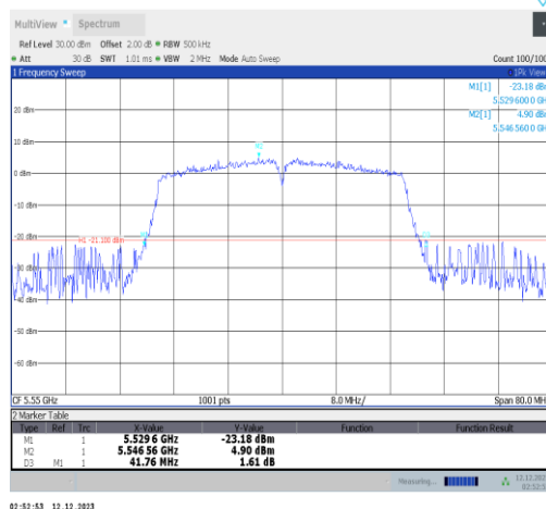
11n40SISO-Ant2-5550
