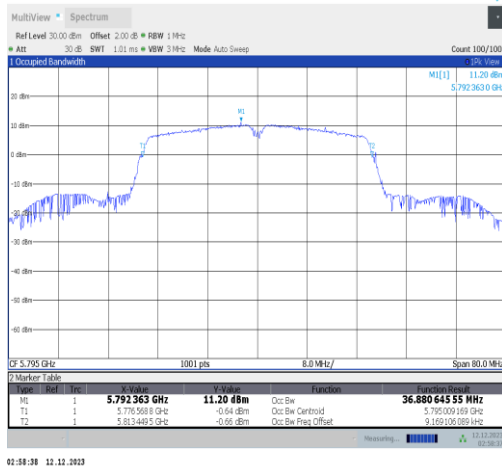
11n40SISO-Ant2-5795
