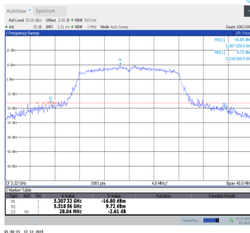
11a-Ant2-5320
