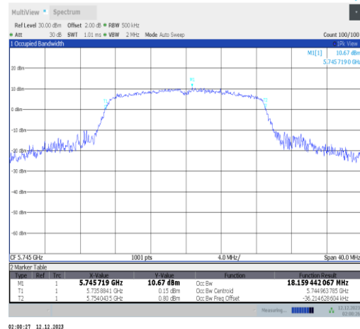
11n20SISO-Ant2-5745
