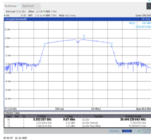
11n40SISO-Ant2-5550
