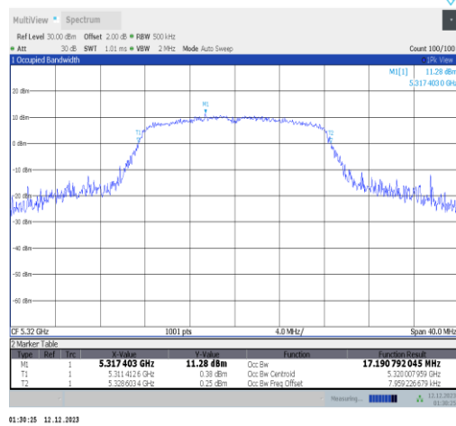
11a-Ant2-5320
