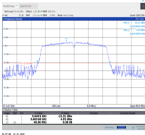
11n40SISO-Ant2-5670
