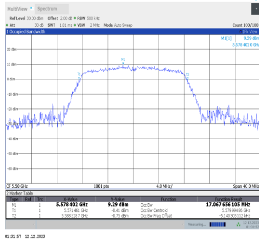
11a-Ant2-5580
