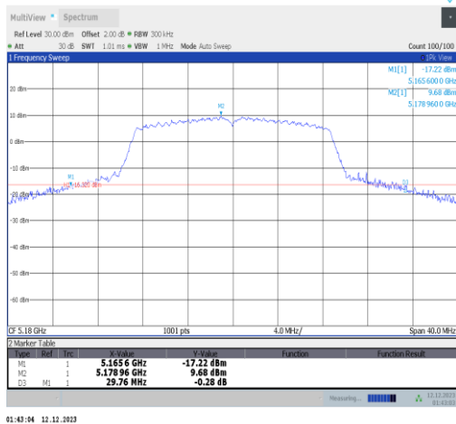
11n20SISO-Ant2-5180
