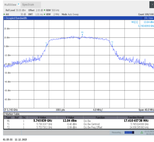
11a-Ant2-5745
