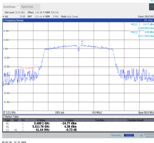
11n40SISO-Ant2-5510
