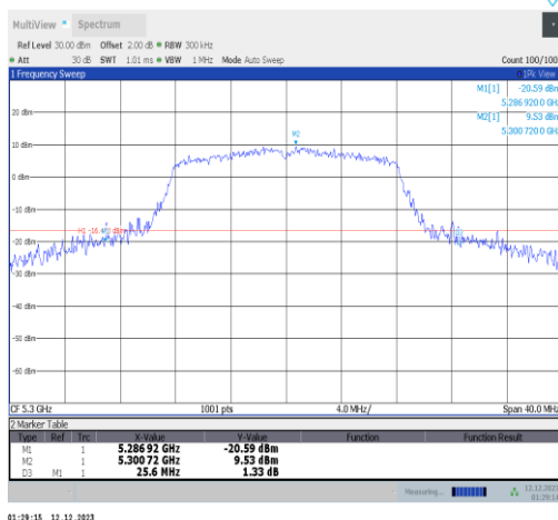
11a-Ant2-5300
