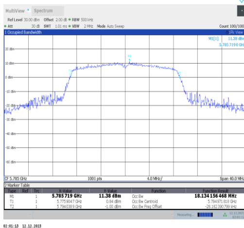
11n20SISO-Ant2-5785
