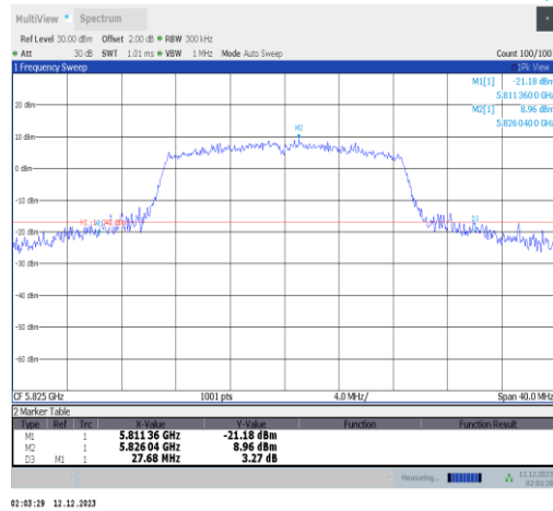
11n20SISO-Ant2-5825
