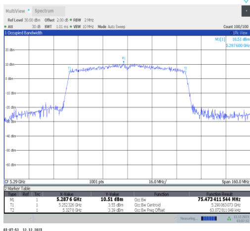
11ac80ISO-Ant2-5290
