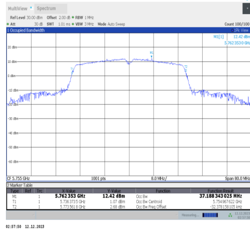
11n40SISO-Ant2-5755
