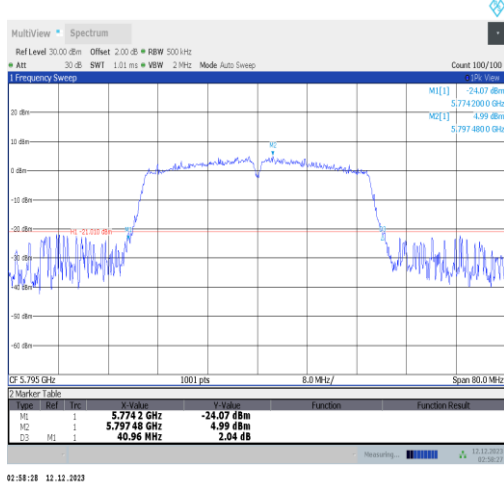
11n40SISO-Ant2-5795
