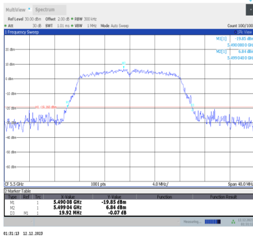
11a-Ant2-5500
