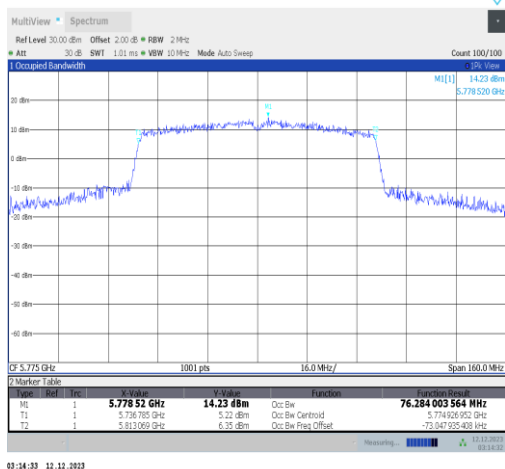
11ac80ISO-Ant2-5775
