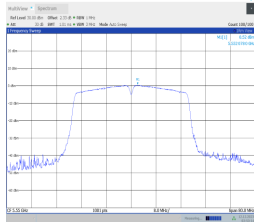
11n40ISO-Ant2-5550-PASS
