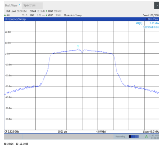
11a-Ant2-5825-PASS
