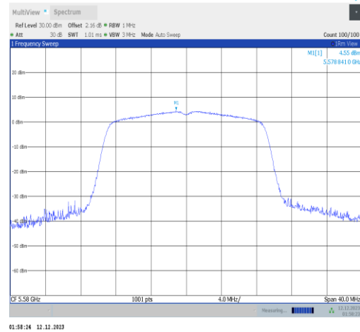
11n20ISO-Ant2-5580-PASS
