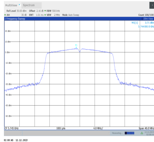
11n20ISO-Ant2-5745-PASS
