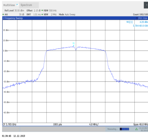
11a-Ant2-5785-PASS
