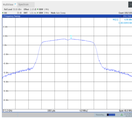
11a-Ant2-5300-PASS
