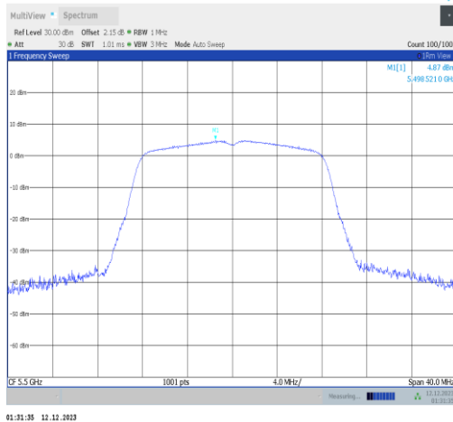
11a-Ant2-5500-PASS
