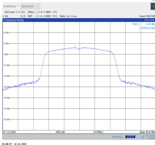
11n20ISO-Ant2-5240-PASS
