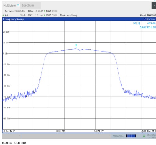
11n20ISO-Ant2-5700-PASS
