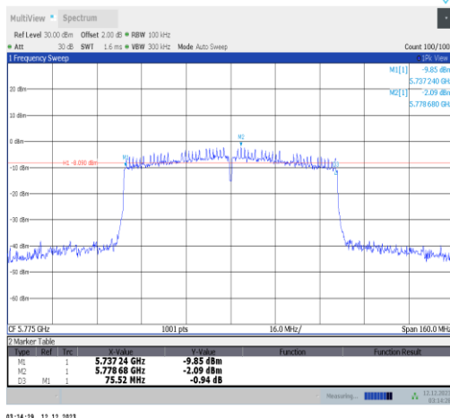
11ac80ISO-Ant2-5775-PASS
