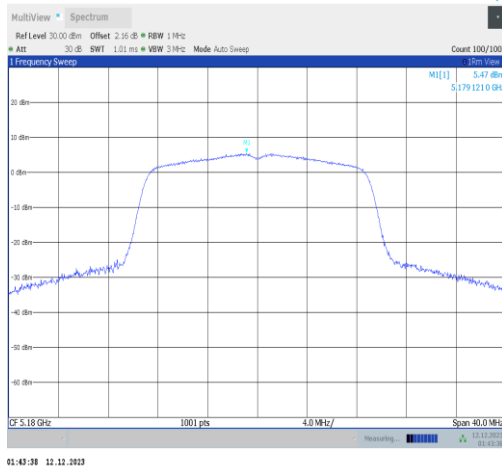
11n20ISO-Ant2-5180-PASS
