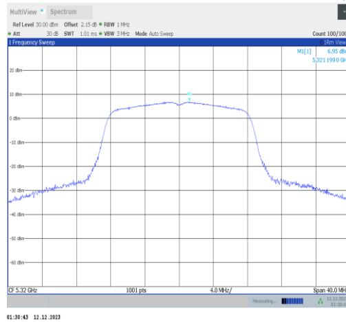
11a-Ant2-5320-PASS
