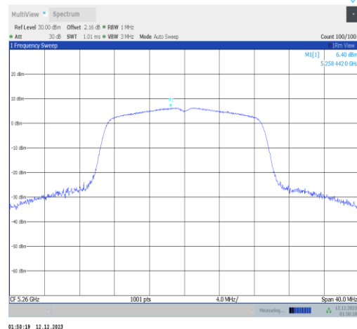
11n20ISO-Ant2-5260-PASS
