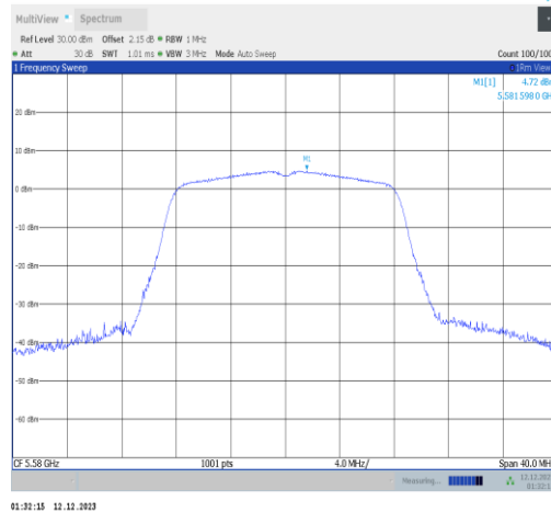
11a-Ant2-5580-PASS
