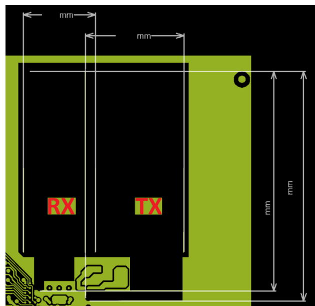
Antenna Dimension
