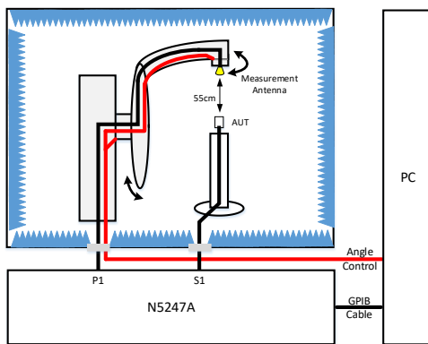
Test Setup
