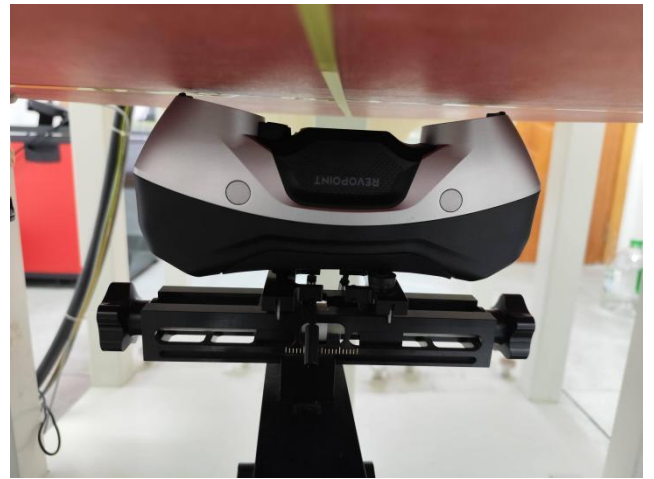
Body Back(5mm)
