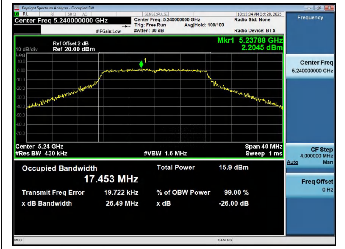
11A-Ant2-5240
