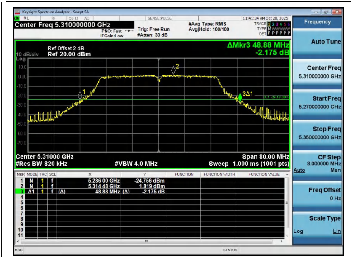
11AC40MIMO-Ant1-5310
