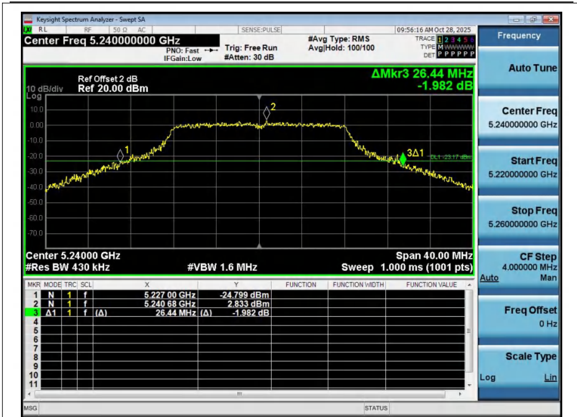
11A-Ant1-5240
