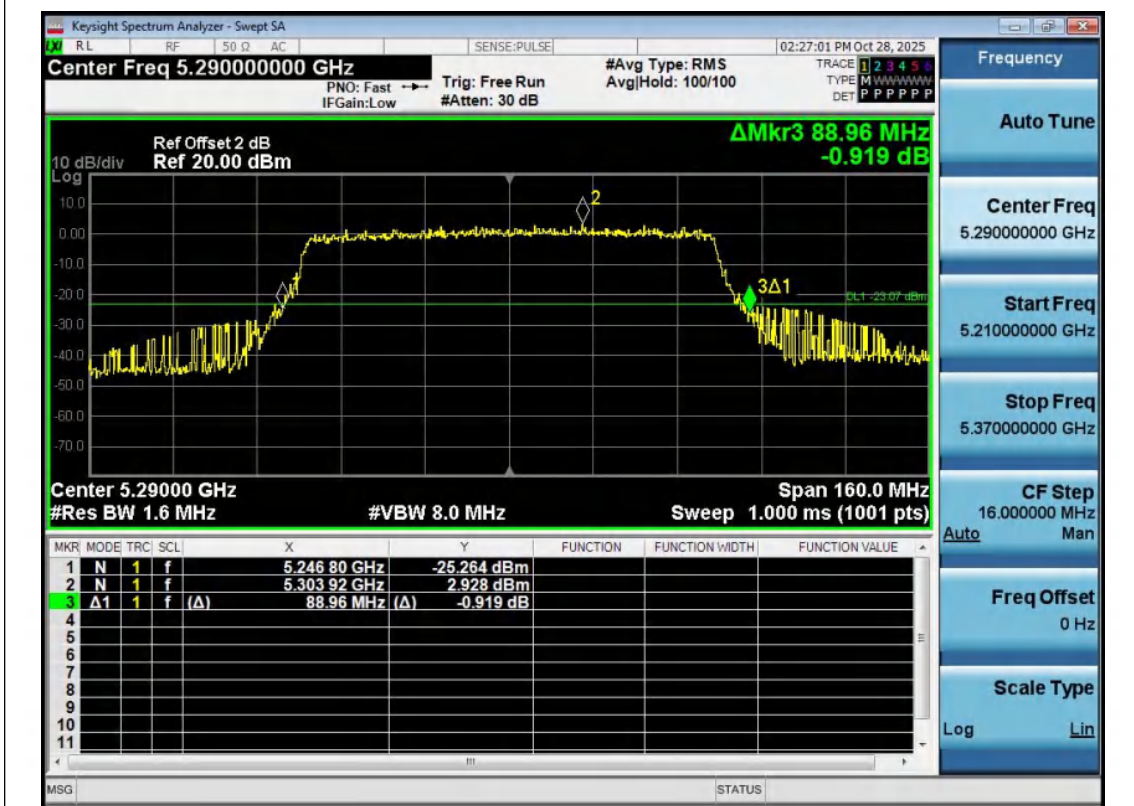
11AX80MIMO-Ant2-5290
