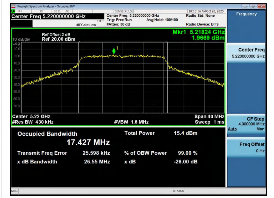
11A-Ant2-5220
