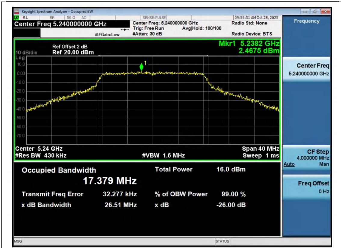
11A-Ant1-5240
