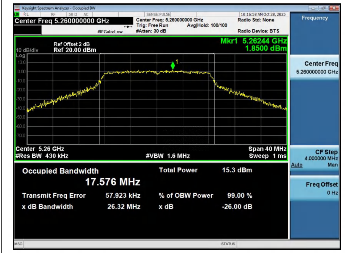
11A-Ant2-5260
