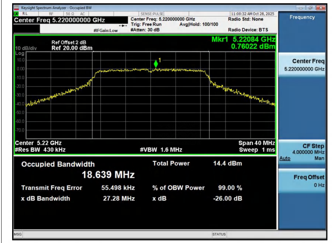
11AC20MIMO-Ant2-5220
