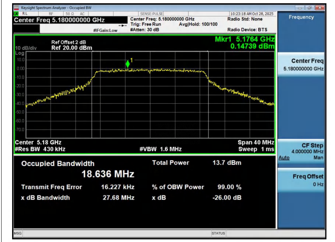
11N20MIMO-Ant2-5180
