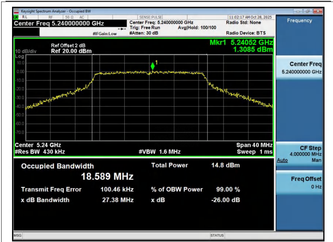
11AC20MIMO-Ant1-5240
