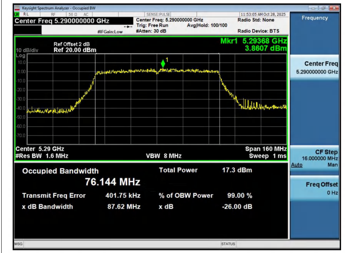
11AC80MIMO-Ant2-5290
