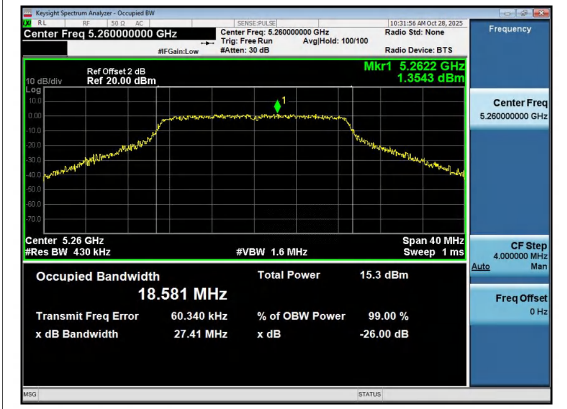
11N20MIMO-Ant2-5260
