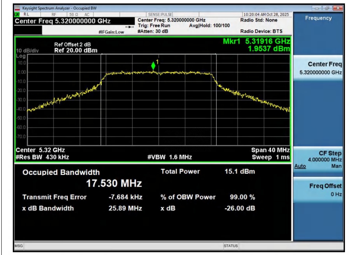
11A-Ant2-5320
