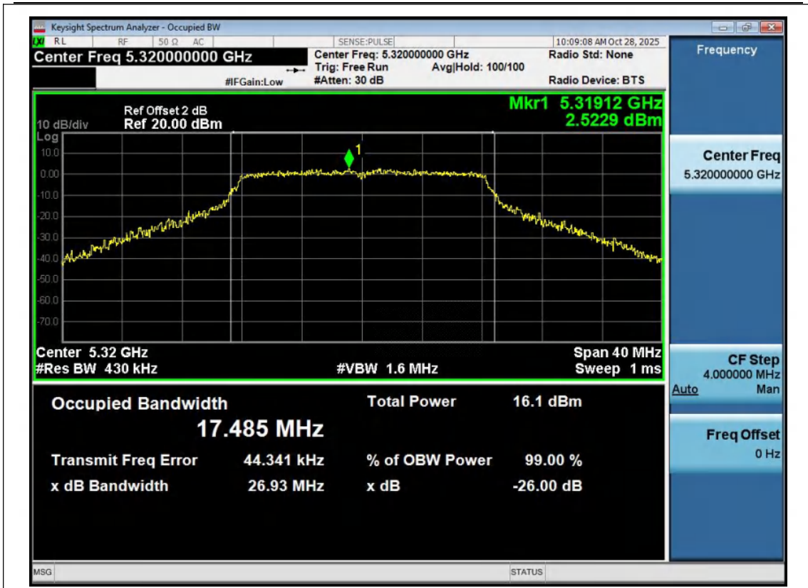
11A-Ant1-5320
