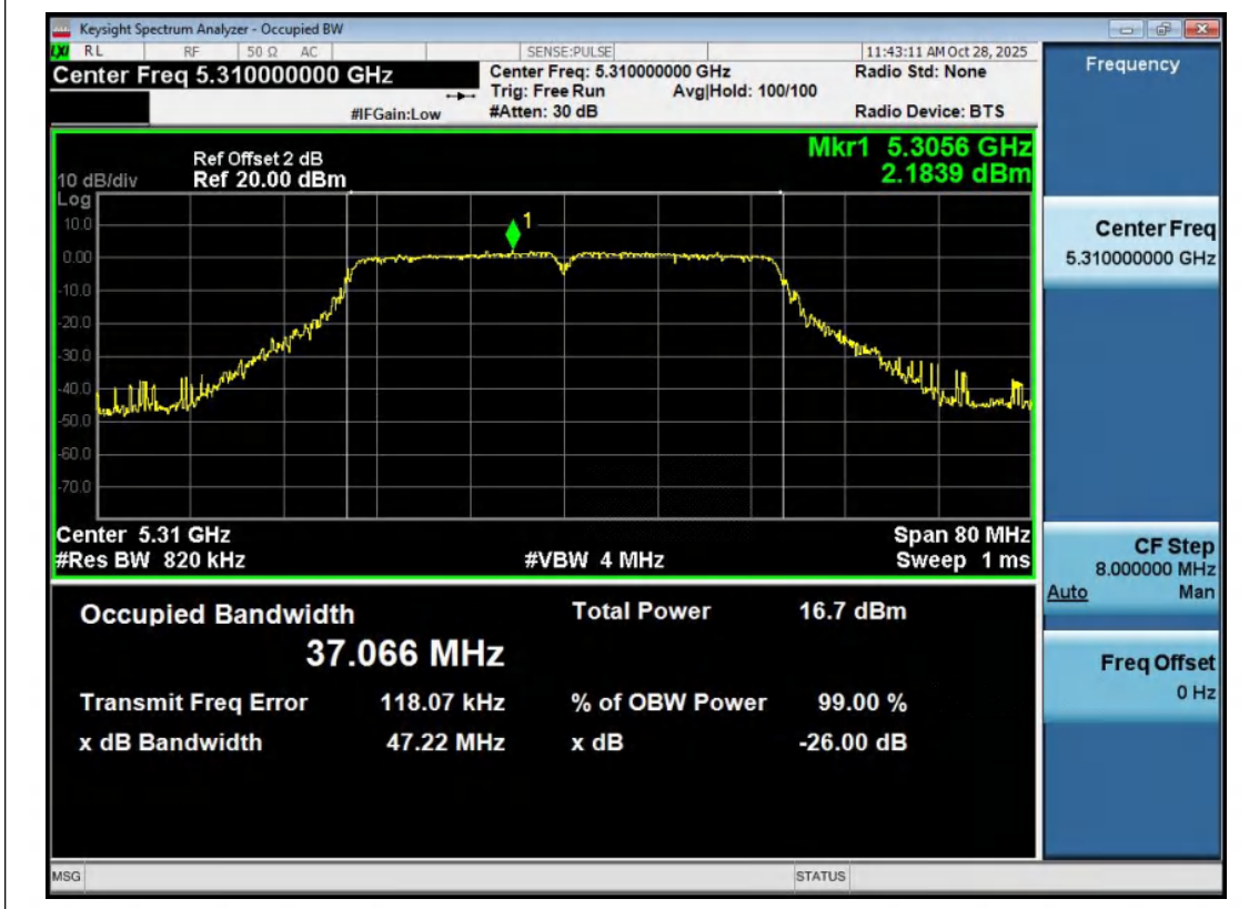
11AC40MIMO-Ant2-5310
