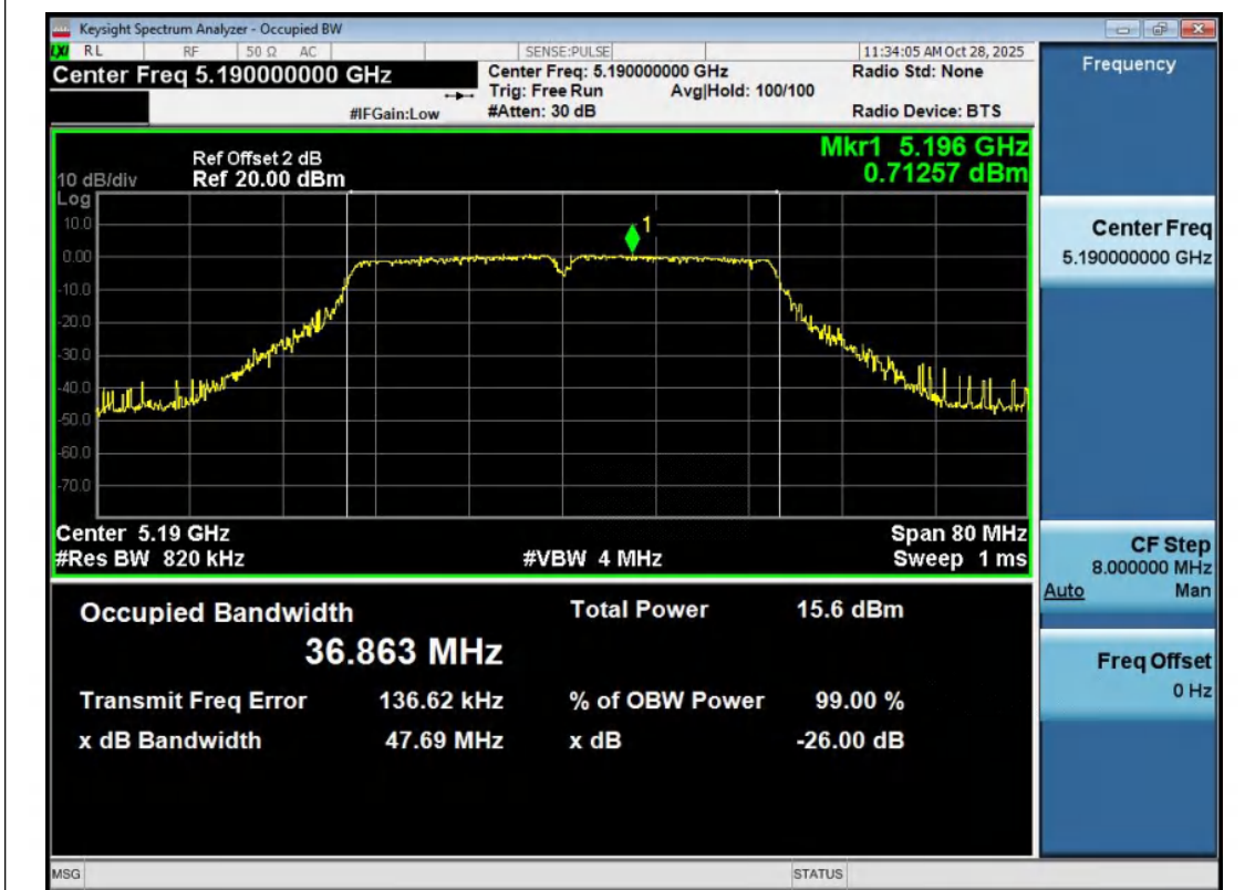
11AC40MIMO-Ant2-5190
