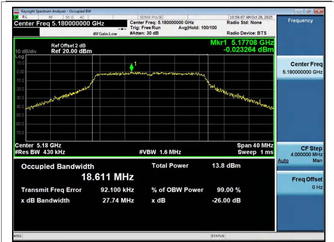
11AC20MIMO-Ant1-5180
