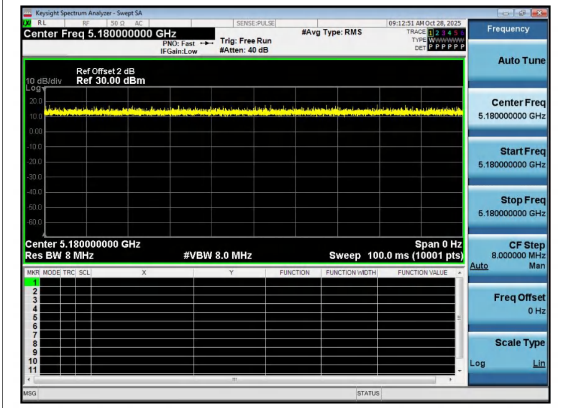
NTNV-11N20MIMO-Ant2-5180
