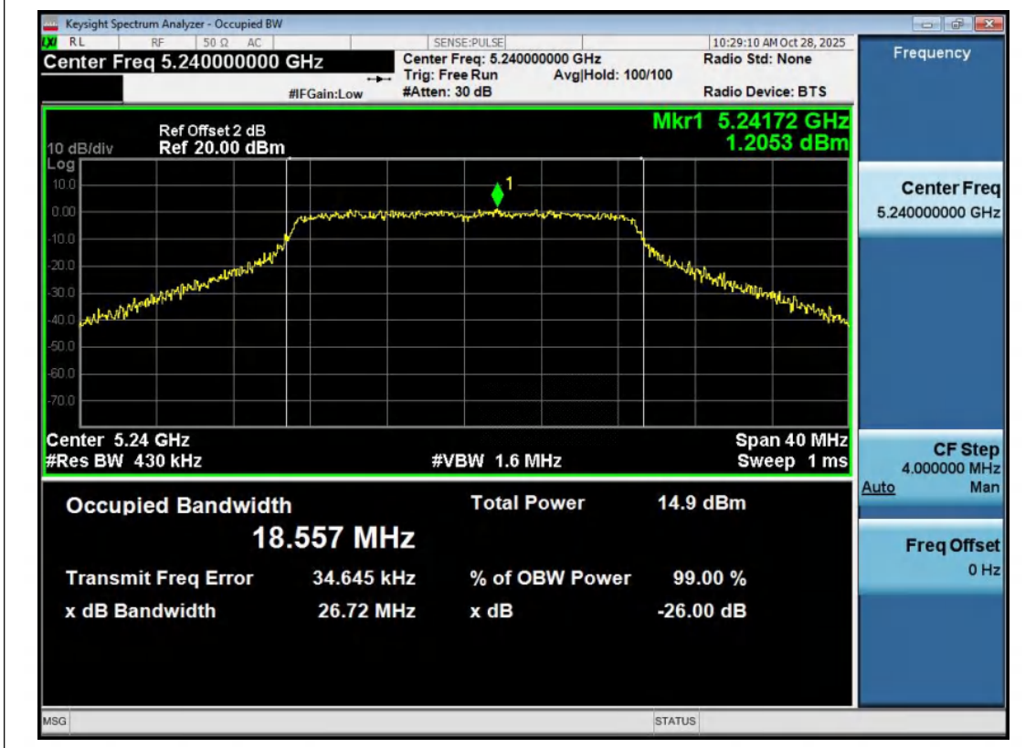
11N20MIMO-Ant2-5240
