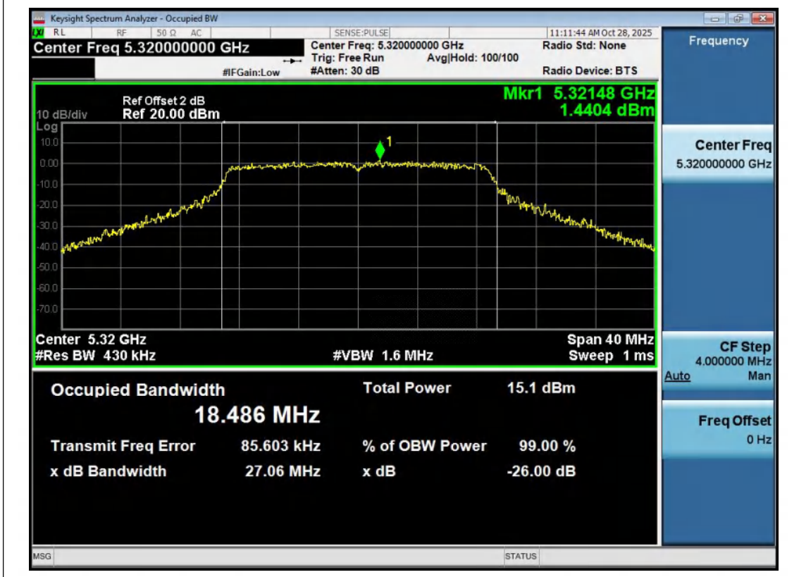
11AC20MIMO-Ant2-5320
