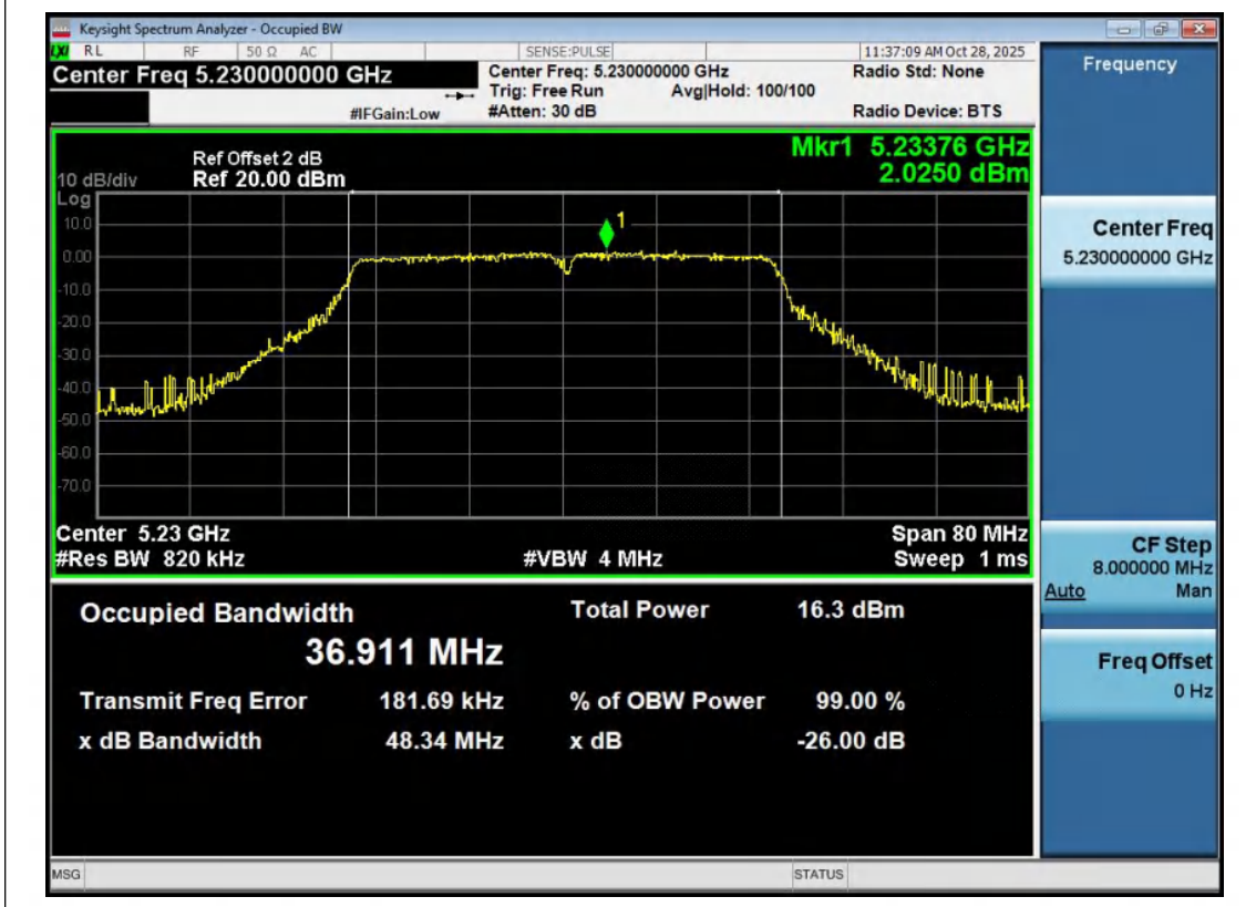
11AC40MIMO-Ant2-5230
