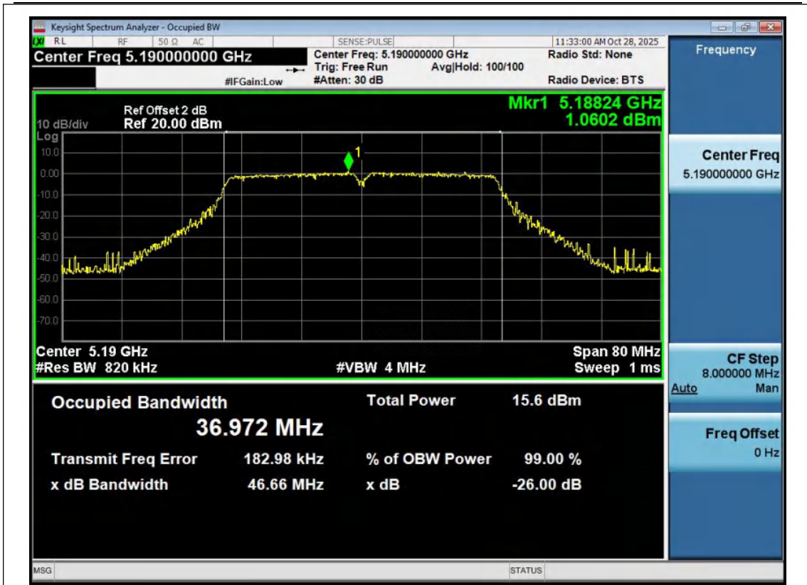
11AC40MIMO-Ant1-5190
