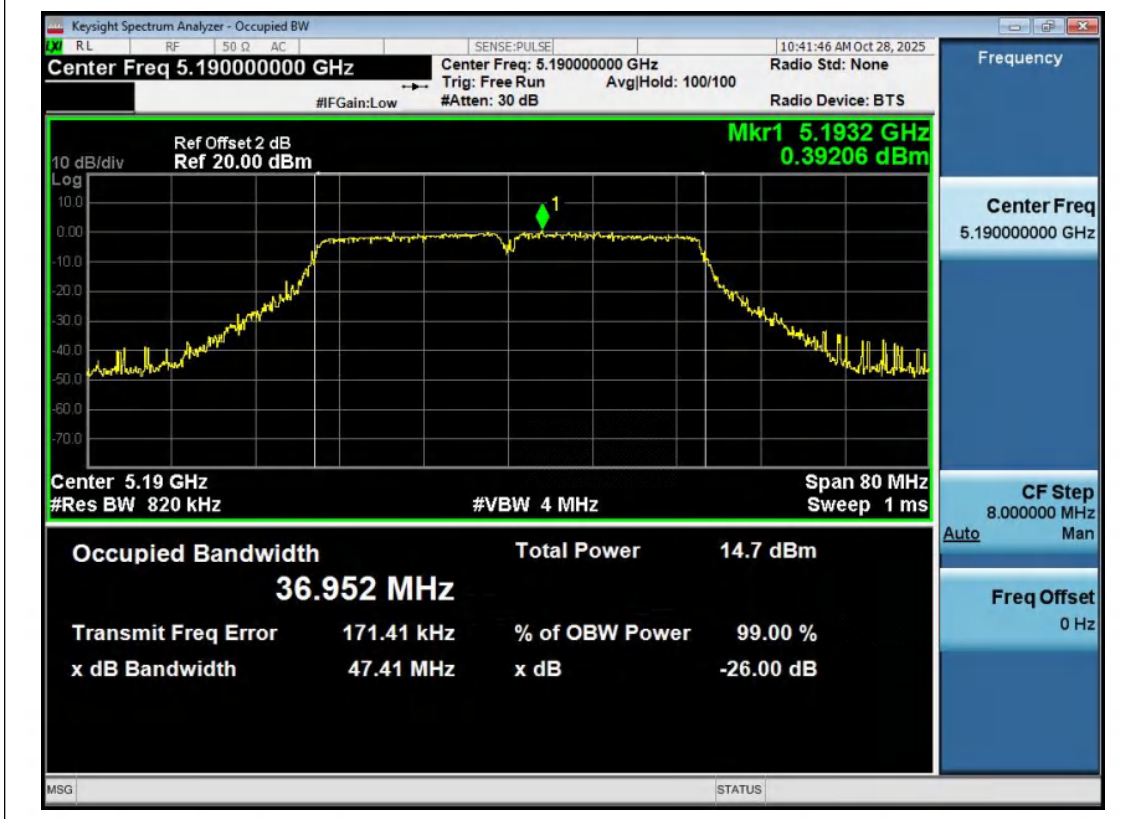
11N40MIMO-Ant2-5190
