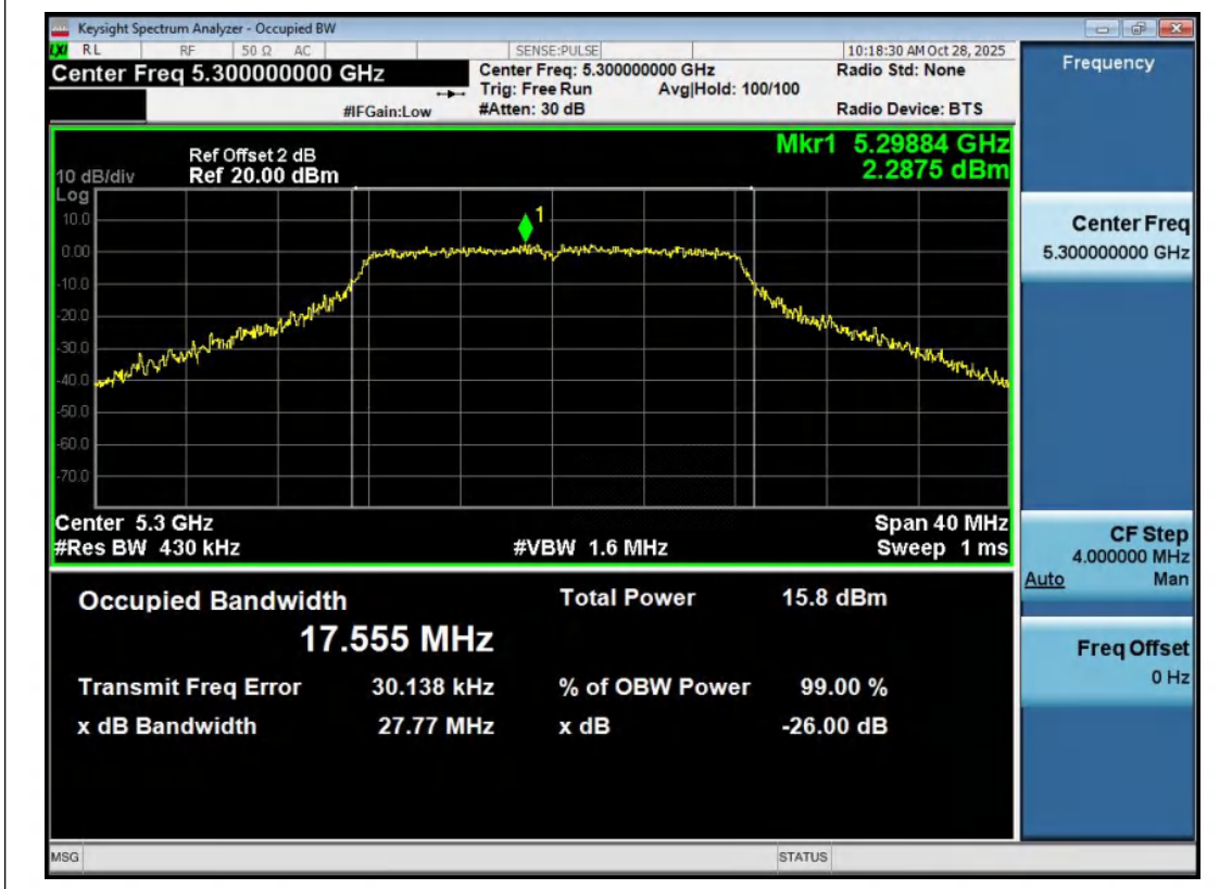
11A-Ant2-5300
