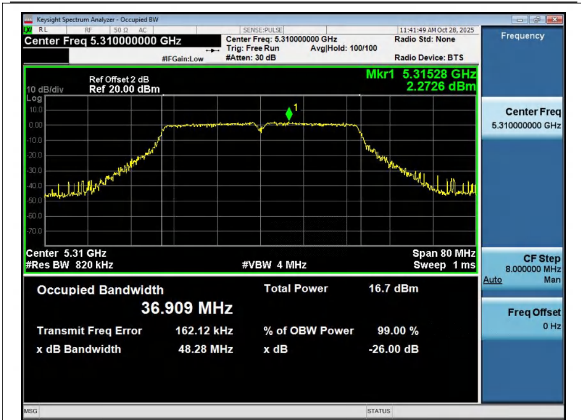
11AC40MIMO-Ant1-5310
