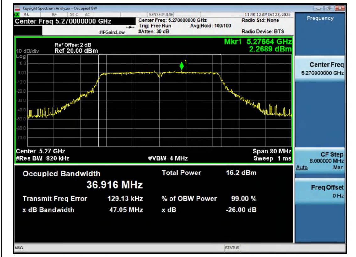
11AC40MIMO-Ant2-5270
