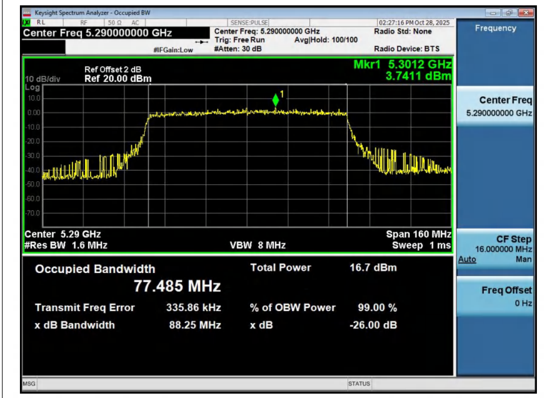
11AX80MIMO-Ant2-5290
