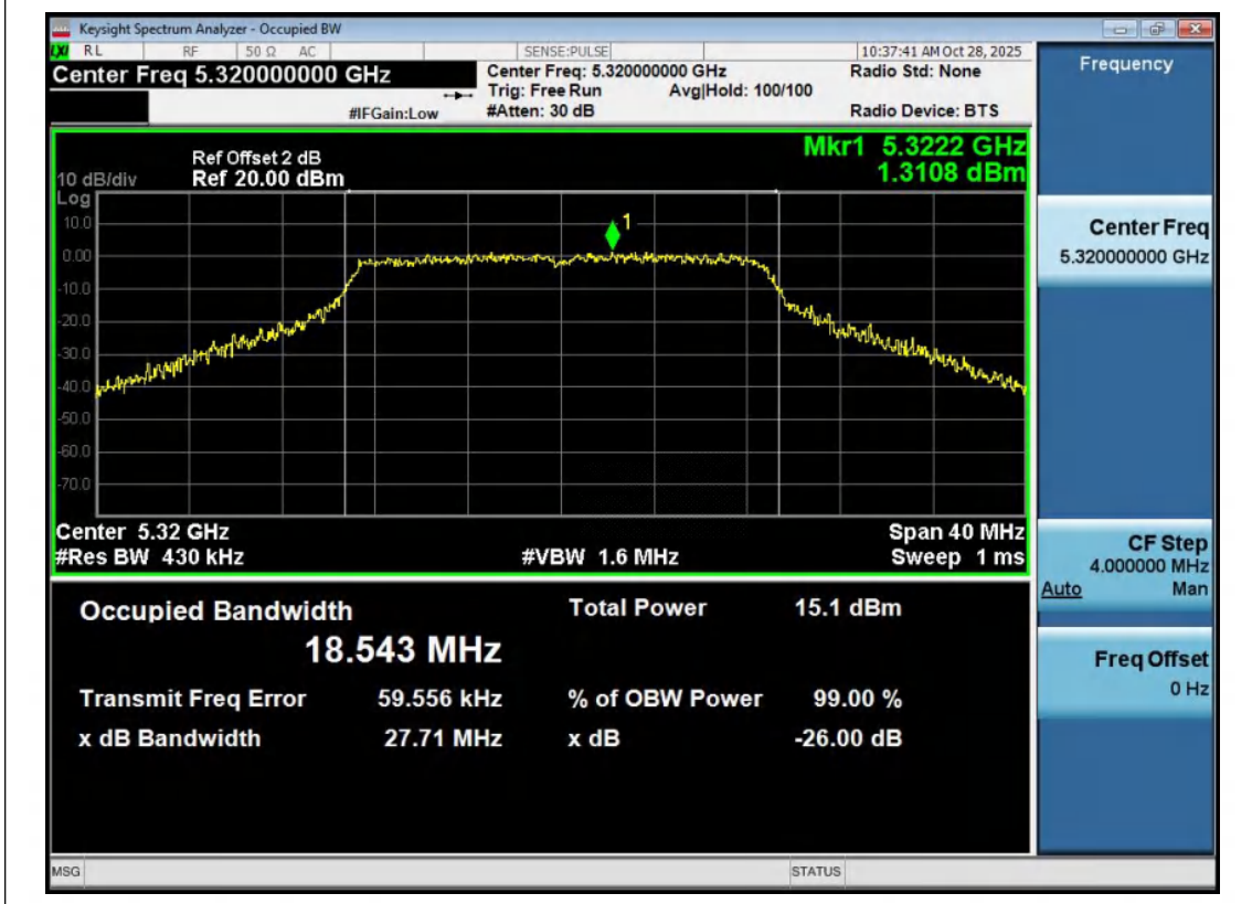
11N20MIMO-Ant2-5320
