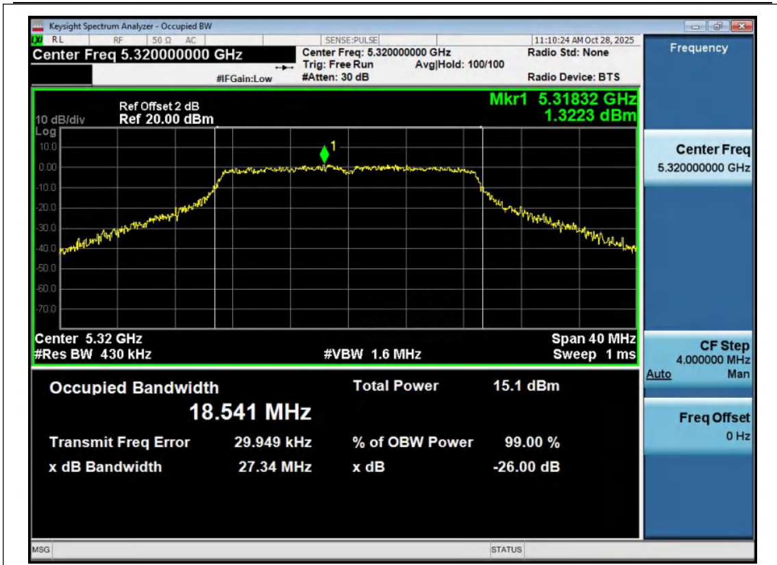
11AC20MIMO-Ant1-5320
