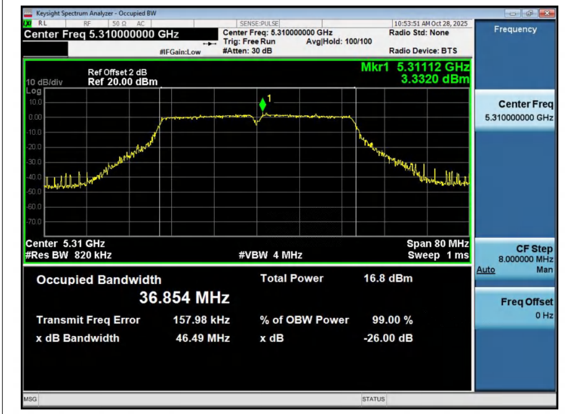
11N40MIMO-Ant2-5310
