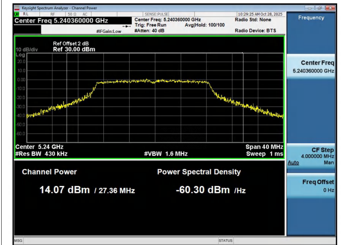
11N20MIMO-Ant2-5240-PASS
