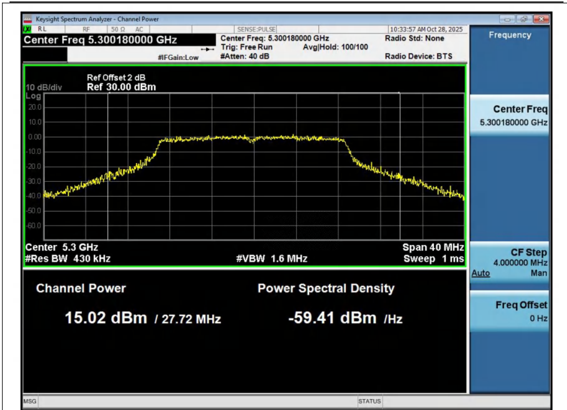
11N20MIMO-Ant1-5300-PASS
