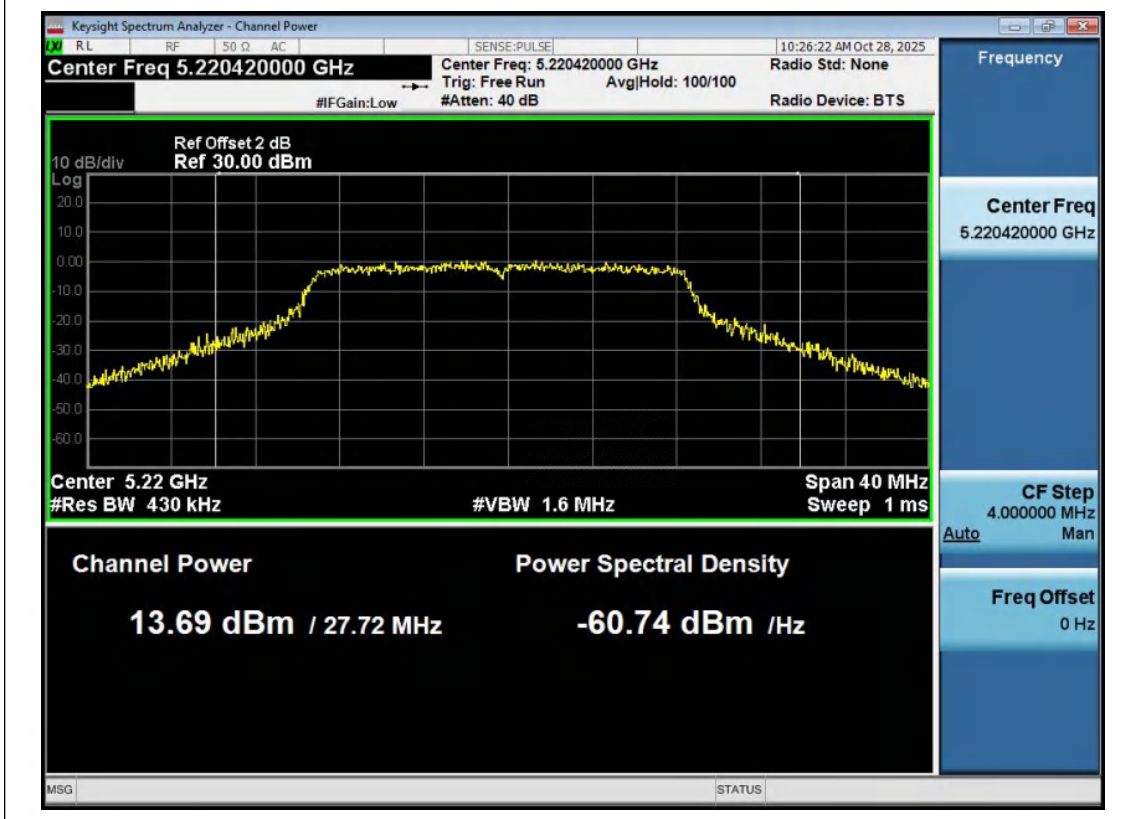
11N20MIMO-Ant2-5220-PASS
