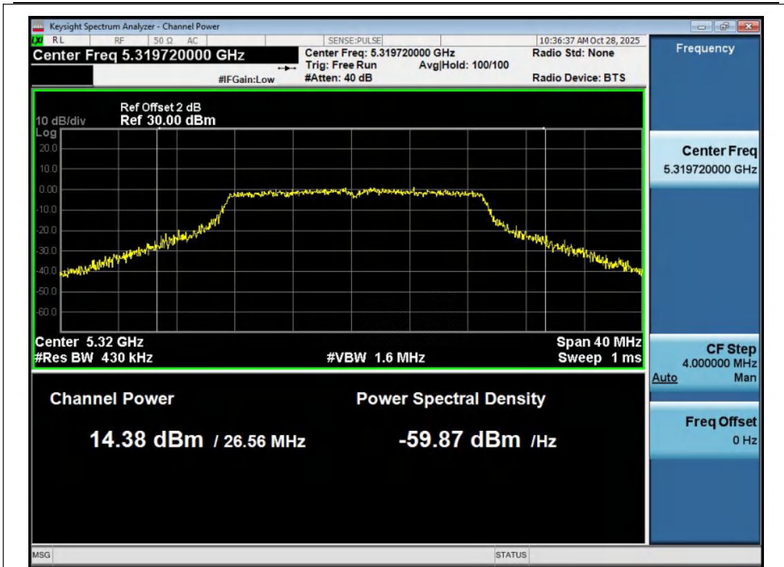
11N20MIMO-Ant1-5320-PASS
