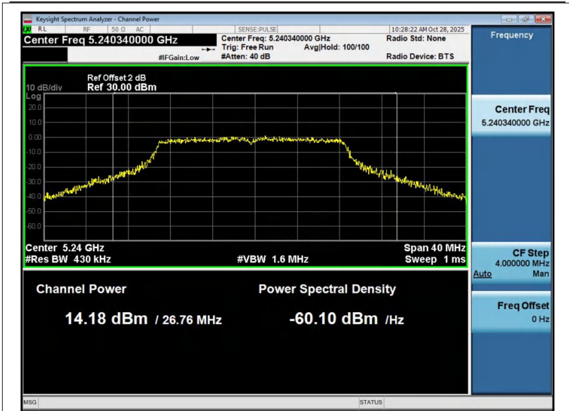
11N20MIMO-Ant1-5240-PASS
