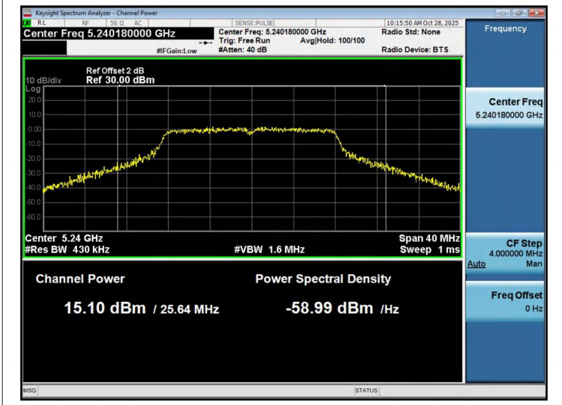
11A-Ant2-5240-PASS
