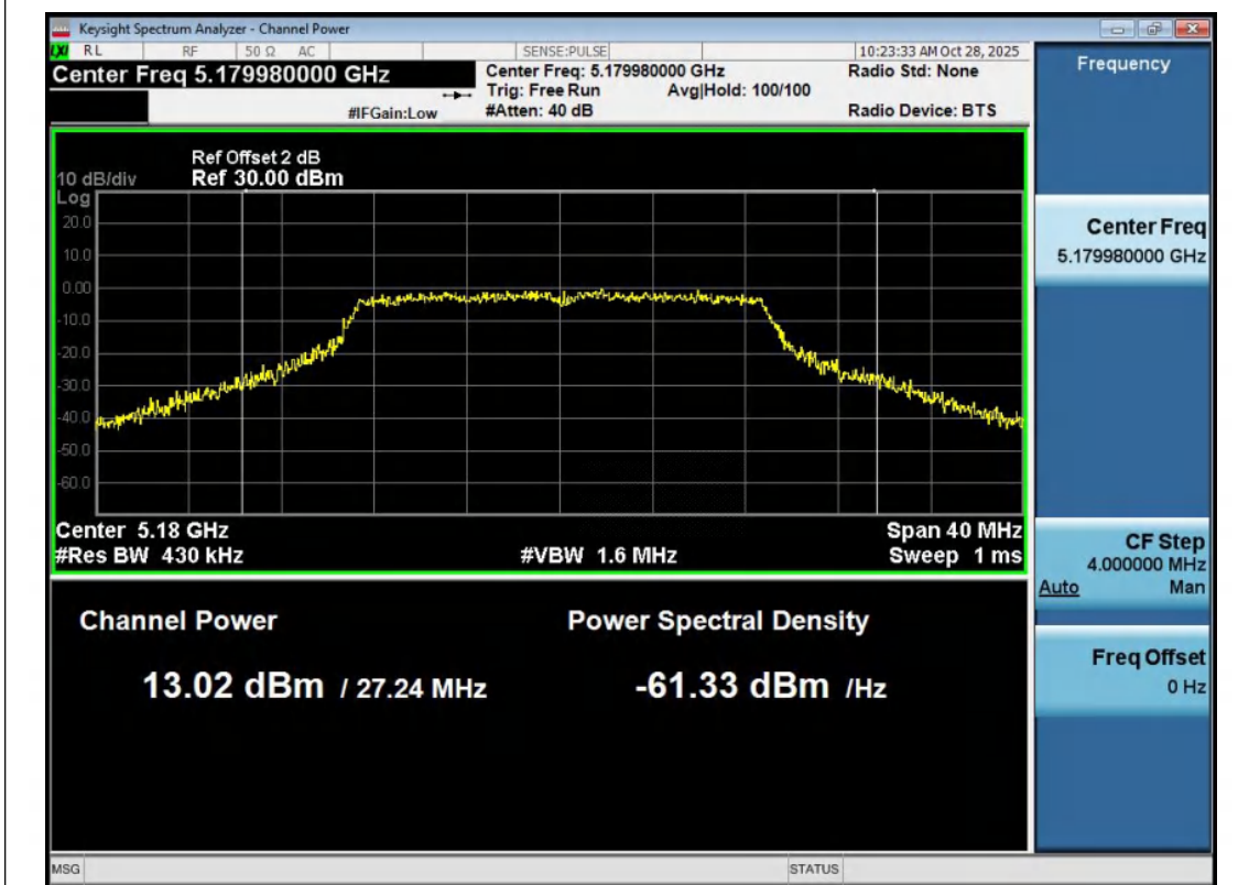
11N20MIMO-Ant2-5180-PASS
