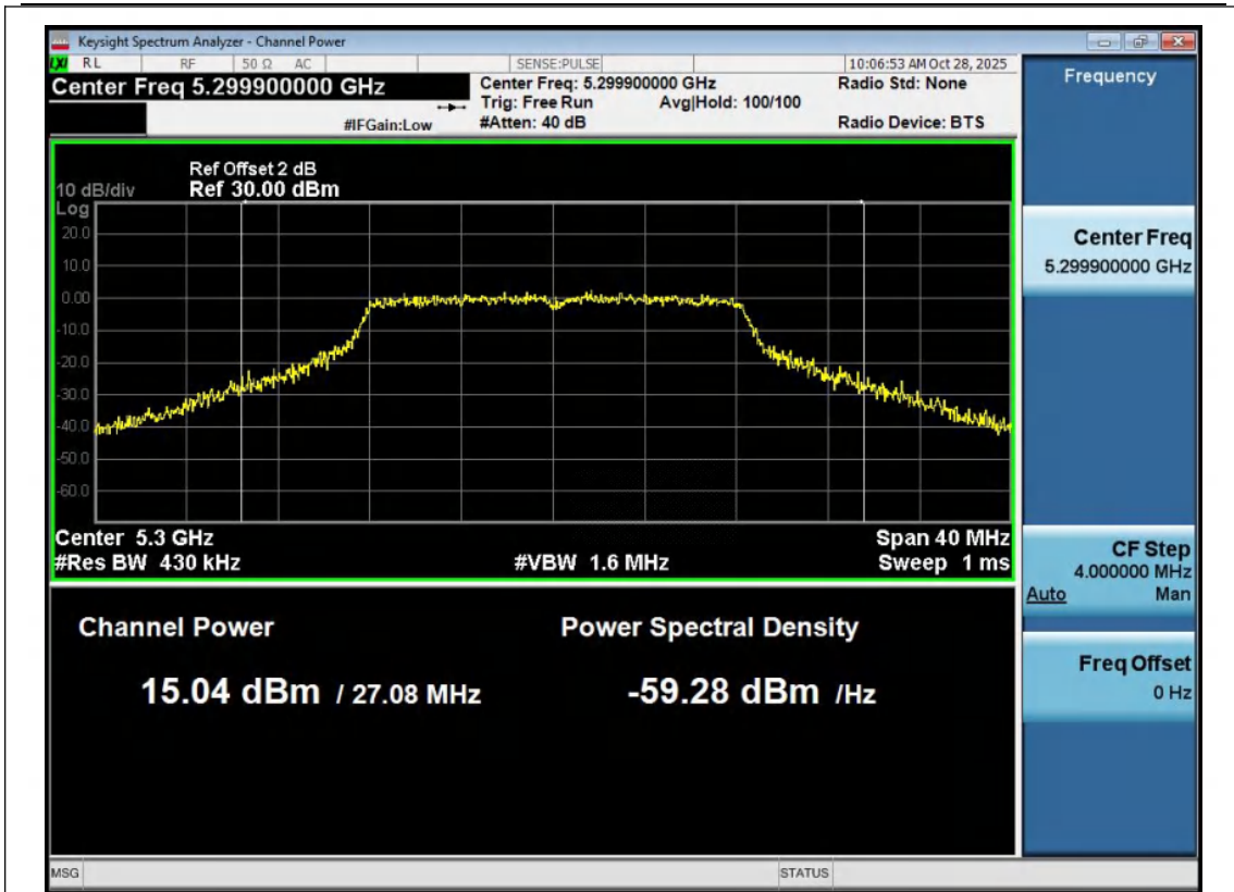
11A-Ant1-5300-PASS
