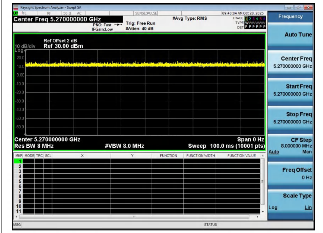
NTNV-11AX40MIMO-Ant2-5270
