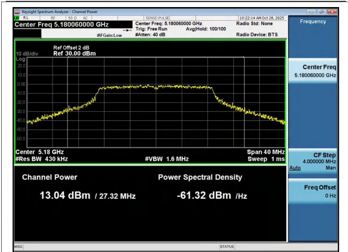
11N20MIMO-Ant1-5180-PASS
