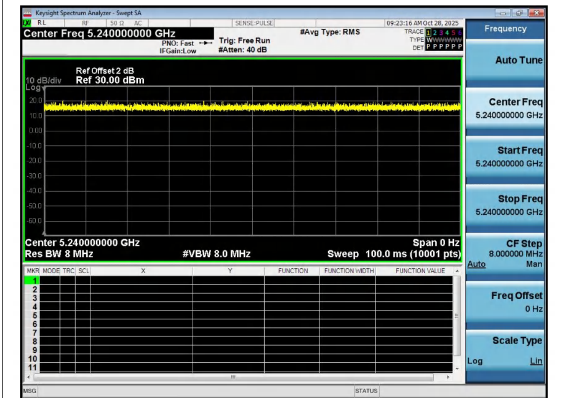
NTNV-11AC20MIMO-Ant2-5240
