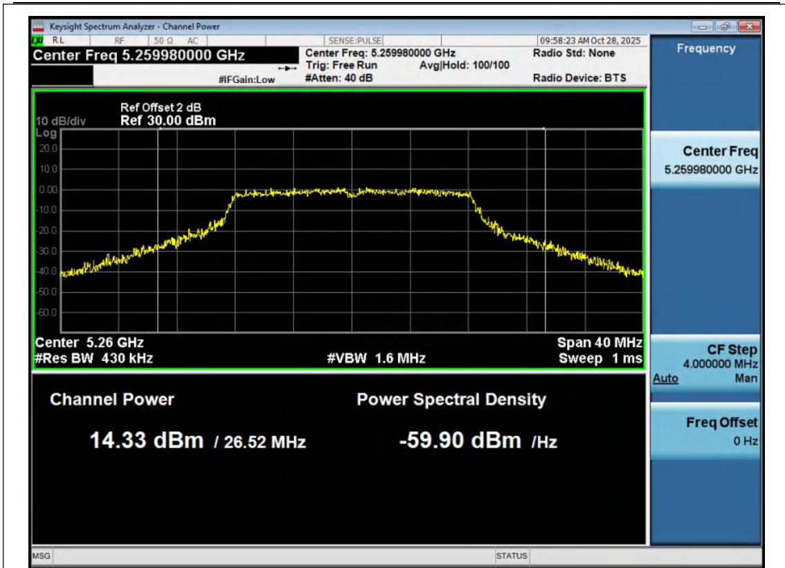
11A-Ant1-5260-PASS
