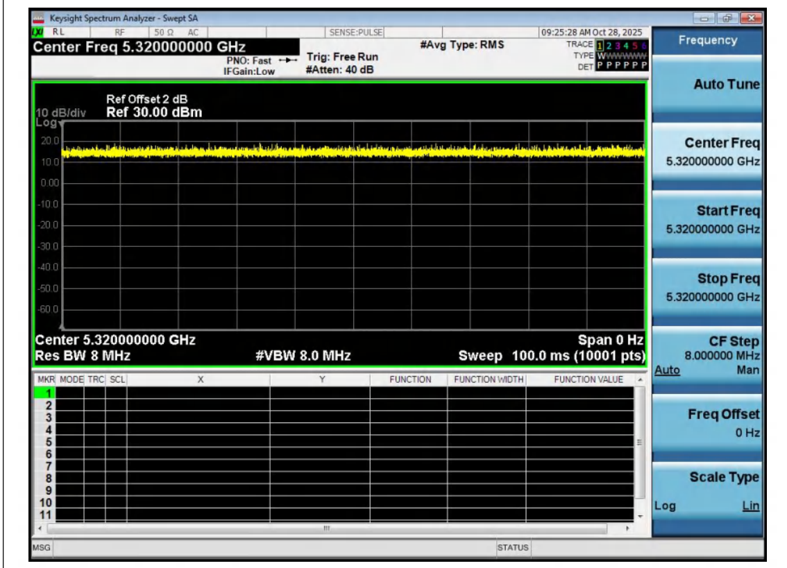
NTNV-11AC20MIMO-Ant2-5320
