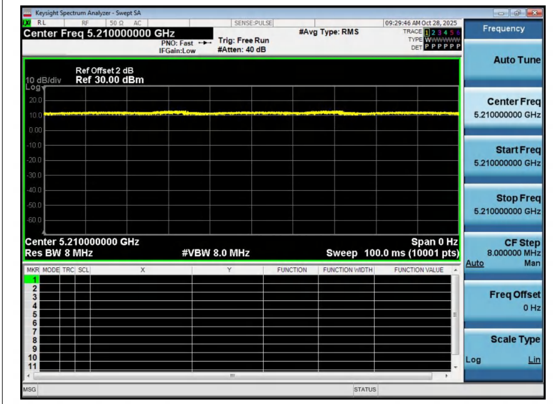
NTNV-11AC80MIMO-Ant2-5210
