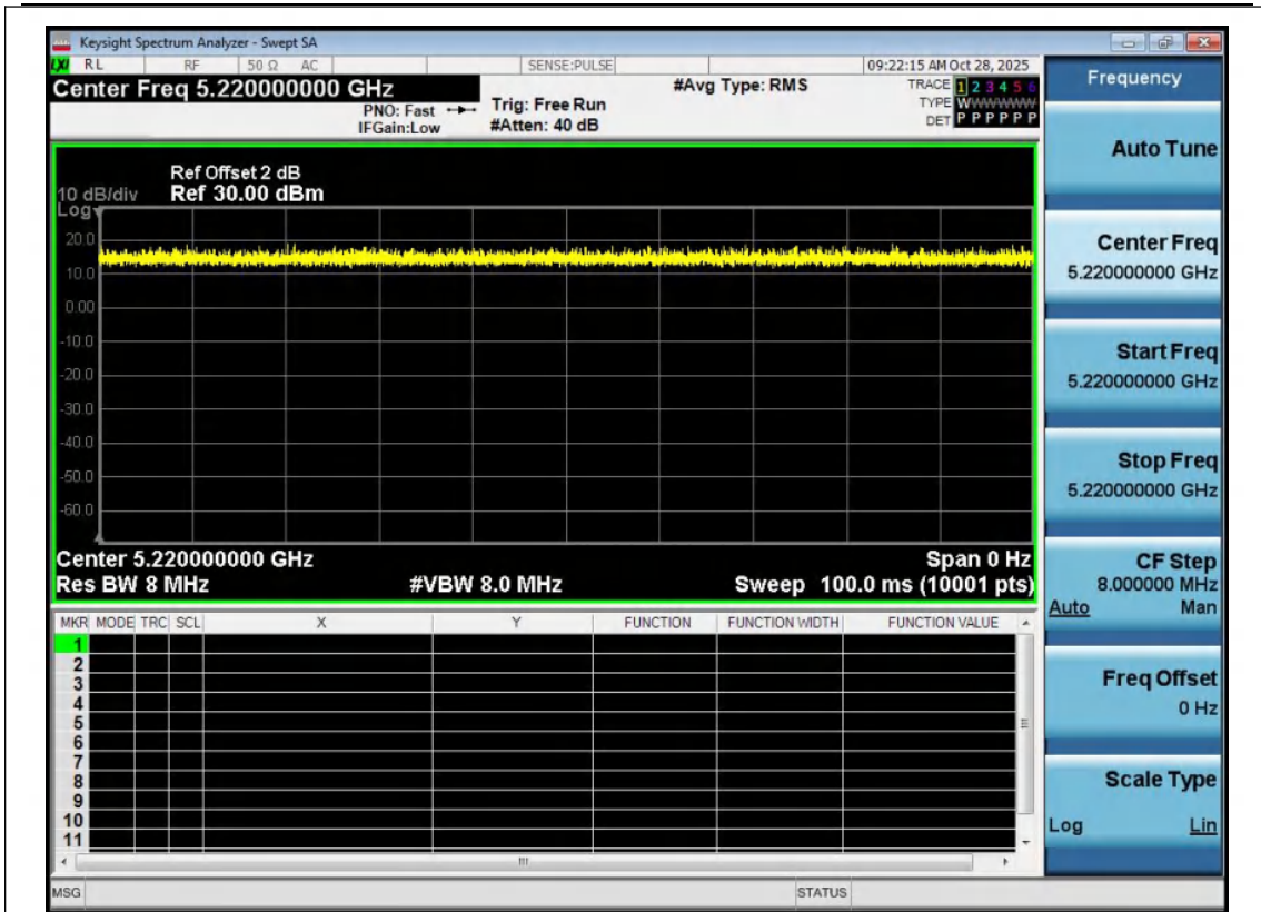
NTNV-11AC20MIMO-Ant1-5220
