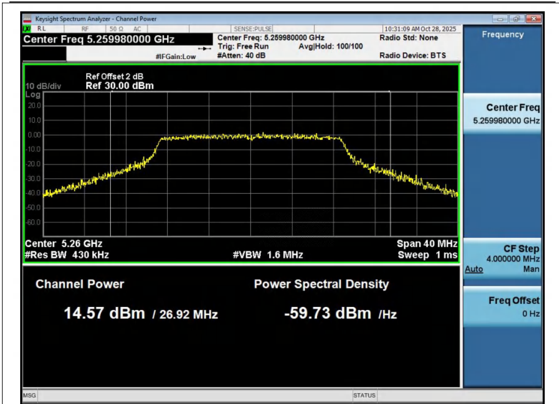
11N20MIMO-Ant1-5260-PASS
