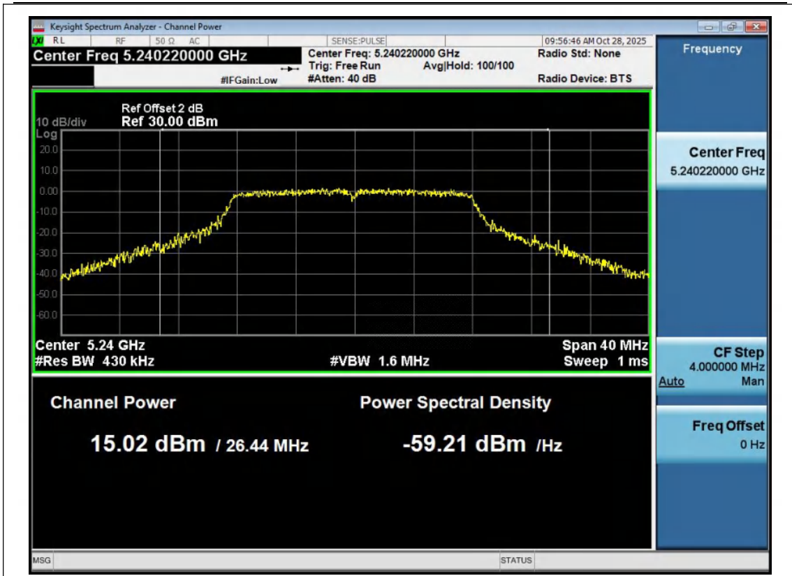
11A-Ant1-5240-PASS
