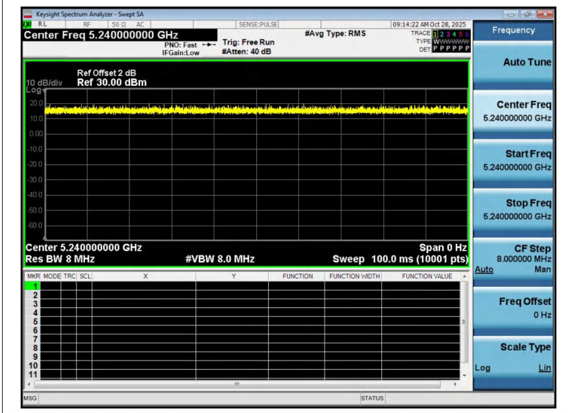
NTNV-11N20MIMO-Ant2-5240
