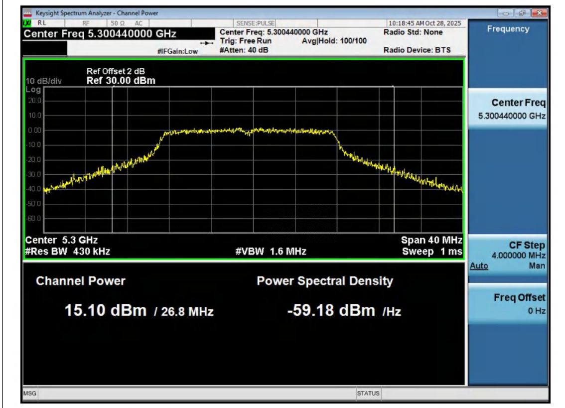
11A-Ant2-5300-PASS
