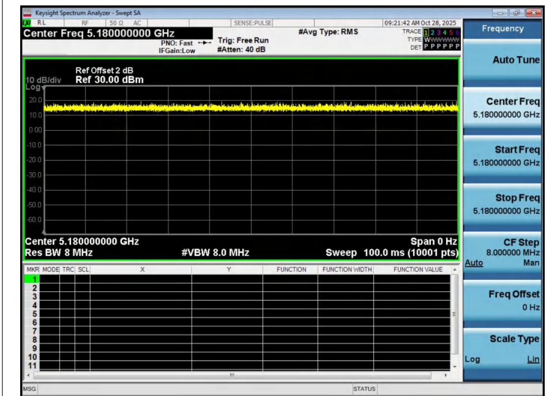
NTNV-11AC20MIMO-Ant2-5180
