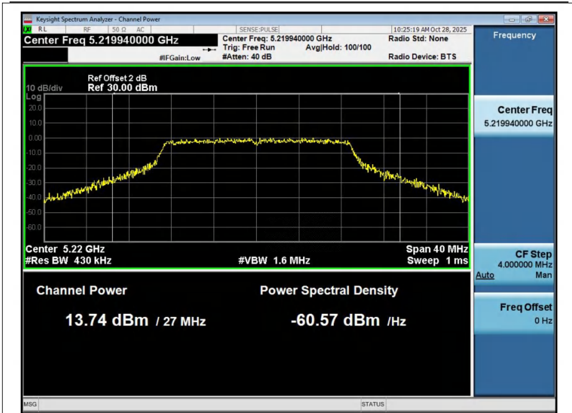
11N20MIMO-Ant1-5220-PASS
