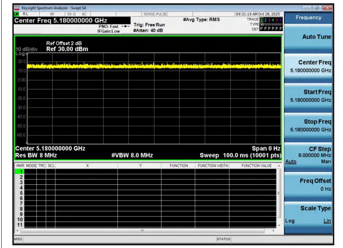
NTNV-11AX20MIMO-Ant2-5180
