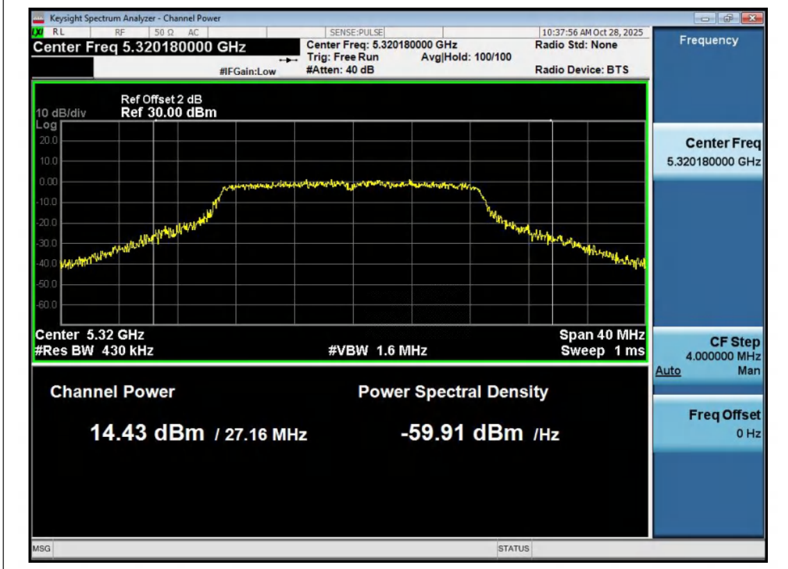
11N20MIMO-Ant2-5320-PASS
