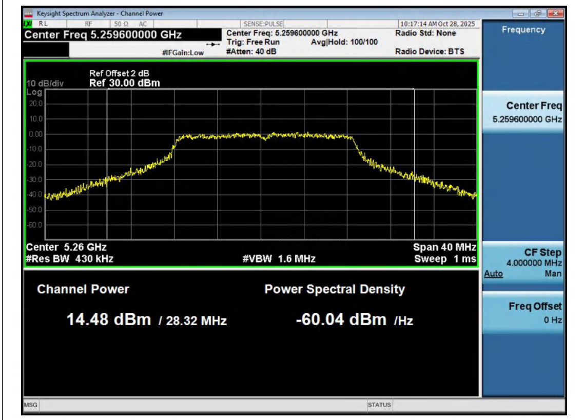
11A-Ant2-5260-PASS
