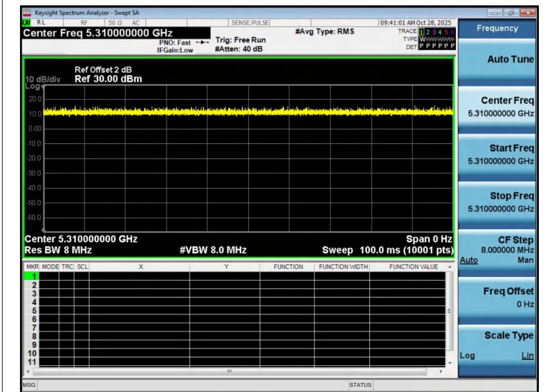
NTNV-11AX40MIMO-Ant2-5310
