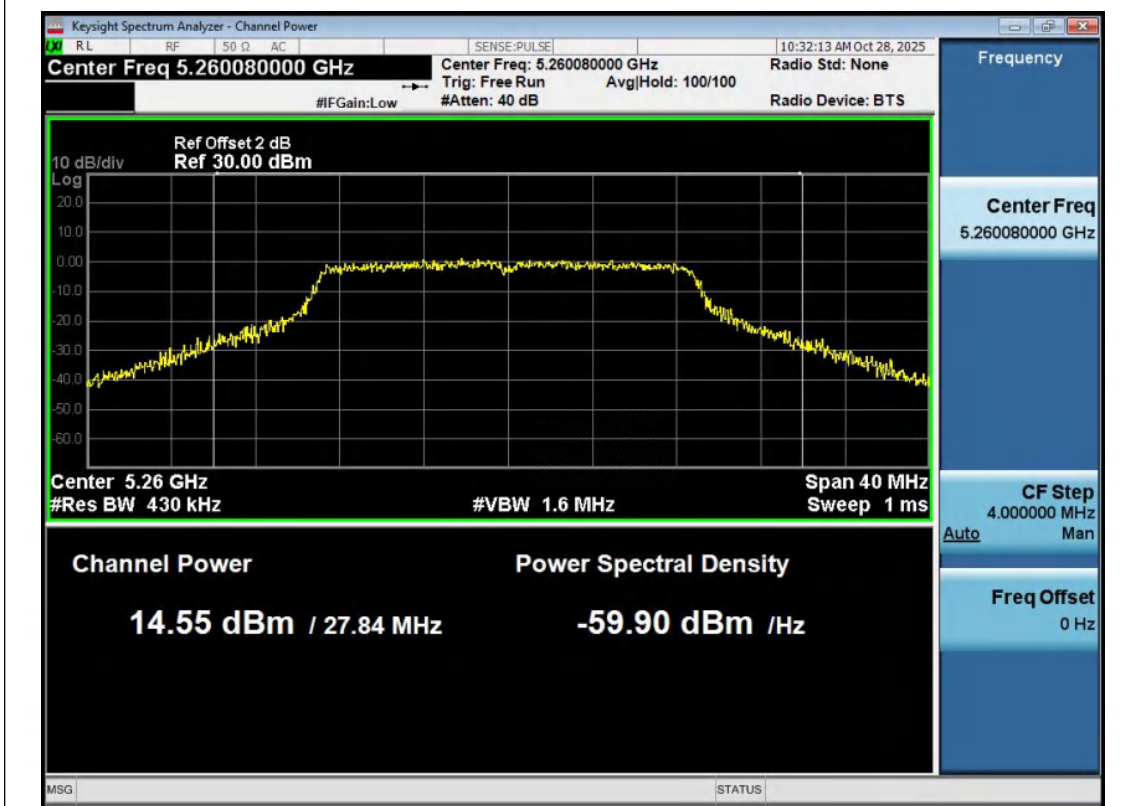
11N20MIMO-Ant2-5260-PASS
