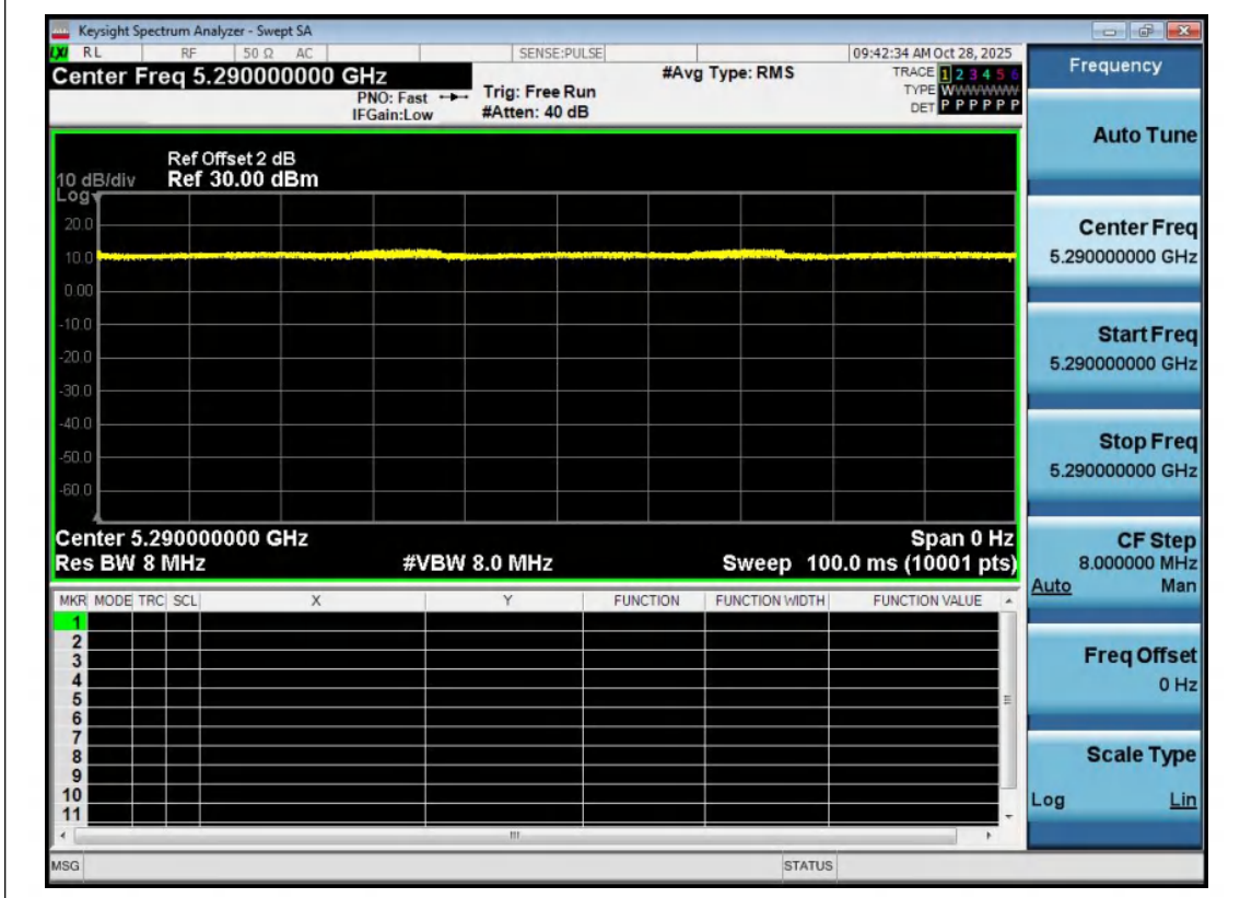
NTNV-11AX80MIMO-Ant2-5290
