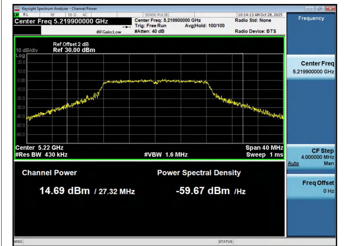
11A-Ant2-5220-PASS
