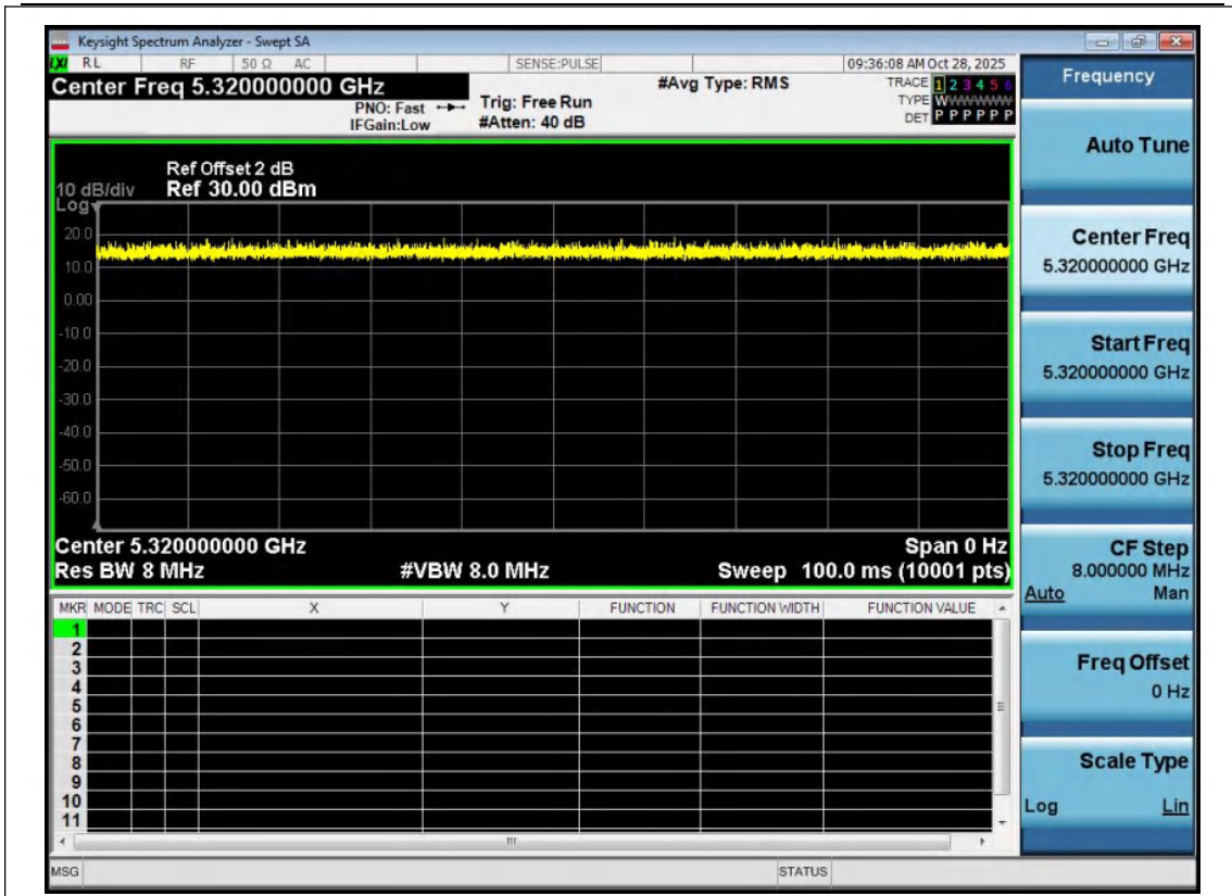
NTNV-11AX20MIMO-Ant2-5320
