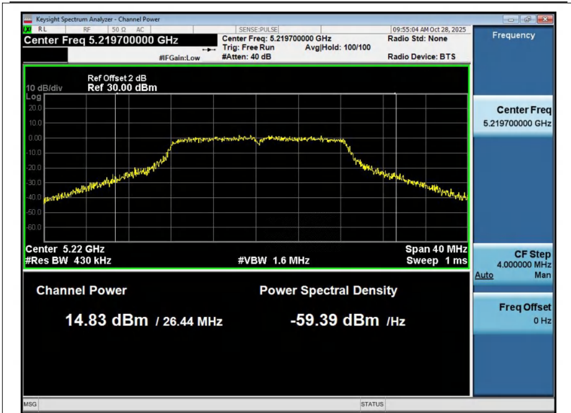
11A-Ant1-5220-PASS
