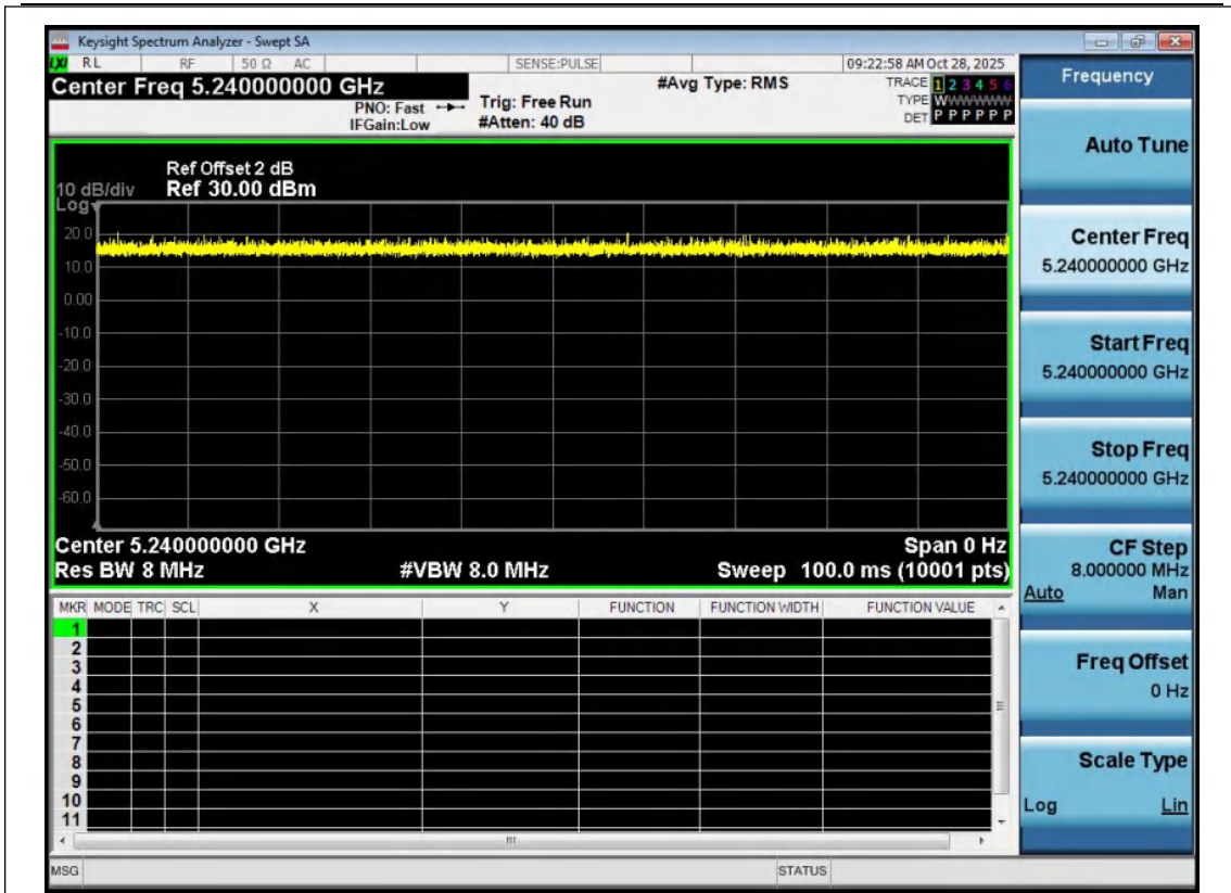
NTNV-11AC20MIMO-Ant1-5240
