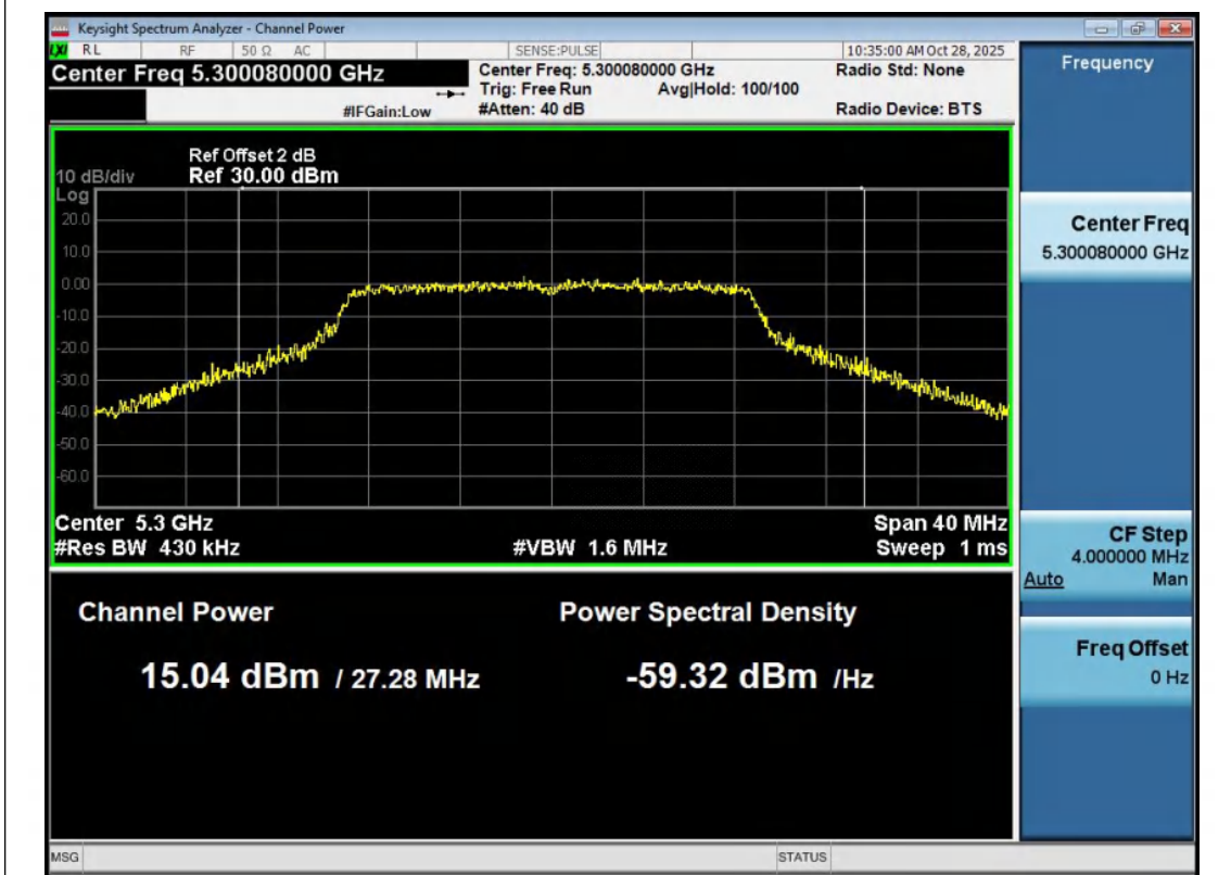
11N20MIMO-Ant2-5300-PASS
