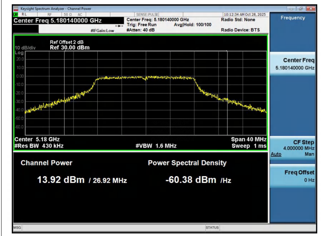
11A-Ant2-5180-PASS
