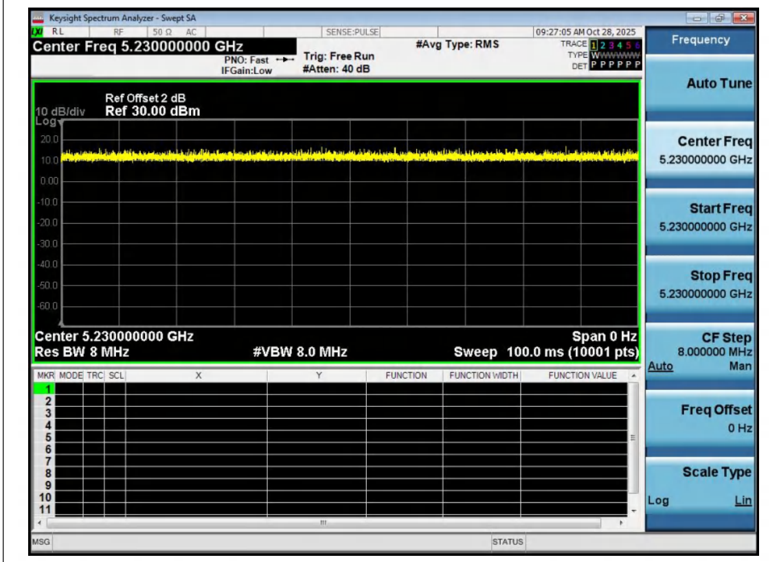
NTNV-11AC40MIMO-Ant2-5230
