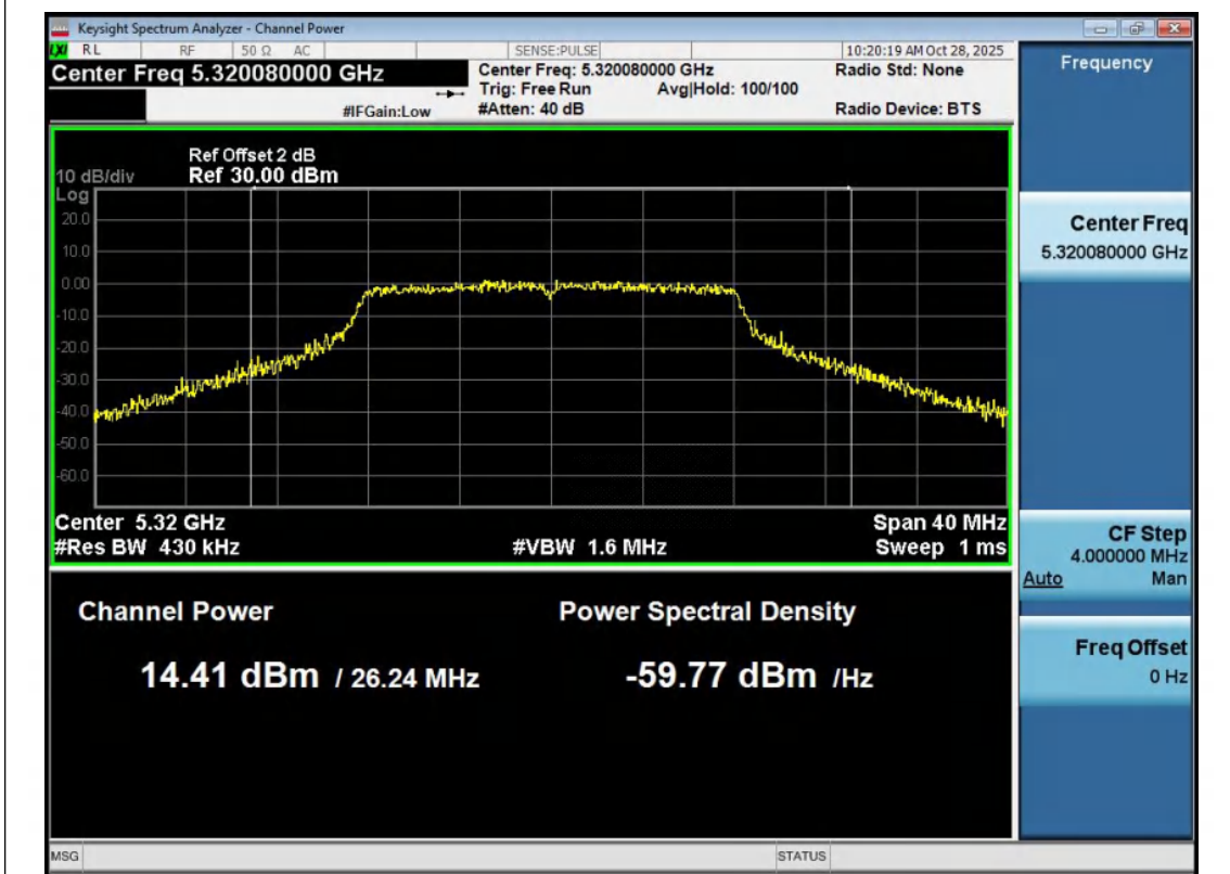
11A-Ant2-5320-PASS
