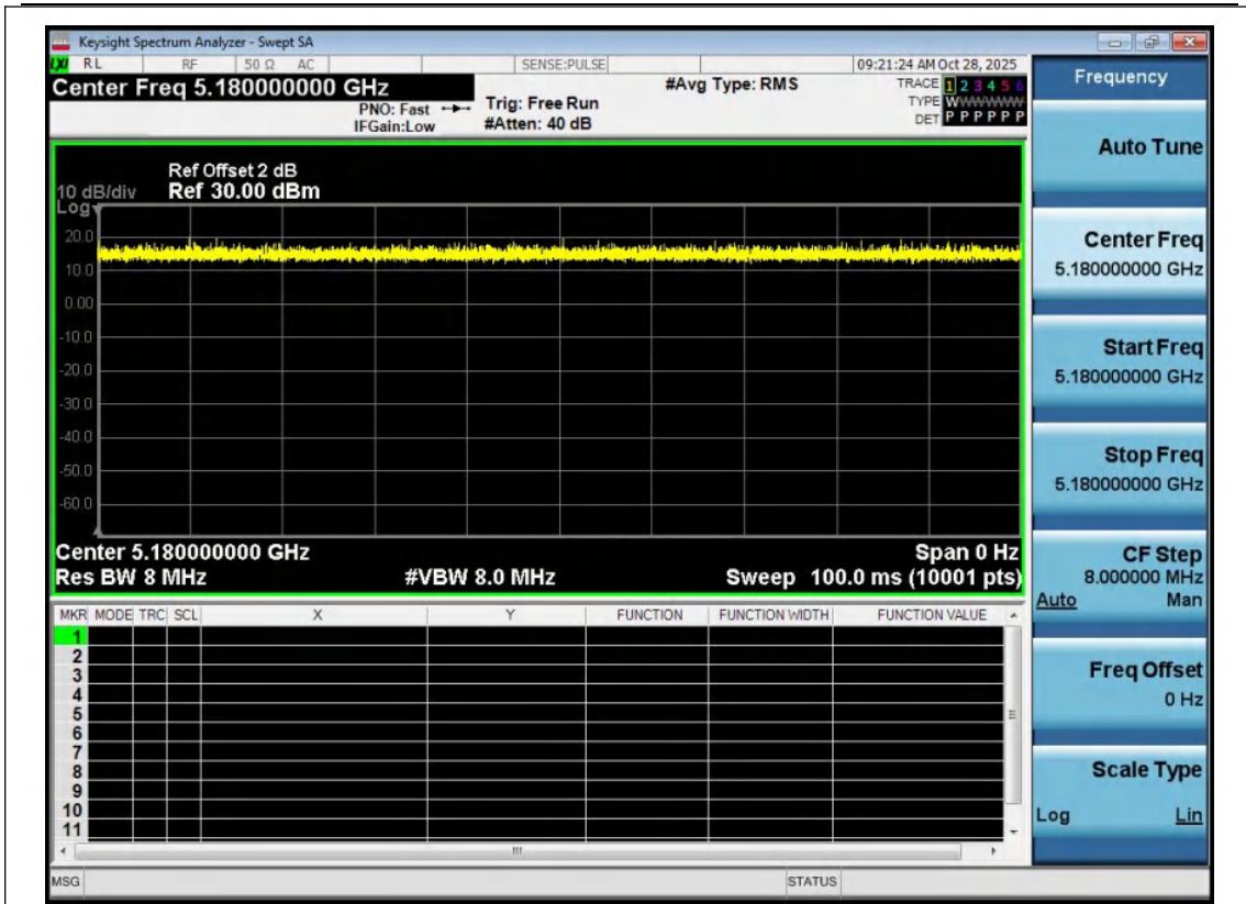
NTNV-11AC20MIMO-Ant1-5180
