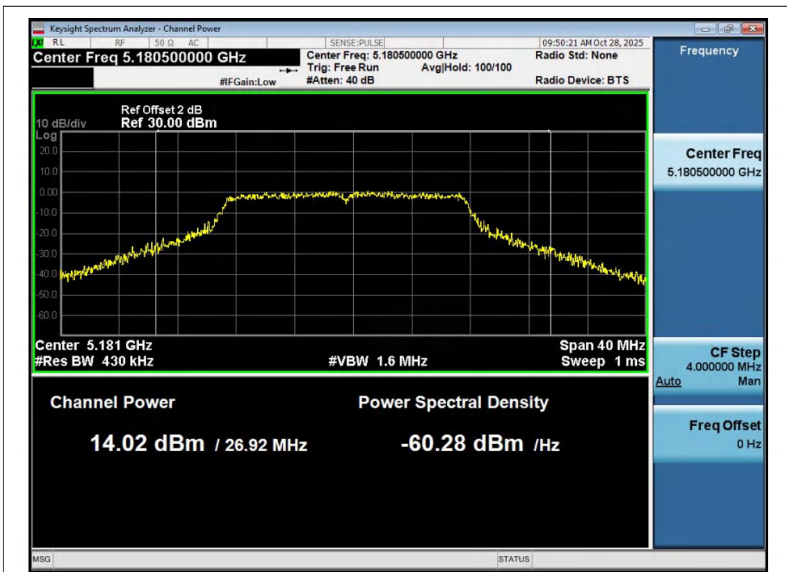
11A-Ant1-5180-PASS
