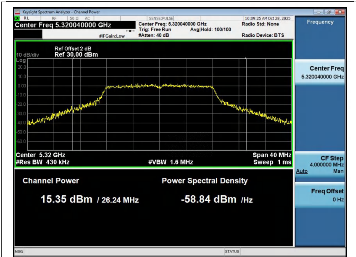
11A-Ant1-5320-PASS
