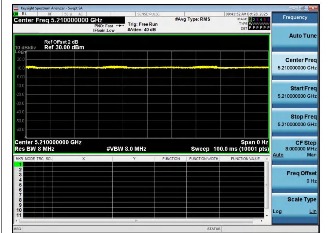
NTNV-11AX80MIMO-Ant2-5210
