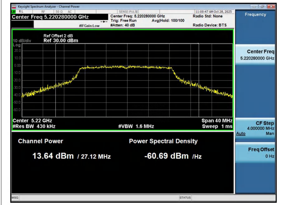
11AC20MIMO-Ant2-5220-PASS
