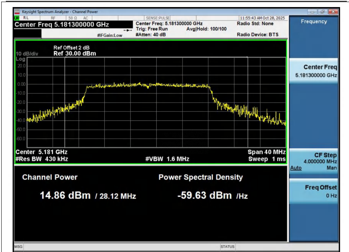
11AX20MIMO-Ant1-5180-PASS
