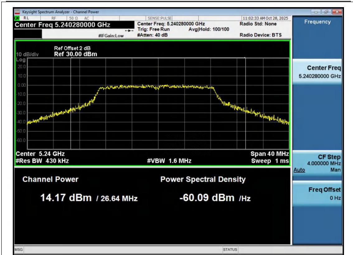
11AC20MIMO-Ant1-5240-PASS
