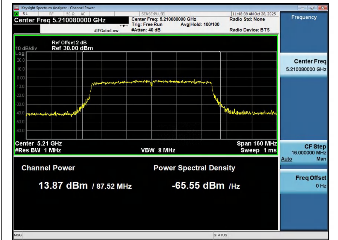
11AC80MIMO-Ant2-5210-PASS
