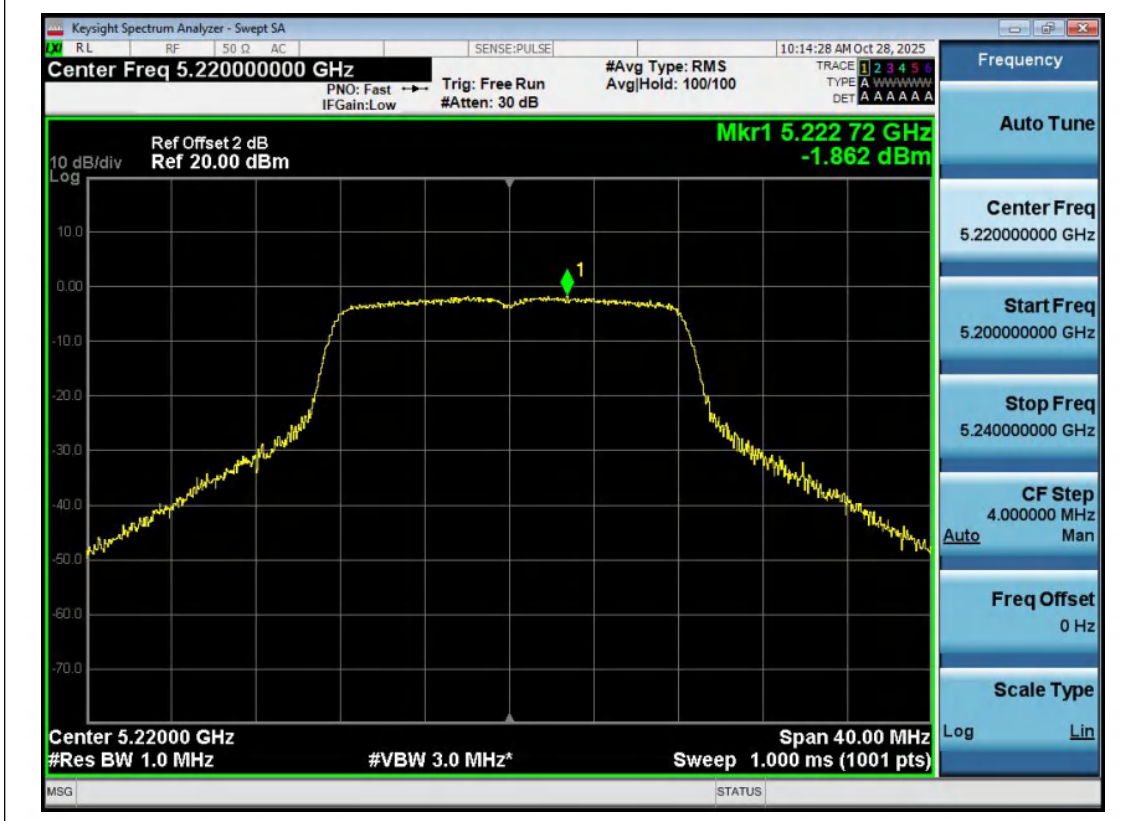
11A-Ant2-5220-PASS
