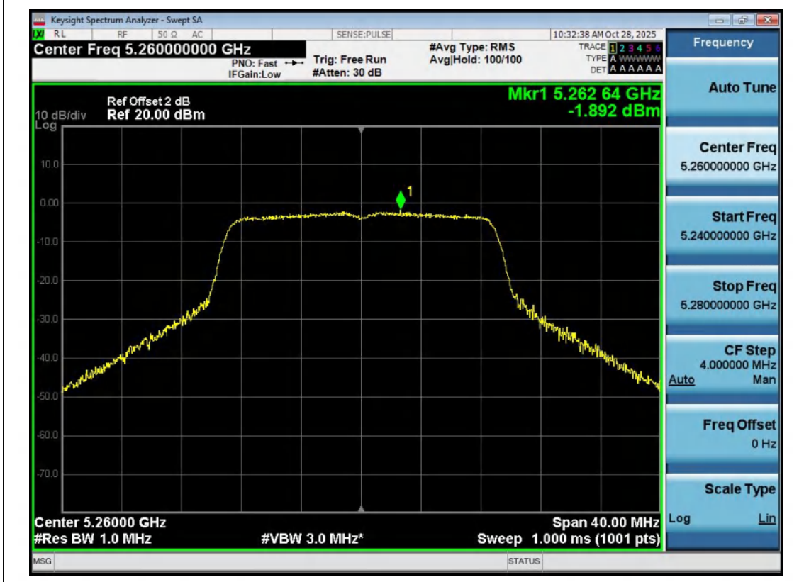
11N20MIMO-Ant2-5260-PASS
