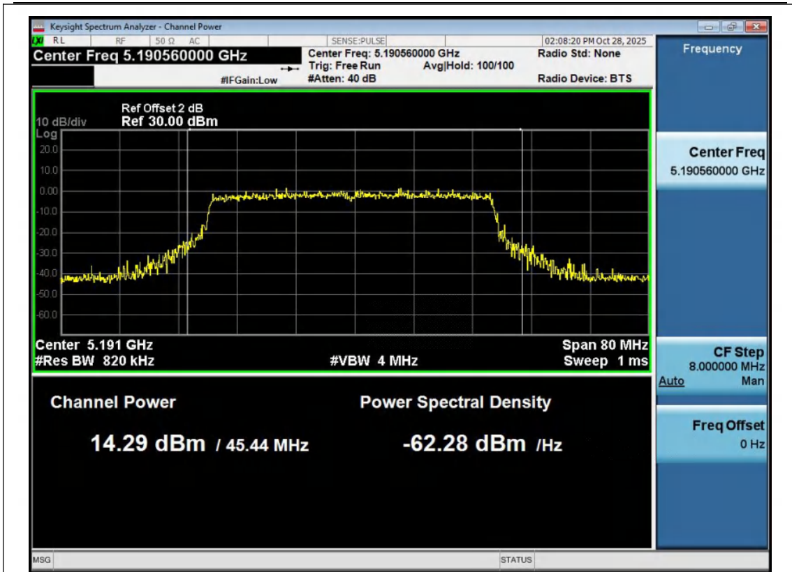
11AX40MIMO-Ant1-5190-PASS
