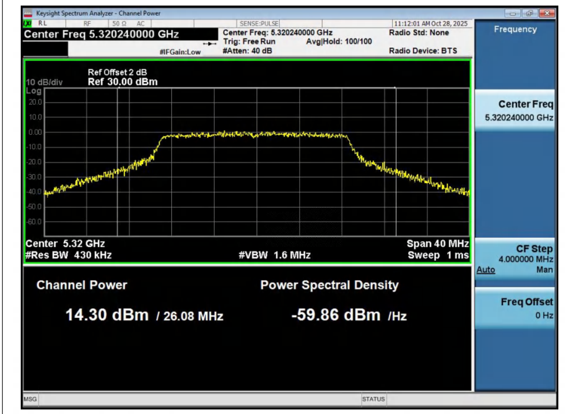
11AC20MIMO-Ant2-5320-PASS
