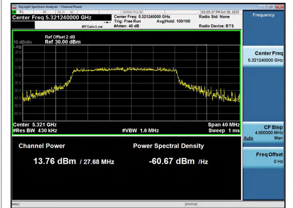
11AX20MIMO-Ant2-5320-PASS
