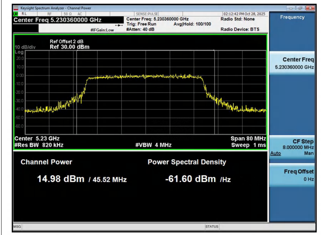
11AX40MIMO-Ant2-5230-PASS
