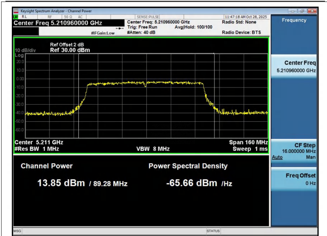
11AC80MIMO-Ant1-5210-PASS
