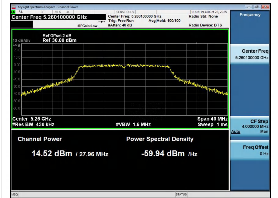
11AC20MIMO-Ant2-5260-PASS
