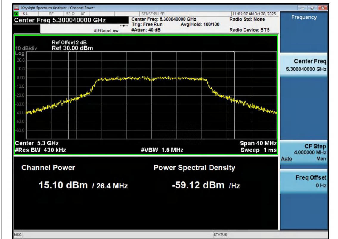
11AC20MIMO-Ant2-5300-PASS
