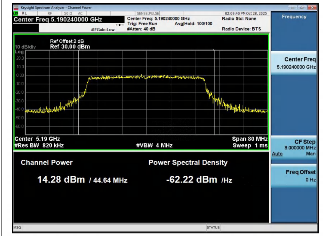
11AX40MIMO-Ant2-5190-PASS
