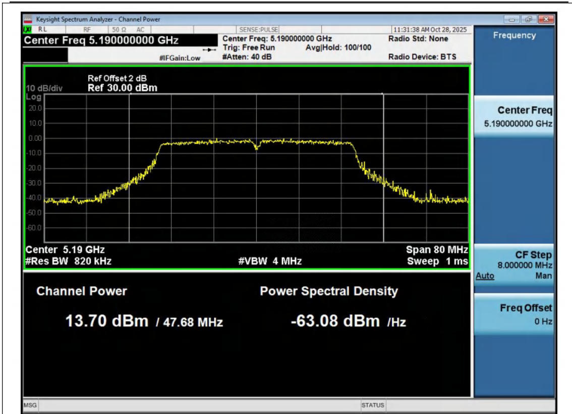
11AC40MIMO-Ant1-5190-PASS
