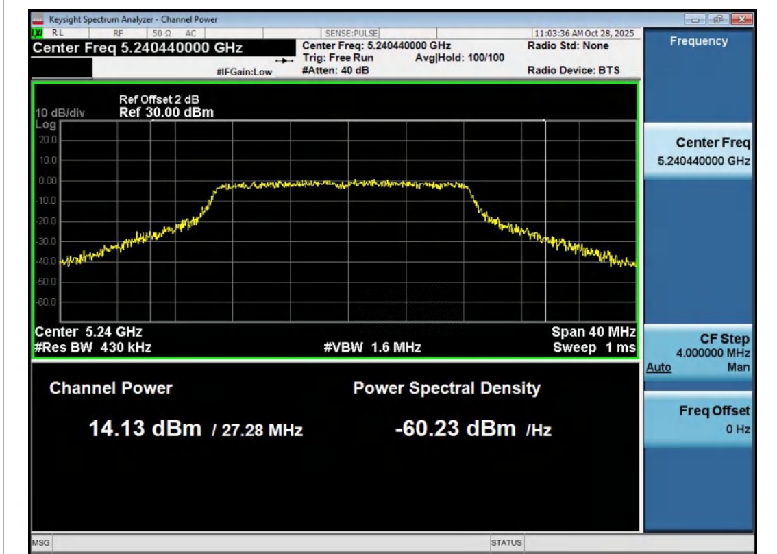
11AC20MIMO-Ant2-5240-PASS
