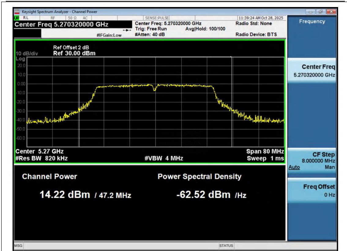
11AC40MIMO-Ant1-5270-PASS
