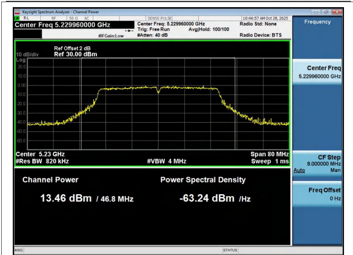
11N40MIMO-Ant1-5230-PASS
