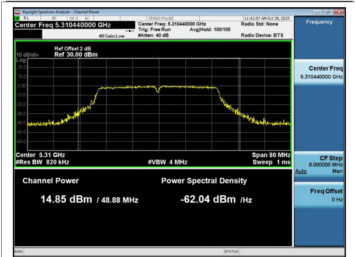
11AC40MIMO-Ant1-5310-PASS
