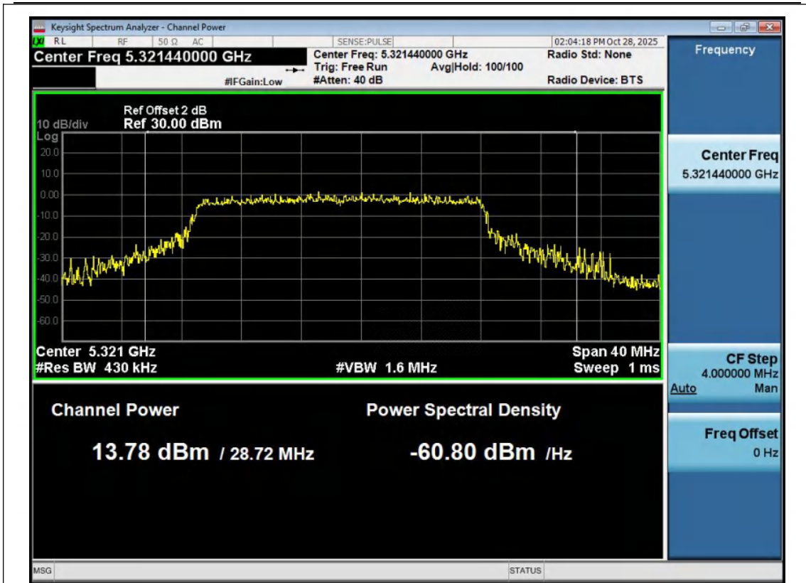
11AX20MIMO-Ant1-5320-PASS
