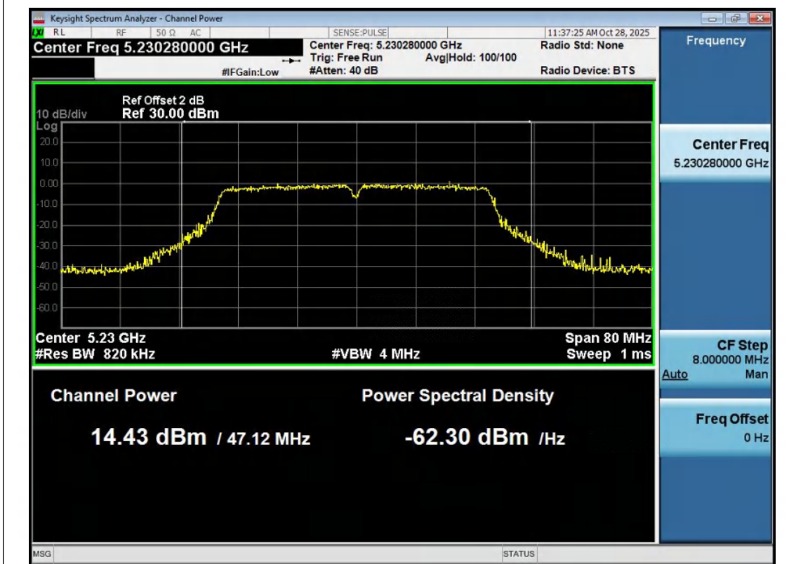
11AC40MIMO-Ant2-5230-PASS
