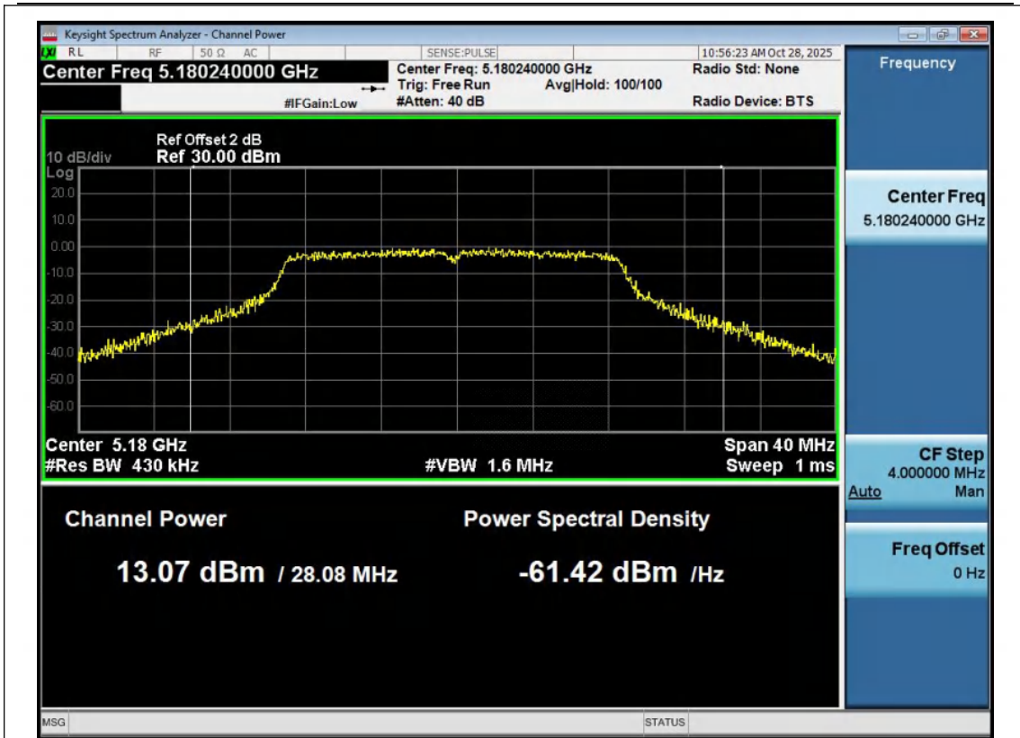
11AC20MIMO-Ant1-5180-PASS
