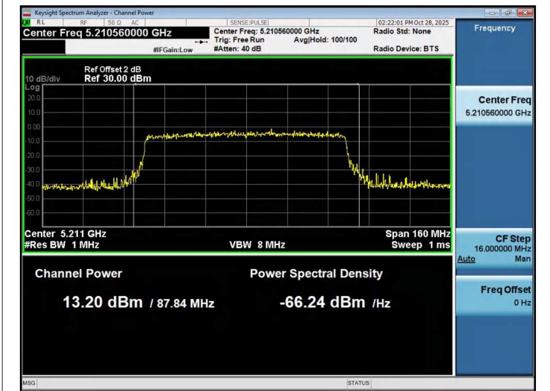
11AX80MIMO-Ant2-5210-PASS
