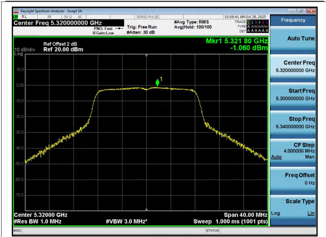
11A-Ant1-5320-PASS
