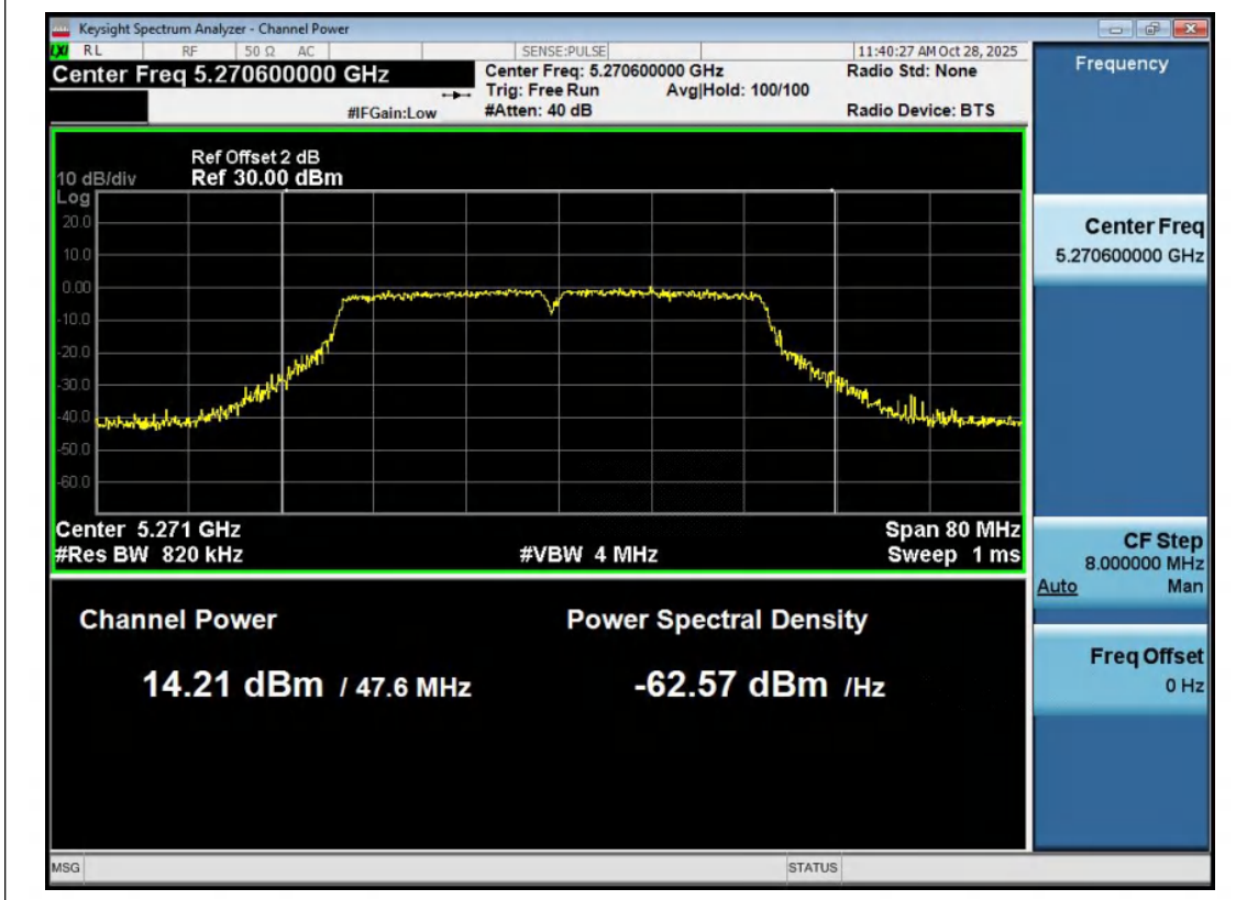
11AC40MIMO-Ant2-5270-PASS
