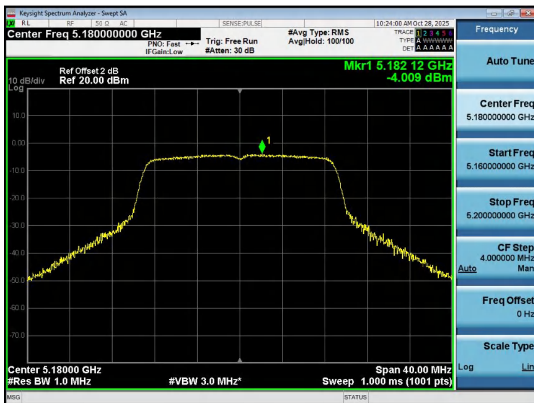
11N20MIMO-Ant2-5180-PASS
