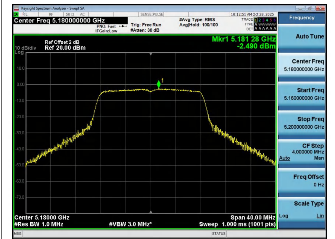
11A-Ant2-5180-PASS
