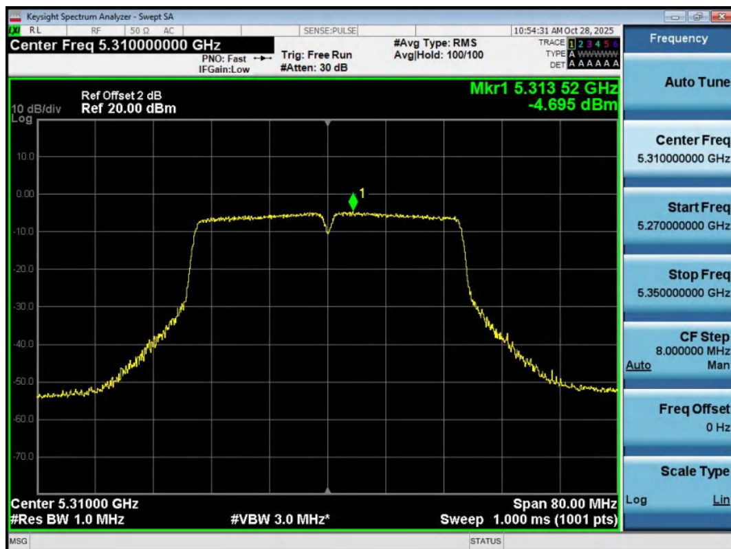
11N40MIMO-Ant2-5310-PASS
