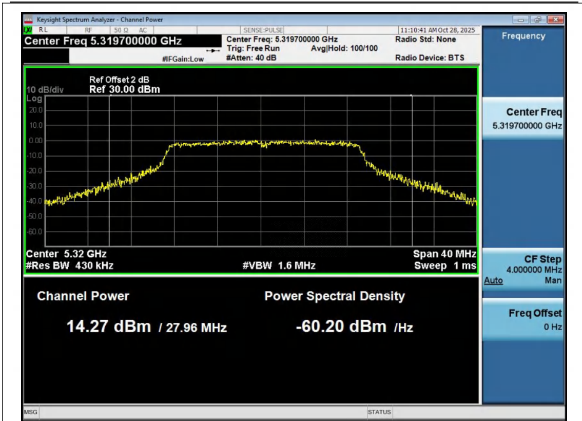
11AC20MIMO-Ant1-5320-PASS
