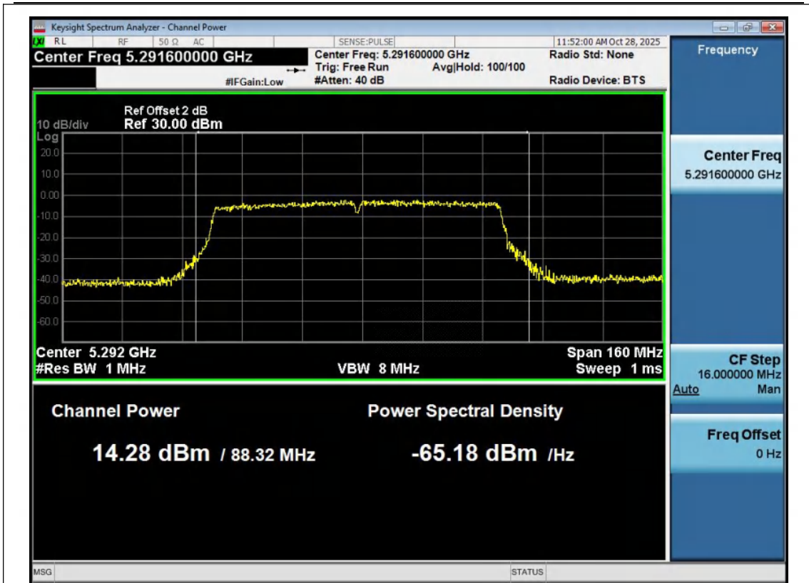
11AC80MIMO-Ant1-5290-PASS
