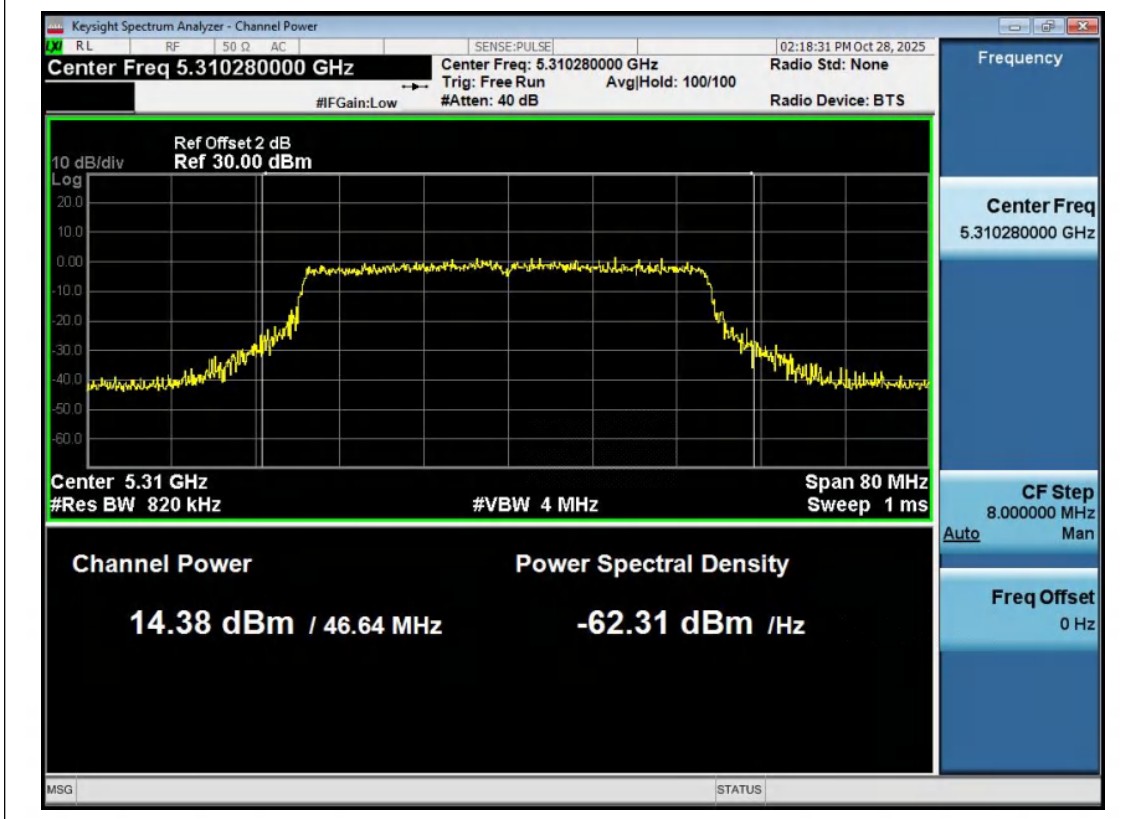
11AX40MIMO-Ant2-5310-PASS
