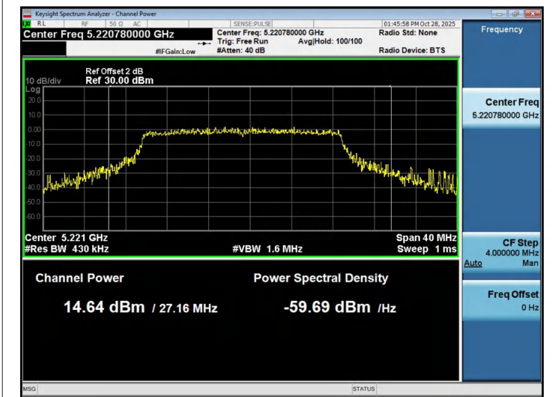
11AX20MIMO-Ant2-5220-PASS
