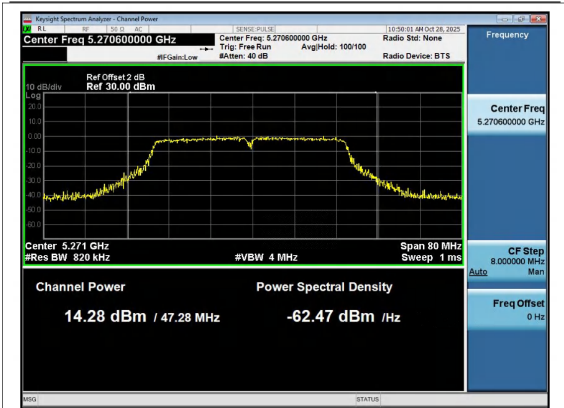
11N40MIMO-Ant1-5270-PASS
