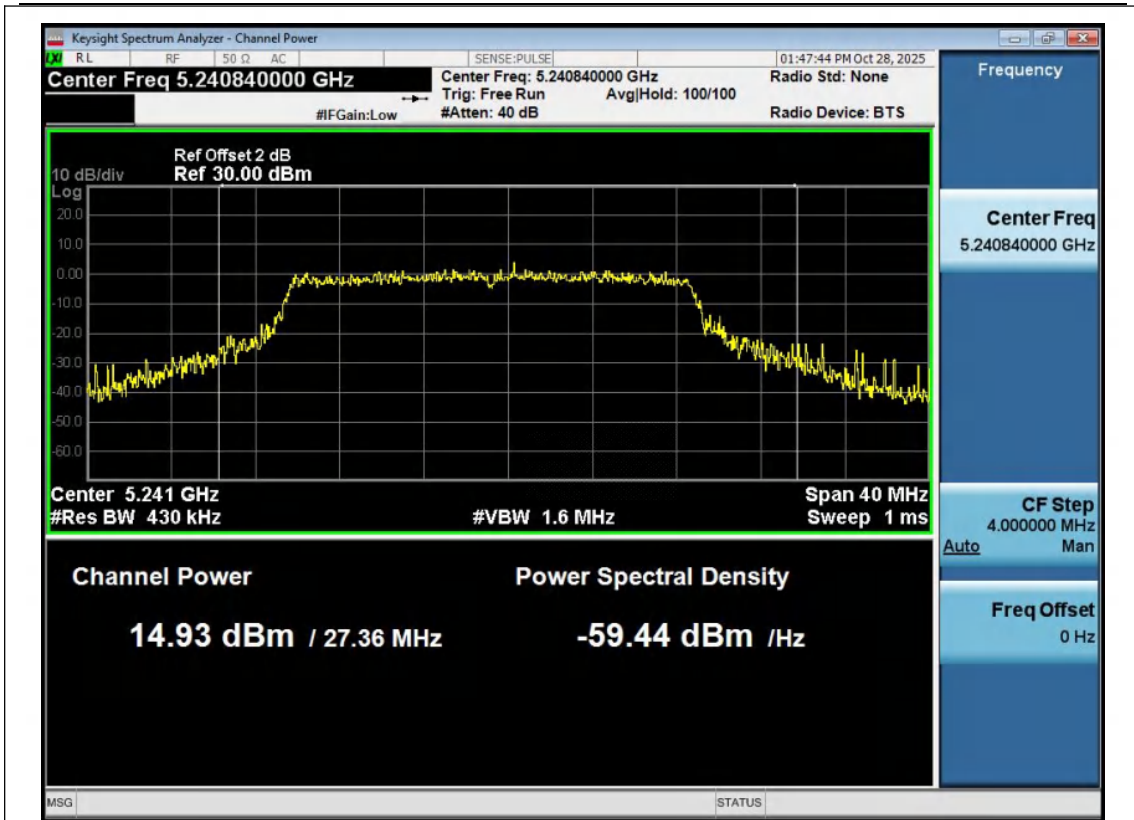
11AX20MIMO-Ant1-5240-PASS
