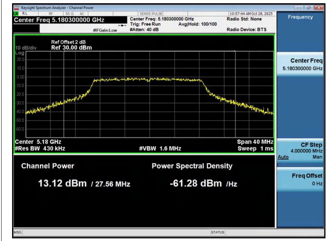
11AC20MIMO-Ant2-5180-PASS
