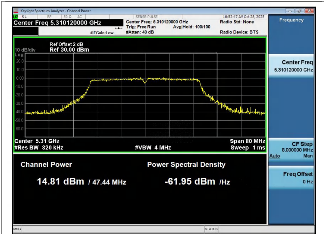
11N40MIMO-Ant1-5310-PASS
