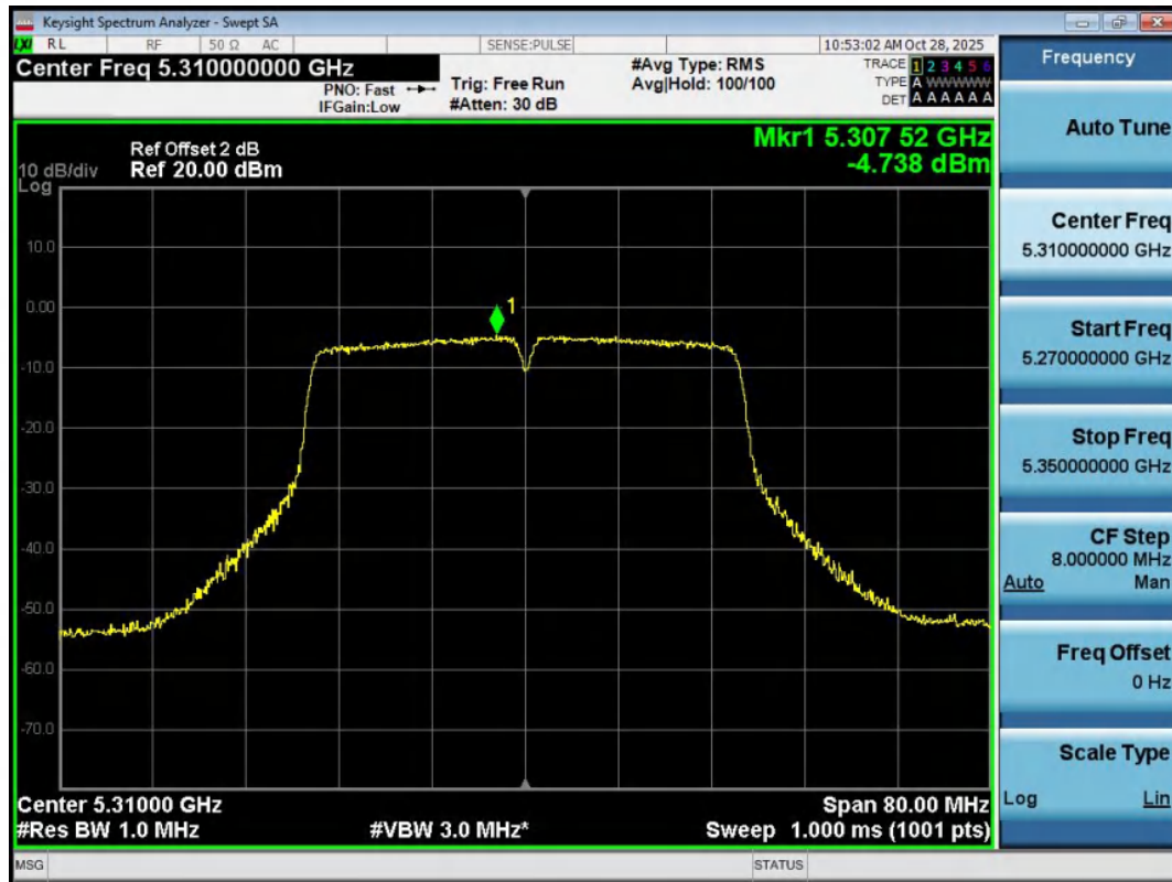
11N40MIMO-Ant1-5310-PASS
