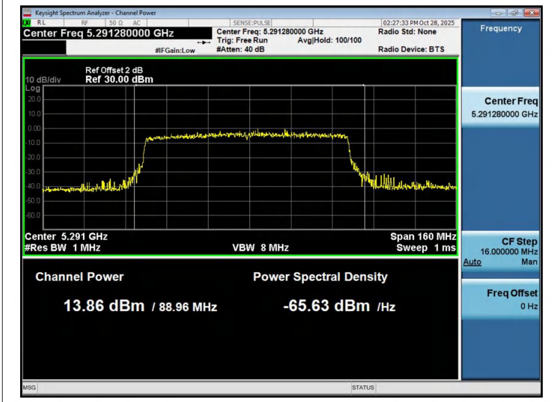
11AX80MIMO-Ant2-5290-PASS
