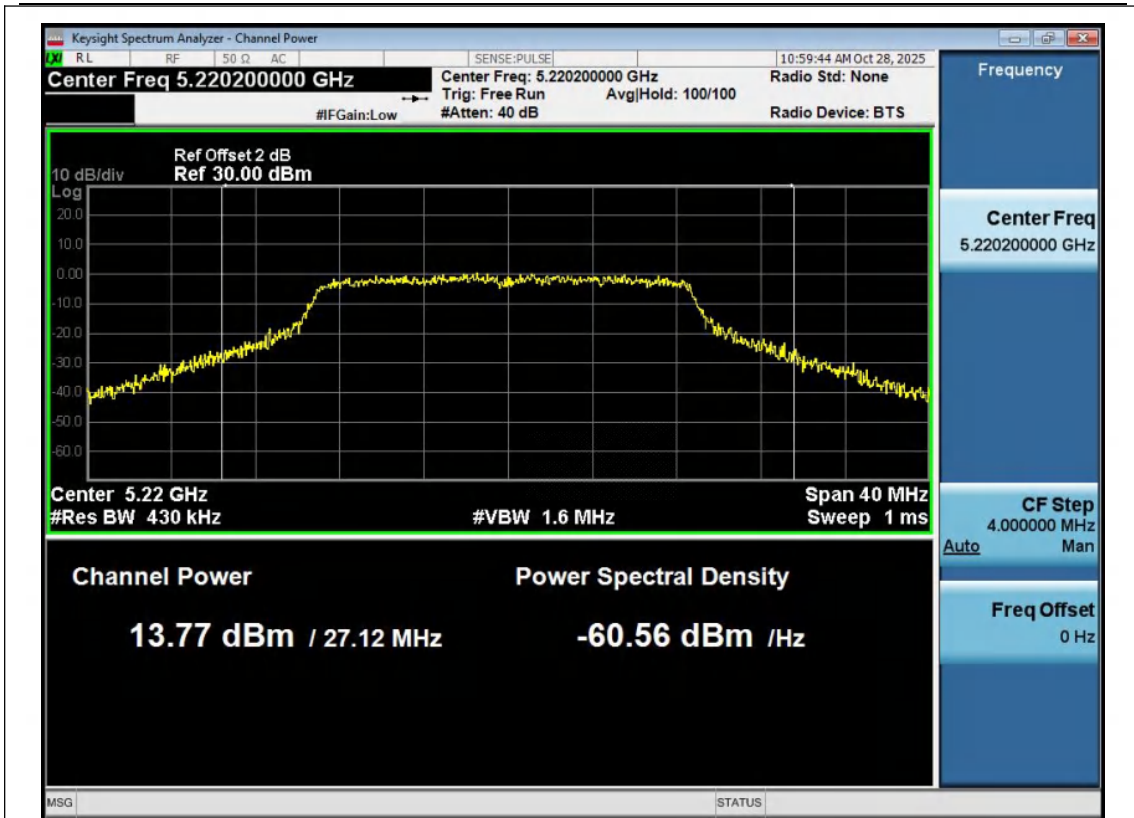
11AC20MIMO-Ant1-5220-PASS
