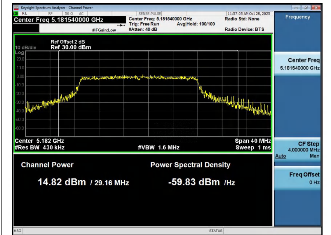
11AX20MIMO-Ant2-5180-PASS
