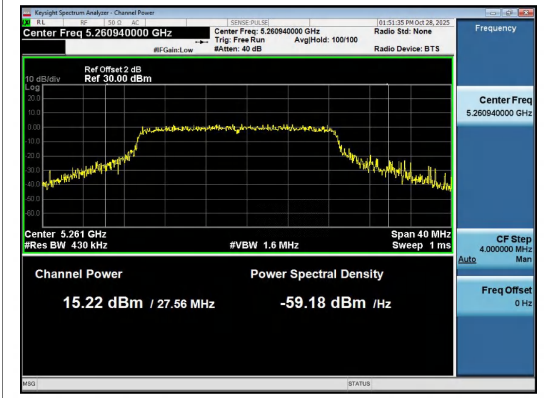
11AX20MIMO-Ant2-5260-PASS
