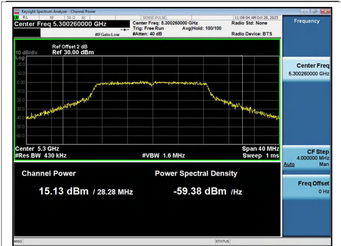
11AC20MIMO-Ant1-5300-PASS
