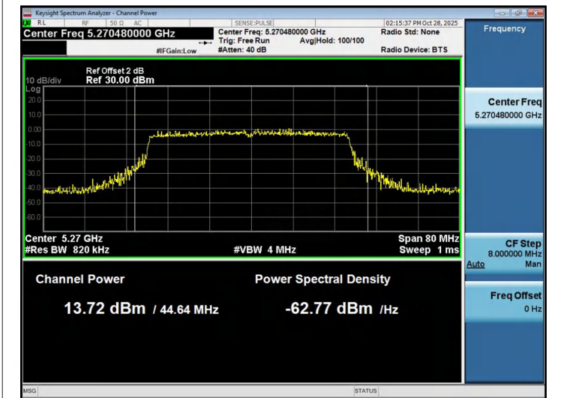
11AX40MIMO-Ant2-5270-PASS
