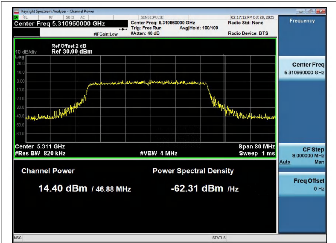
11AX40MIMO-Ant1-5310-PASS
