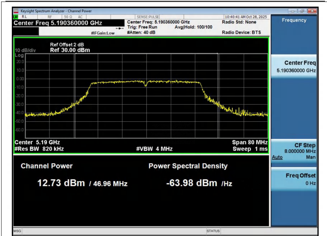
11N40MIMO-Ant1-5190-PASS
