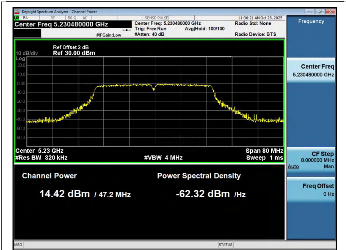
11AC40MIMO-Ant1-5230-PASS
