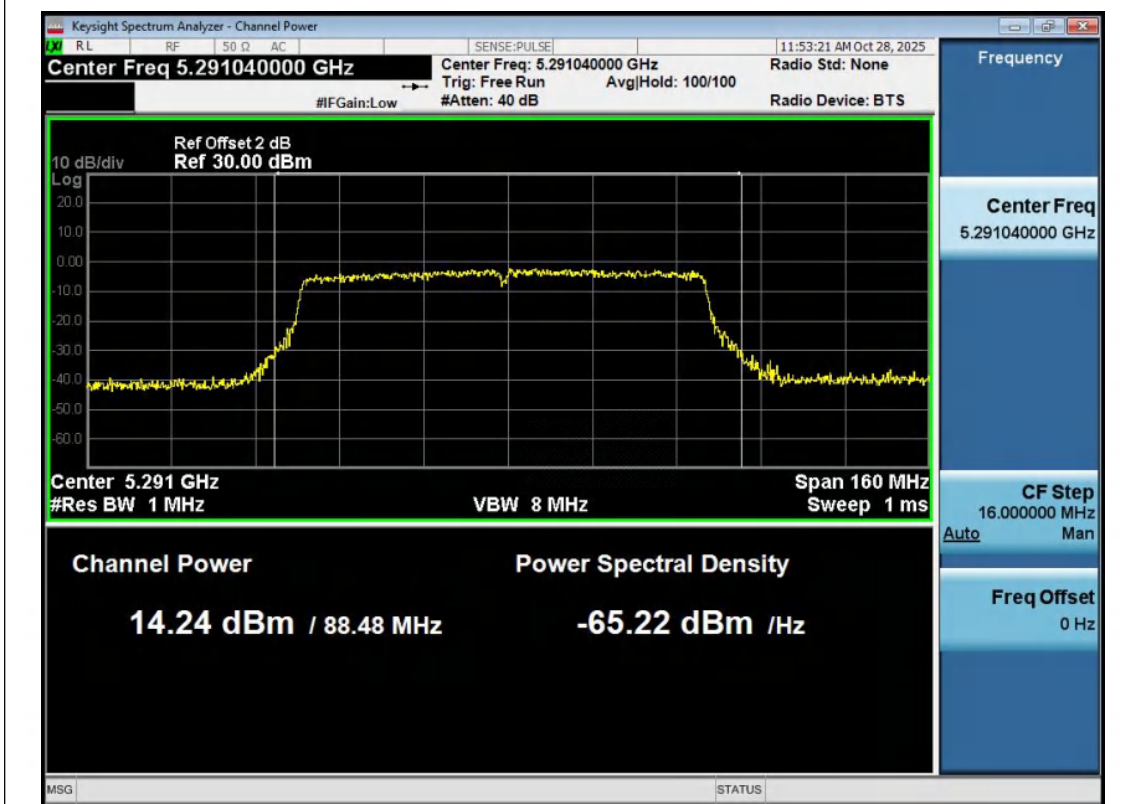
11AC80MIMO-Ant2-5290-PASS
