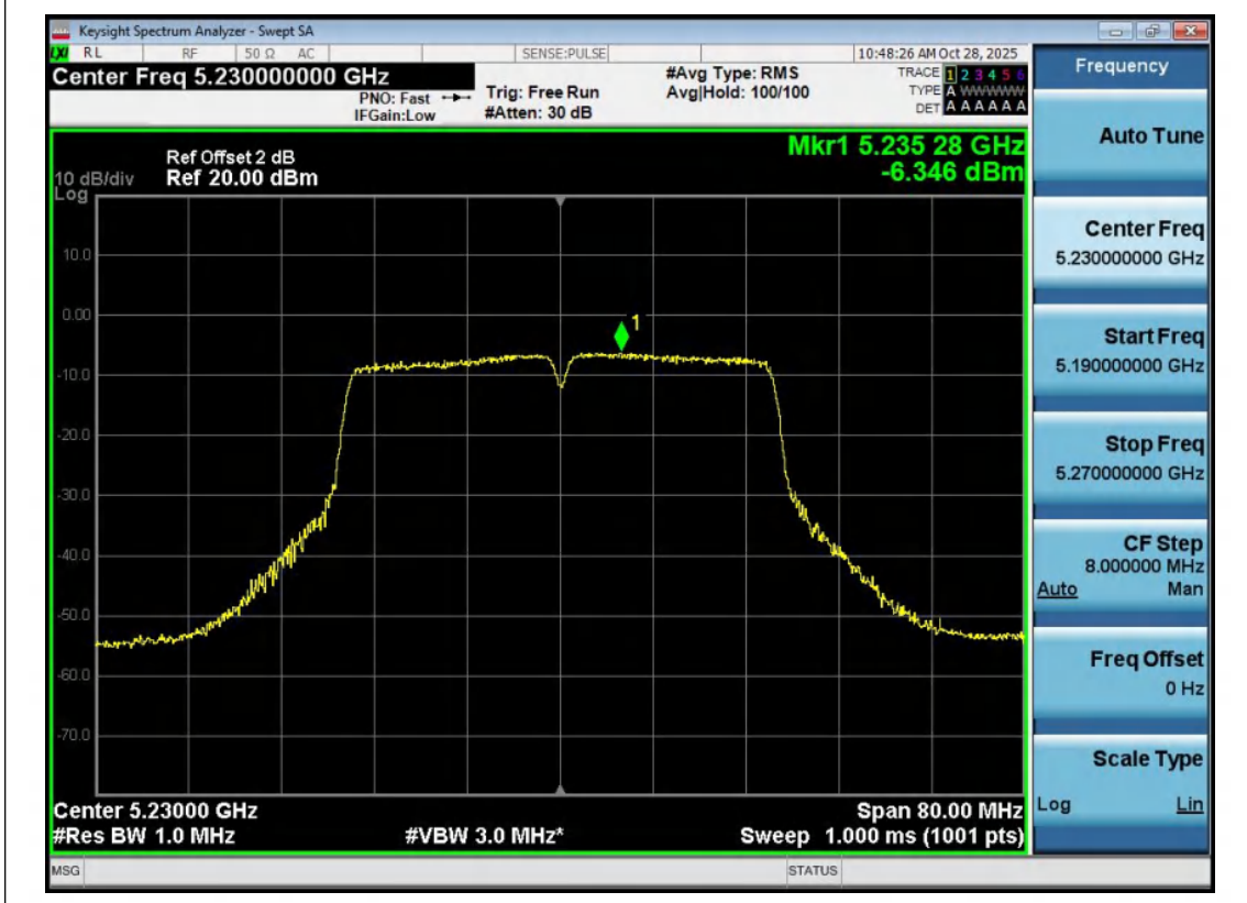
11N40MIMO-Ant2-5230-PASS
