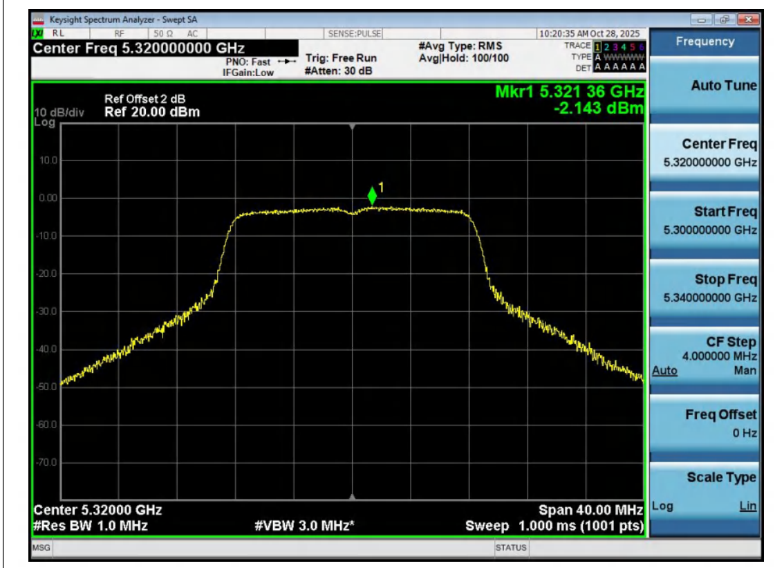
11A-Ant2-5320-PASS
