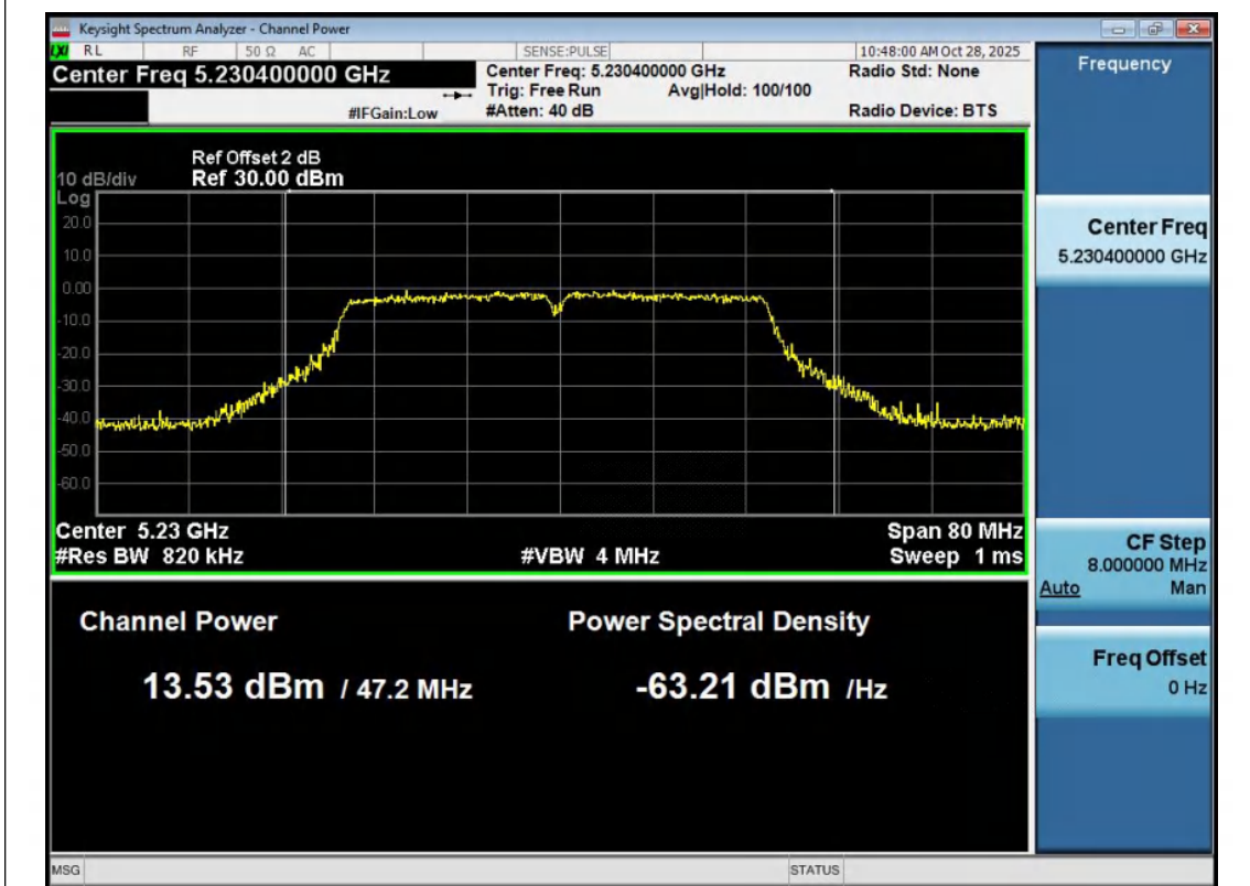
11N40MIMO-Ant2-5230-PASS
