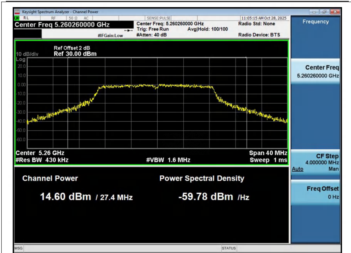
11AC20MIMO-Ant1-5260-PASS
