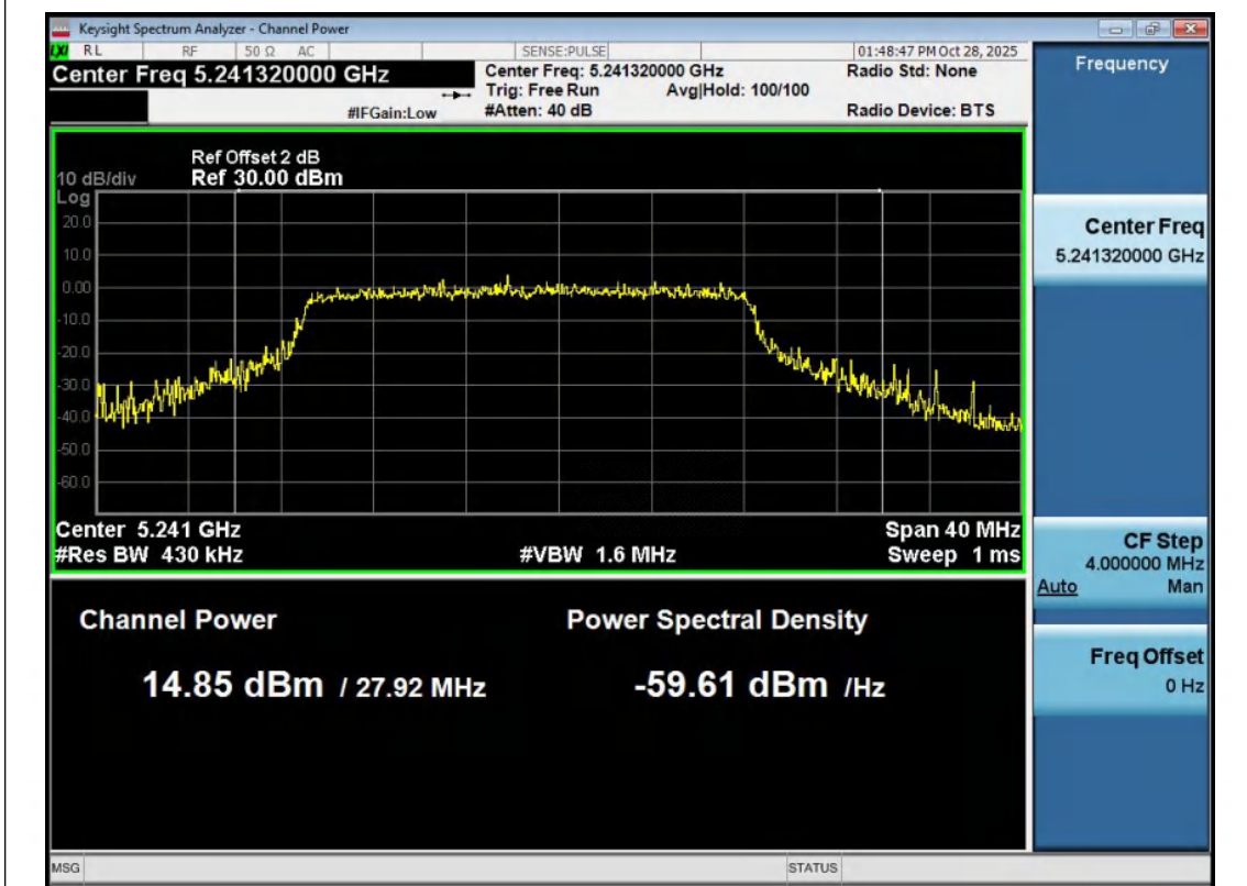
11AX20MIMO-Ant2-5240-PASS
