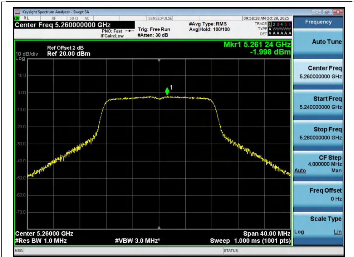
11A-Ant1-5260-PASS
