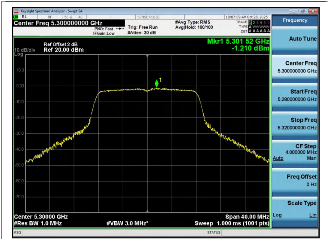
11A-Ant1-5300-PASS
