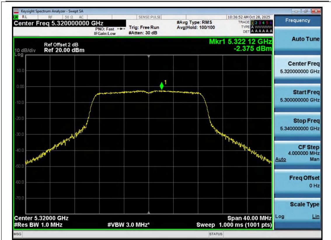
11N20MIMO-Ant1-5320-PASS
