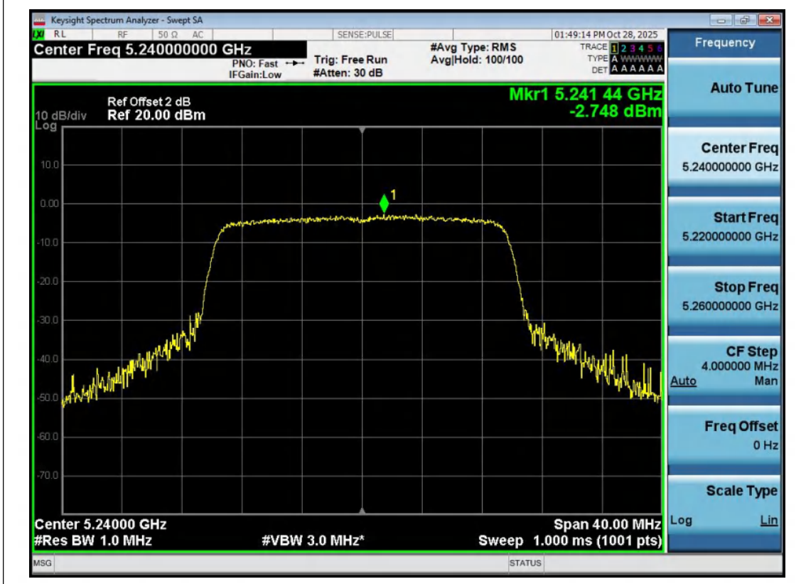
11AX20MIMO-Ant2-5240-PASS
