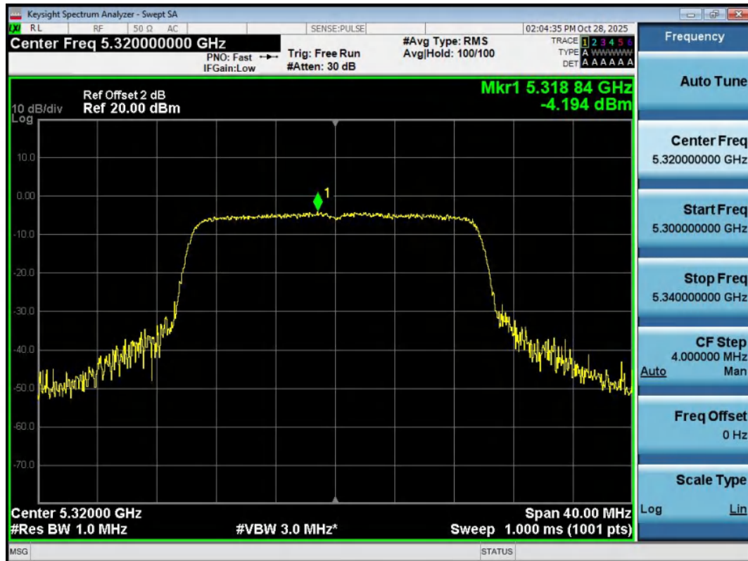
11AX20MIMO-Ant1-5320-PASS
