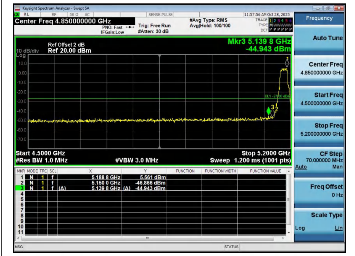
11AX20MIMO-Ant2-5180-PASS
