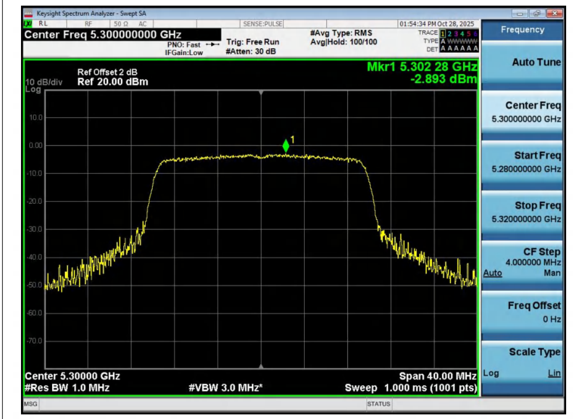
11AX20MIMO-Ant2-5300-PASS
