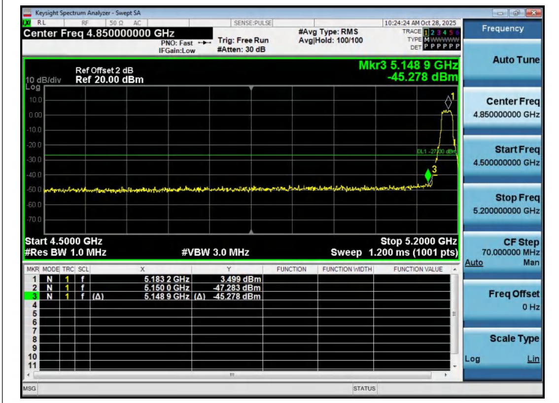
11N20MIMO-Ant2-5180-PASS
