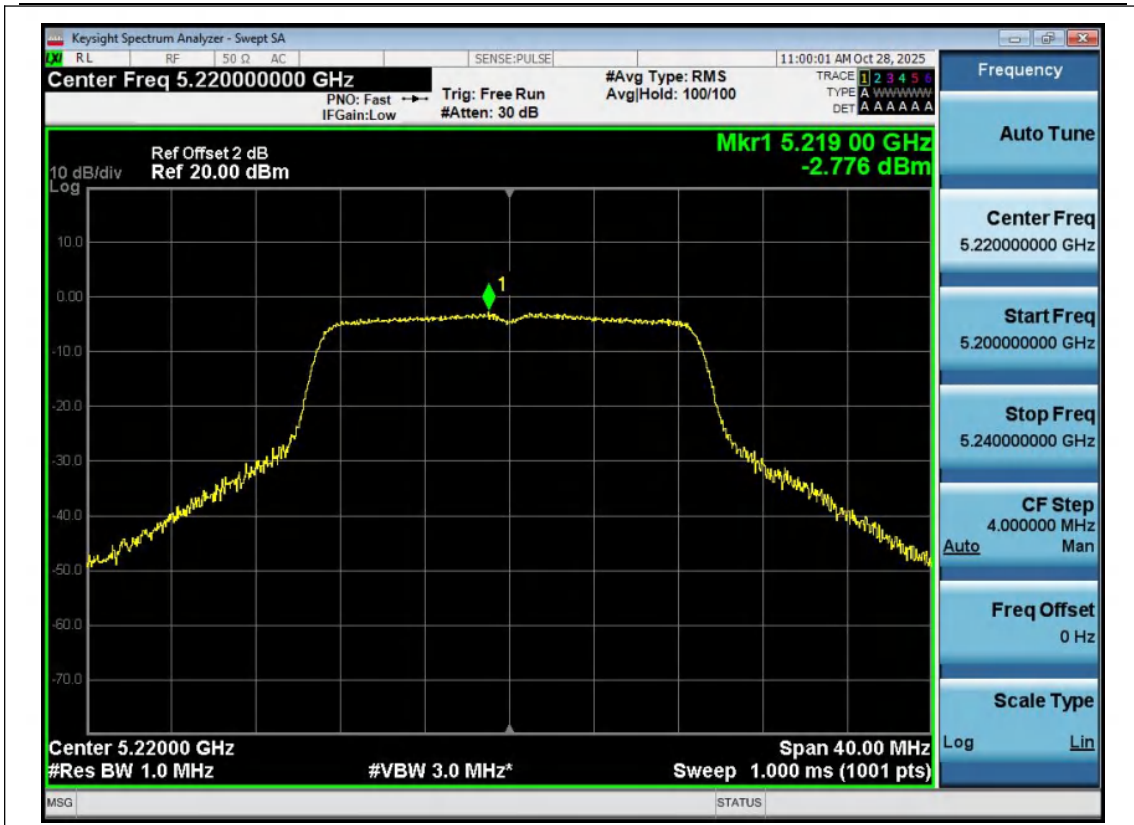
11AC20MIMO-Ant1-5220-PASS
