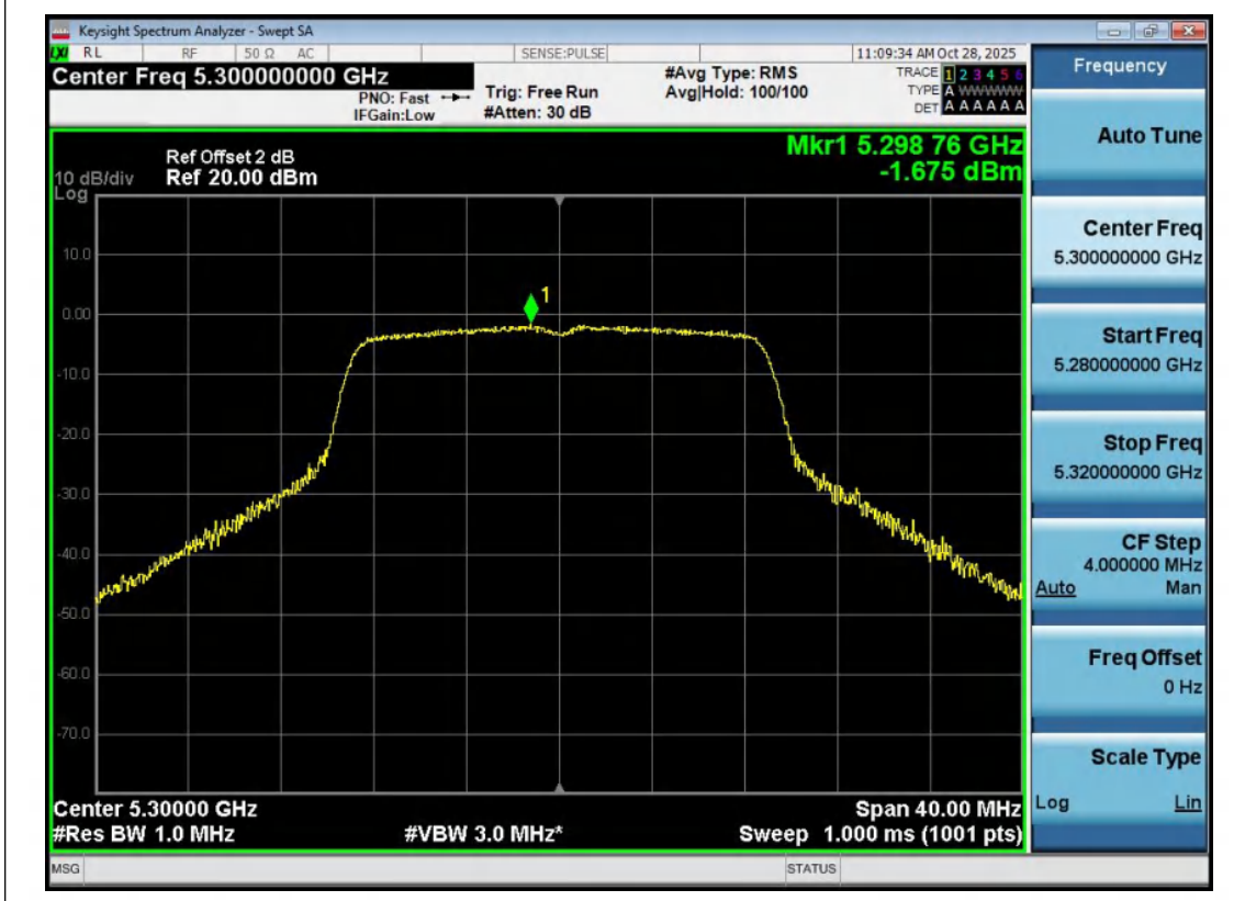
11AC20MIMO-Ant2-5300-PASS
