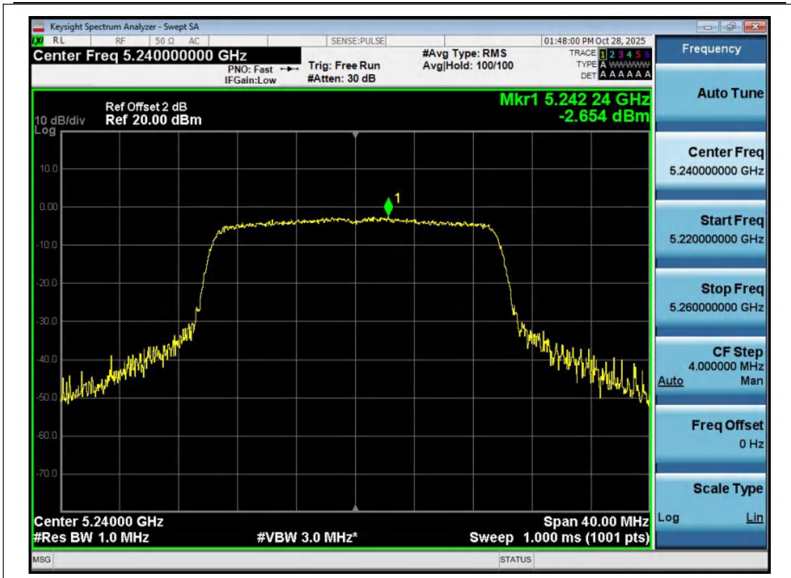
11AX20MIMO-Ant1-5240-PASS
