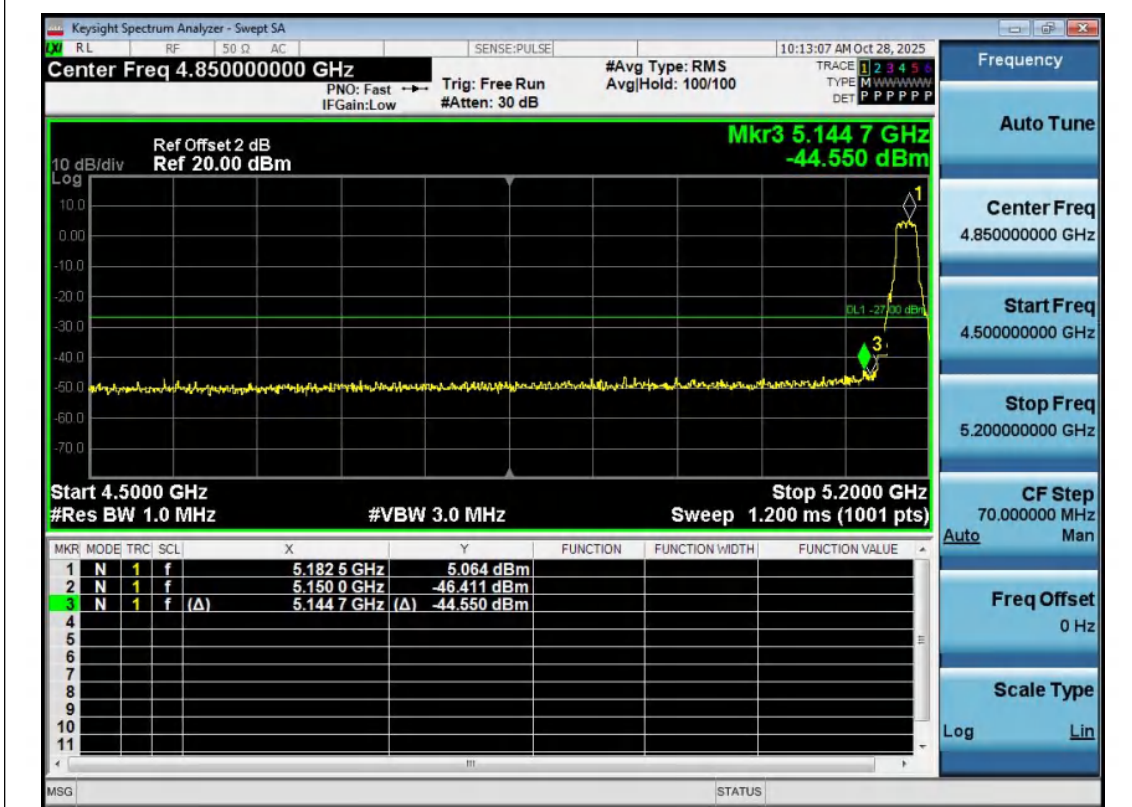
11A-Ant2-5180-PASS
