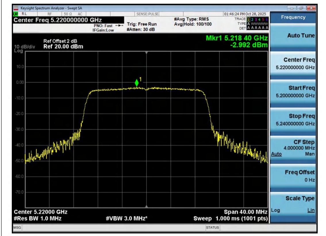
11AX20MIMO-Ant2-5220-PASS
