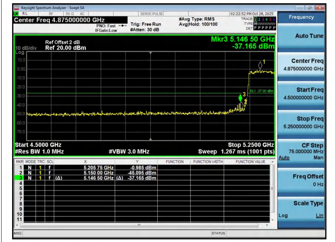
11AX80MIMO-Ant2-5210-PASS
