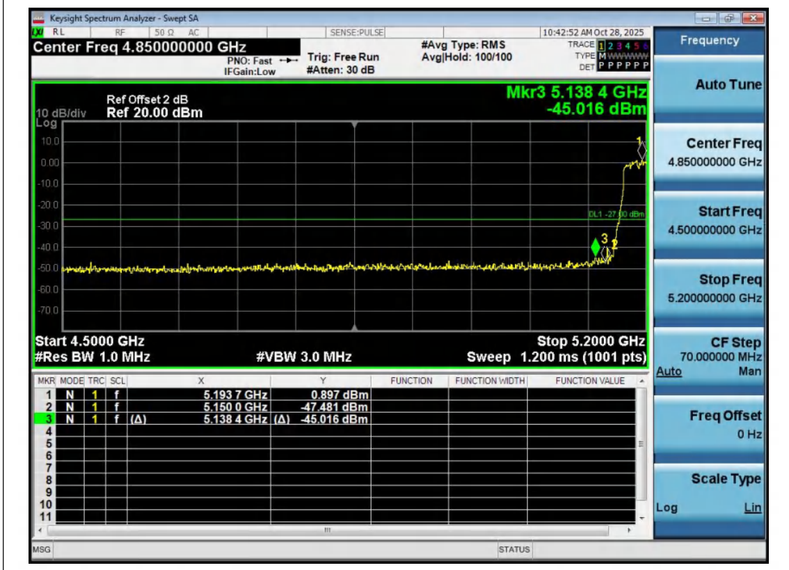
11N40MIMO-Ant2-5190-PASS
