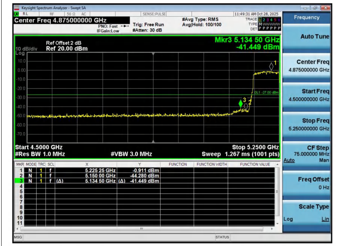
11AC80MIMO-Ant2-5210-PASS
