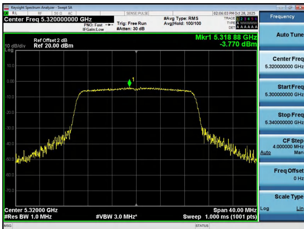
11AX20MIMO-Ant2-5320-PASS
