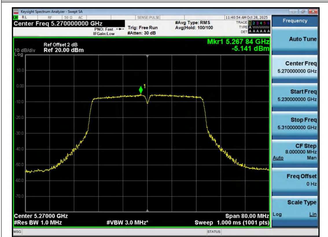
11AC40MIMO-Ant2-5270-PASS
