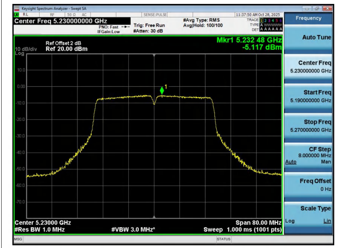
11AC40MIMO-Ant2-5230-PASS
