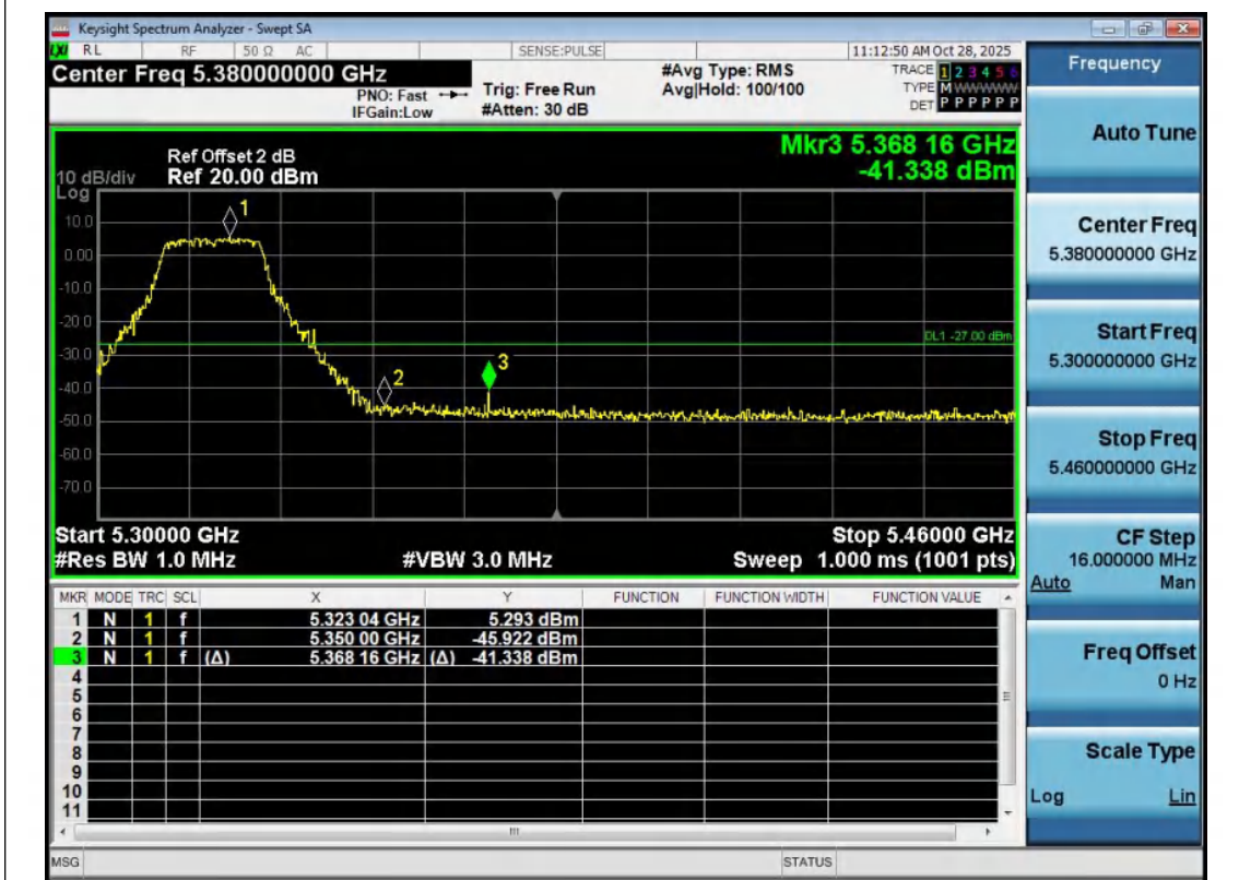
11AC20MIMO-Ant2-5320-PASS
