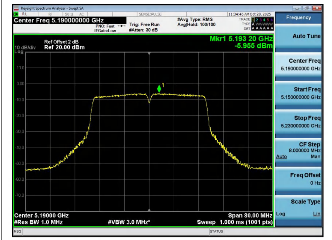
11AC40MIMO-Ant2-5190-PASS
