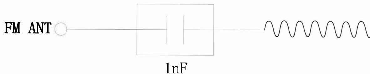
FM antenna connection diagram
