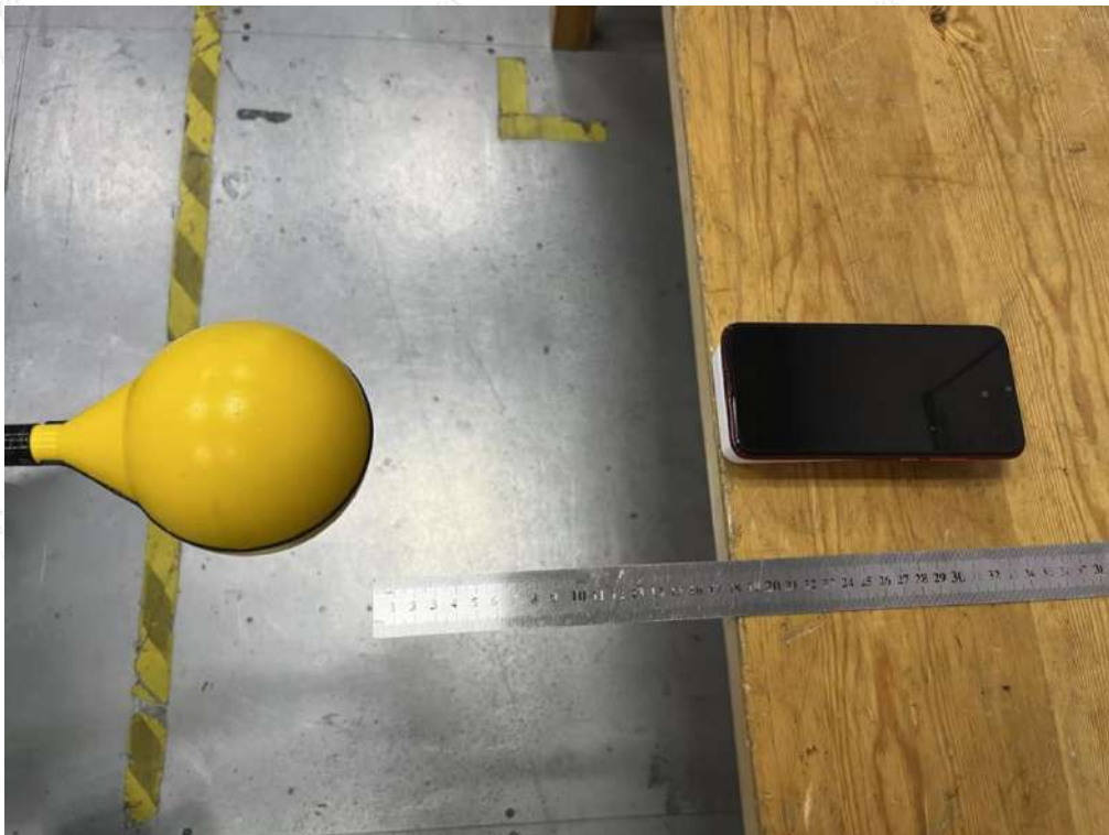
Test Position E(18cm) - Exposure photo from side edge surface-Right(TM1)
