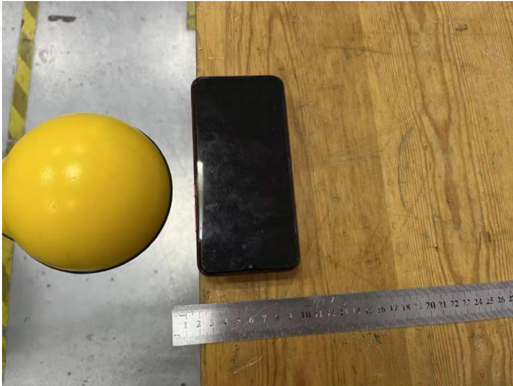
Test Position D(2cm) - Exposure photo from side edge surface-Front(TM1)
