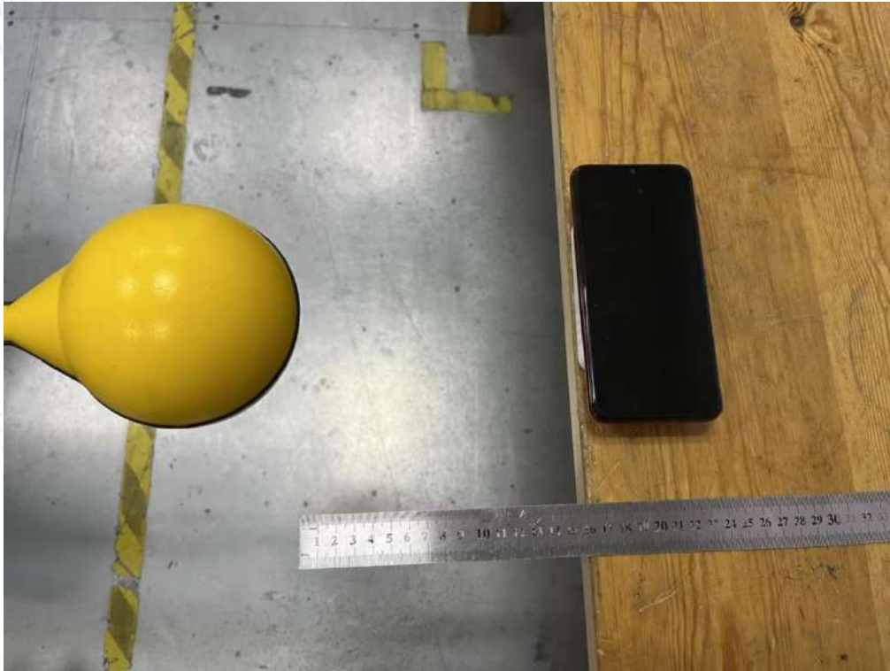
Test Position B(16cm) - Exposure photo from side edge surface-Rear(TM1)
