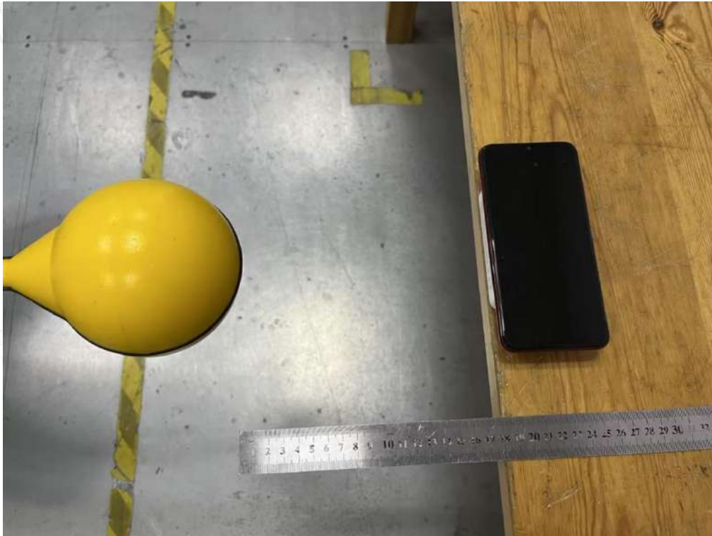
Test Position B(18cm) - Exposure photo from side edge surface-Rear(TM1)
