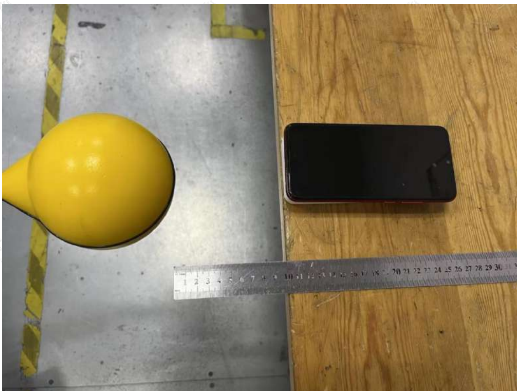
Test Position E(10cm) - Exposure photo from side edge surface-Right(TM1)
