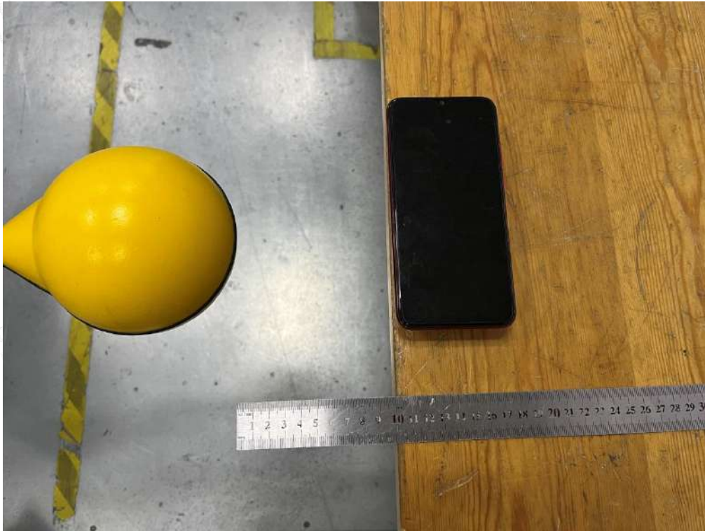
Test Position B(10cm) - Exposure photo from side edge surface-Rear(TM1)
