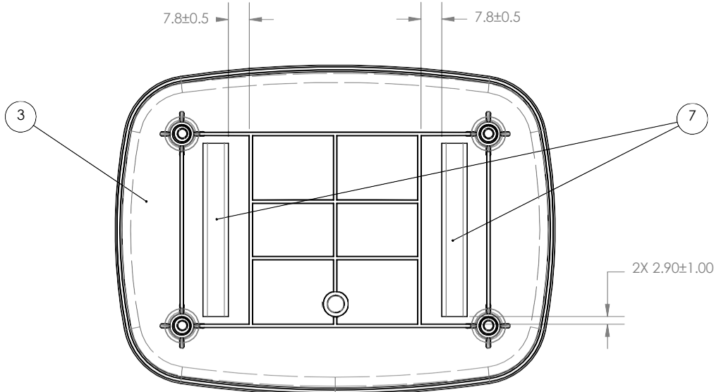
INSIDE OF TOP COVER
