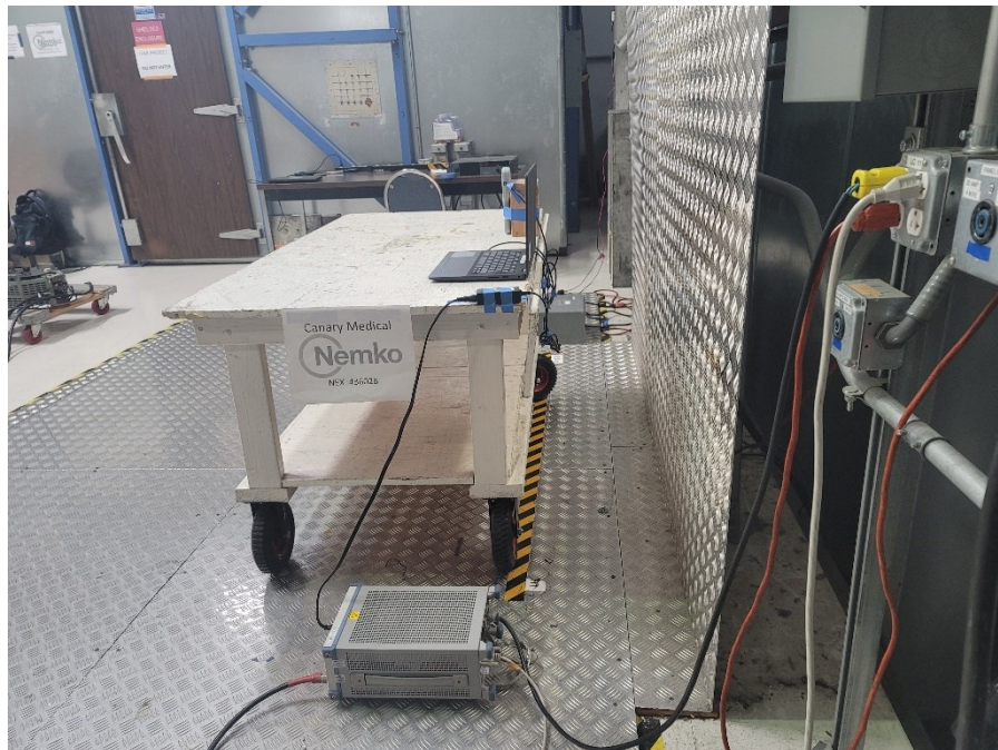
Figure 11 – Test setup, side view.
