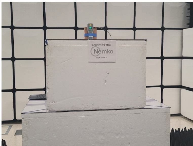
Figure 1 – Test setup
