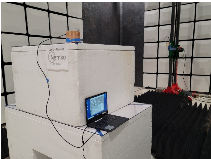
Figure 7 - Radiated emissions above 1 GHz (18 – 26 GHz).
