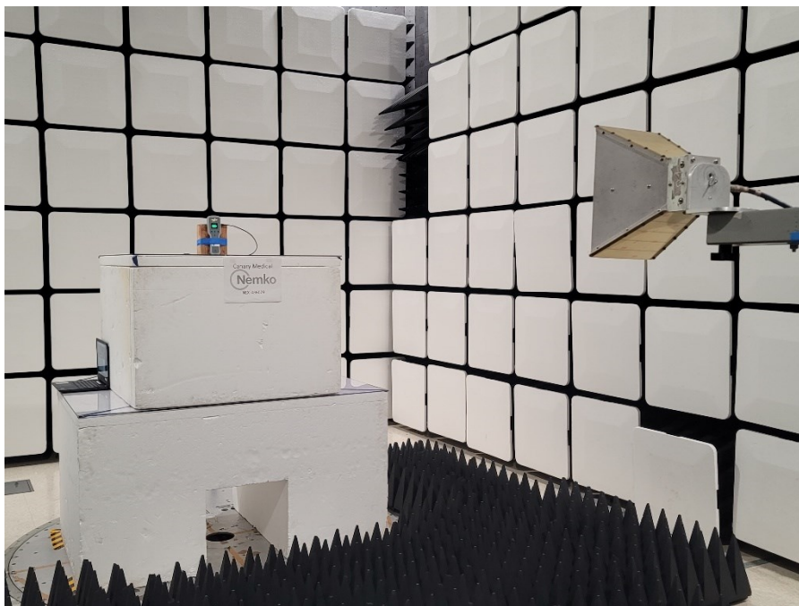
Figure 8- EIRP Measurement setup, front view.
