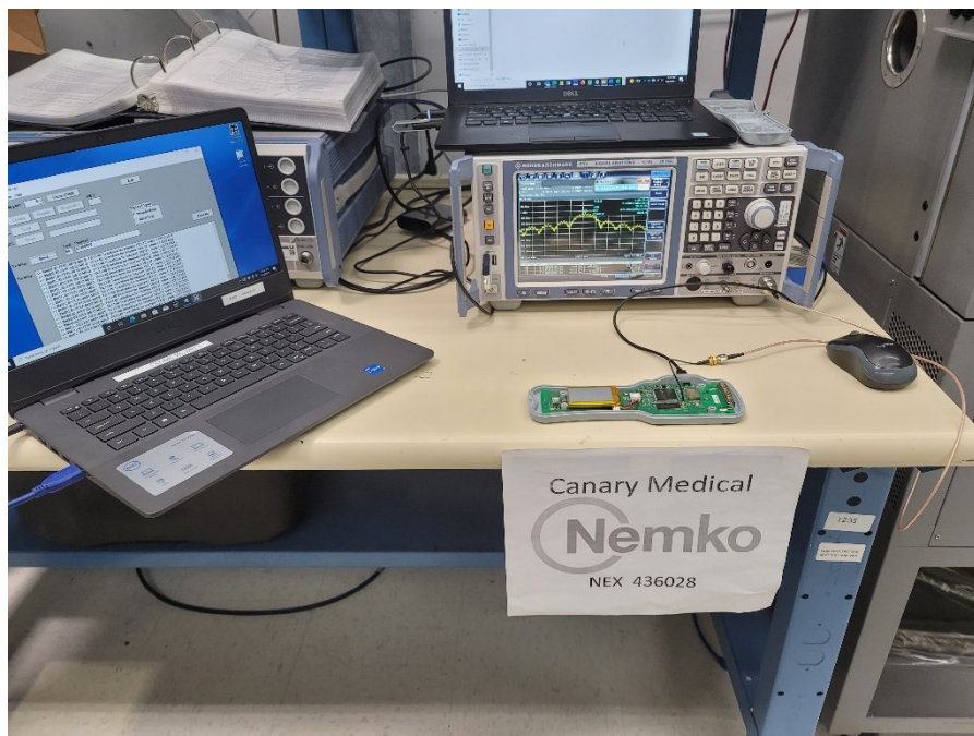
Figure 12 – Test setup, antenna conducted port.
