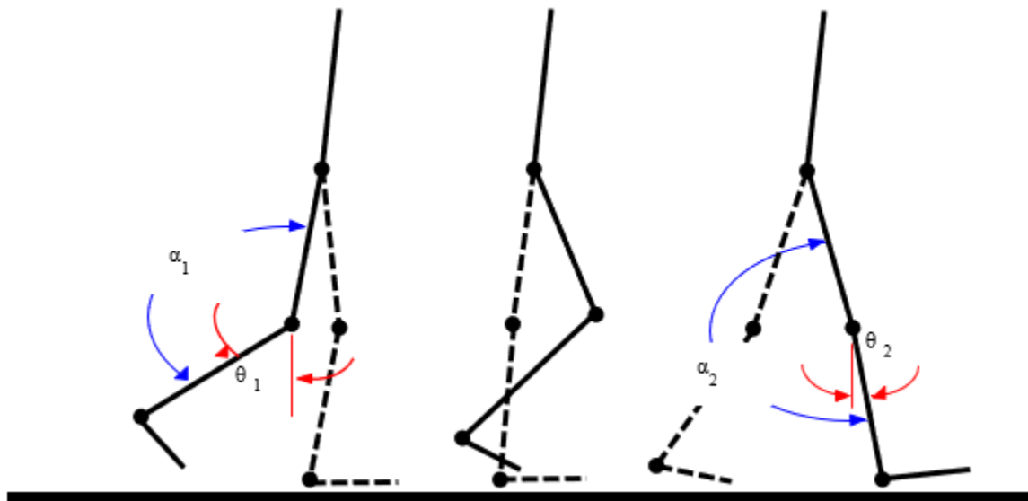
Figure 56: Schematic of Right Leg Motion. Tibia ROM = \theta_1 + \theta_2 and Knee ROM = \alpha_2 - \alpha_1
