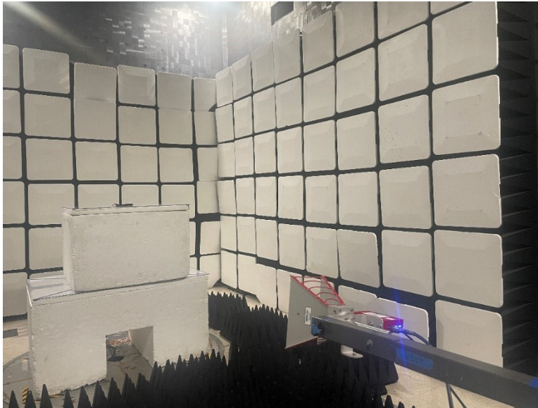
Figure 1.2-1: Radiated emissions setup (1 – 18 GHz): Front view photo.
