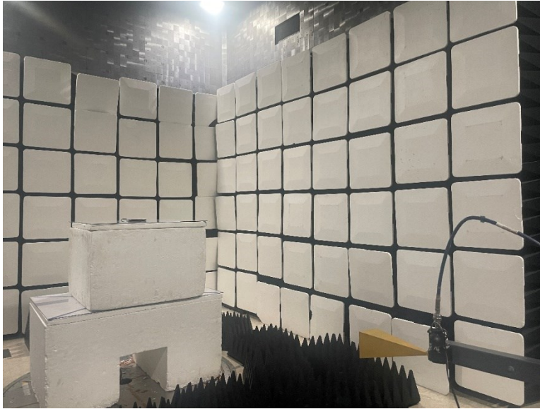
Figure 1.2-3: Radiated emissions setup (18 – 26.5 GHz): Front view photo.
