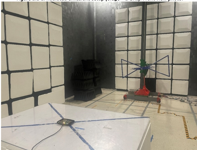
Figure 1.1-2: Radiated emissions setup (0.030 – 1 GHz): Rear view photo.
