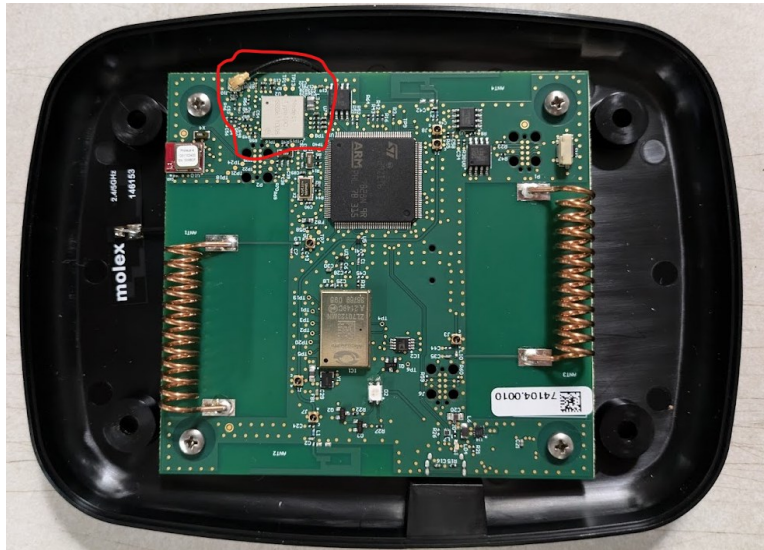
Figure 1.3-1: Wireless module (circled in red) in test jig
