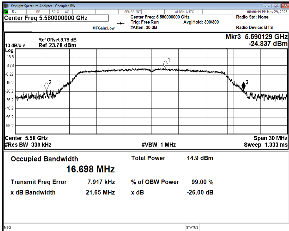
-26dB Bandwidth NVNT a 5580MHz Ant1
