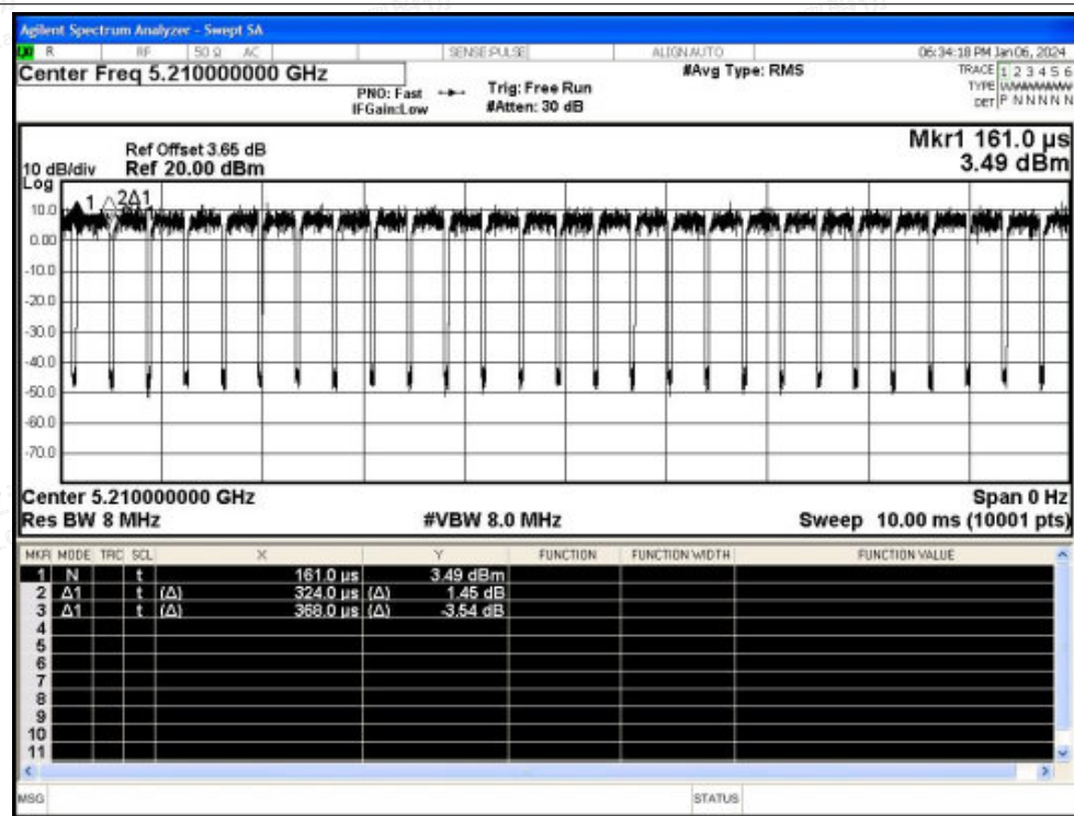
Duty Cycle NVNT ac80 5210MHz Ant3
