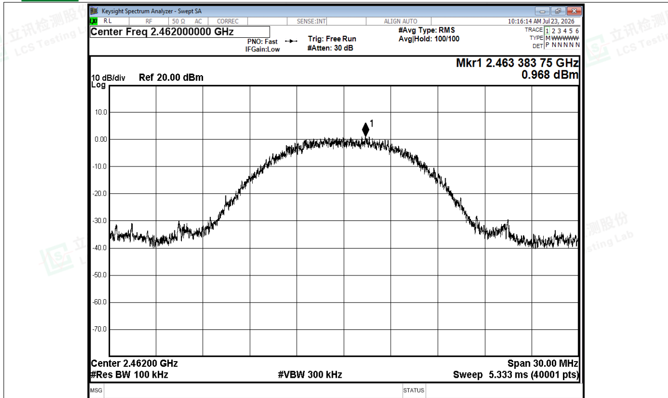
Tx. Spurious NVNT b 2462MHz Ant1 Ref
