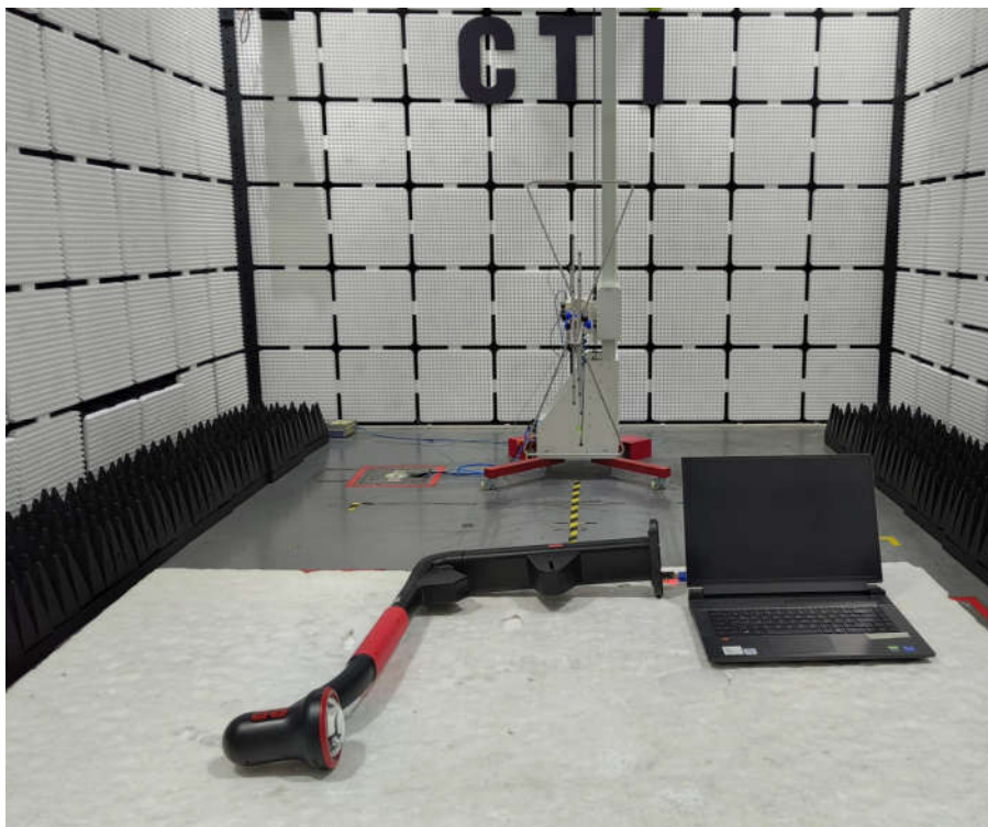
Radiated spurious emission Test Setup-1(Below 1GHz)
