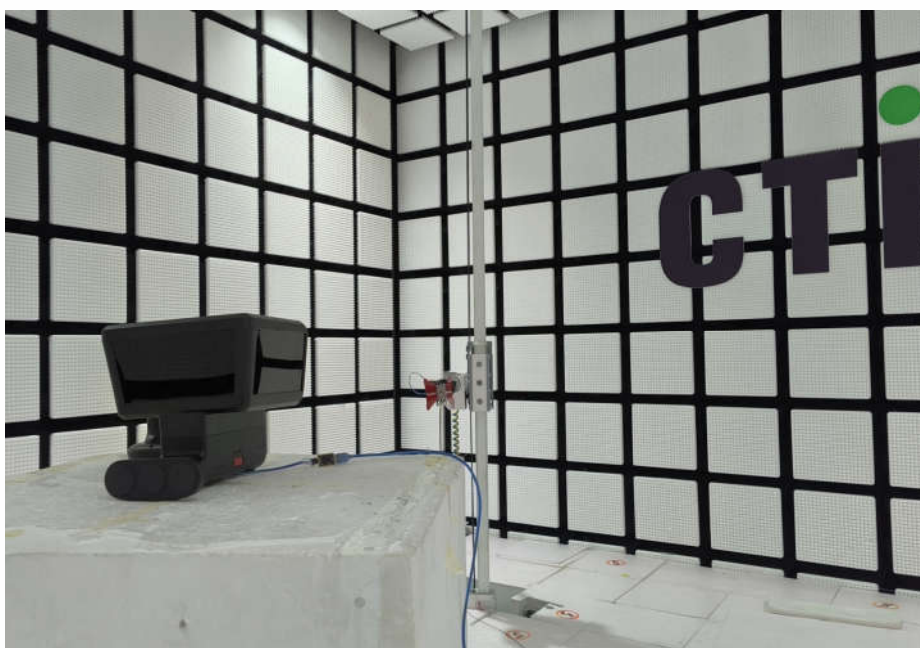
Radiated spurious emission Test Setup-4(Above 1GHz)
