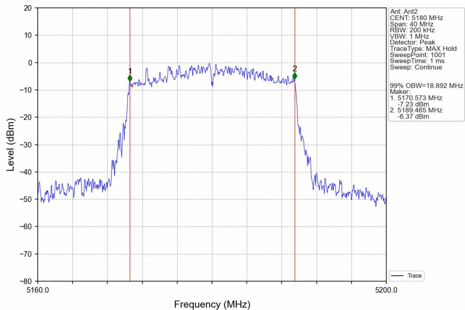
802.11ax(HEW20)_LCH_5180MHz_SU_ / _Ant2_NTNV
