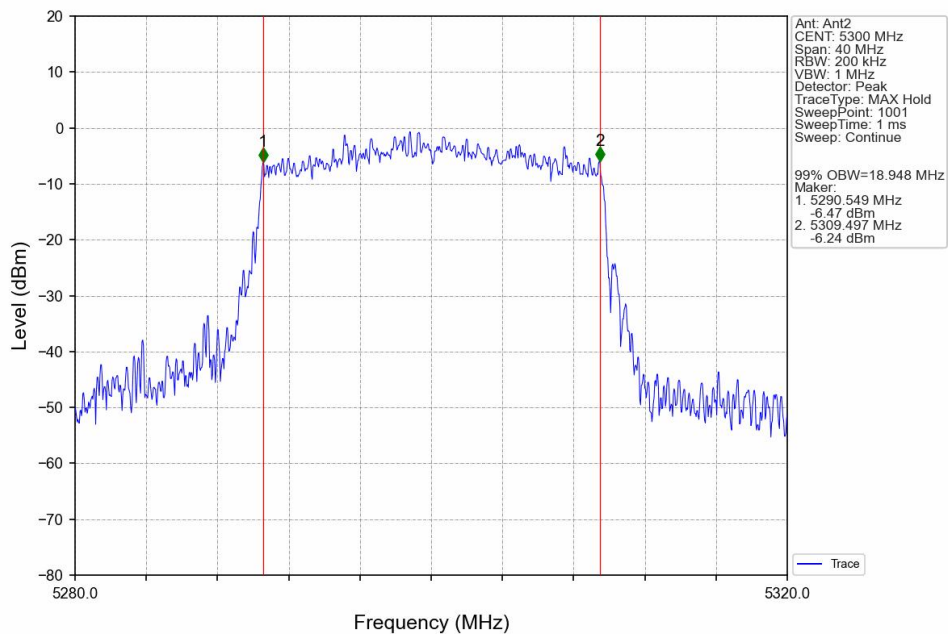
802.11ax(HEW20)_MCH_5300MHz_SU_/_Ant2_NTNV
