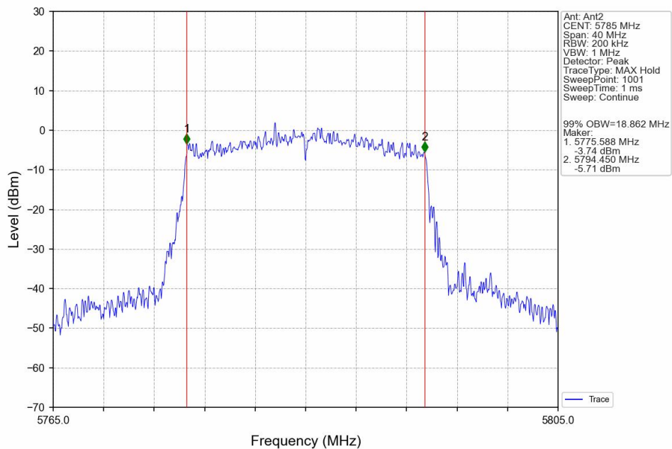
802.11ax(HEW20)_MCH_5785MHz_SU_ / _Ant2_NTNV
