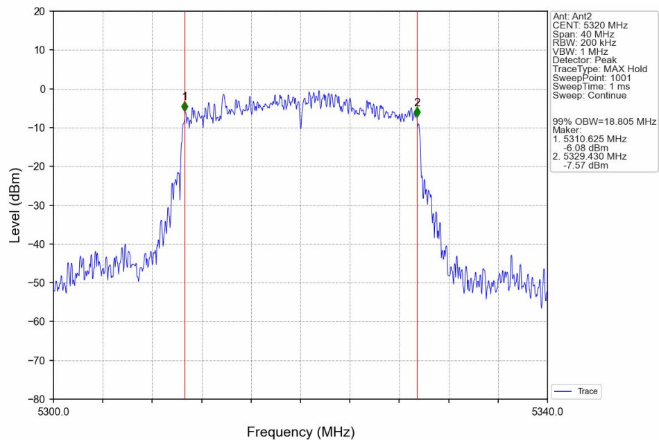
802.11ax(HEW20)_HCH_5320MHz_SU_ / _Ant2_NTNV
