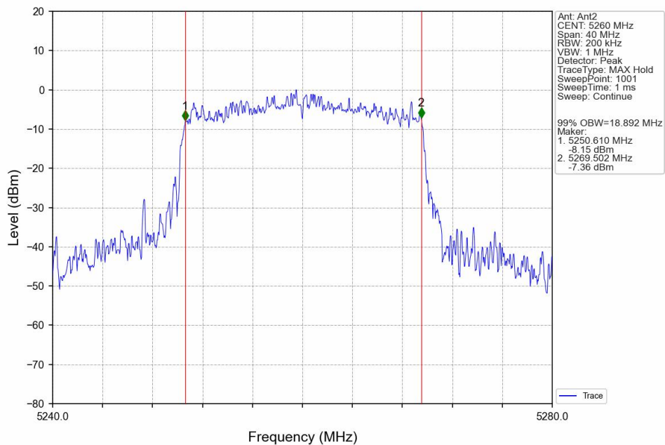
802.11ax(HEW20)_LCH_5260MHz_SU_/_Ant2_NTNV
