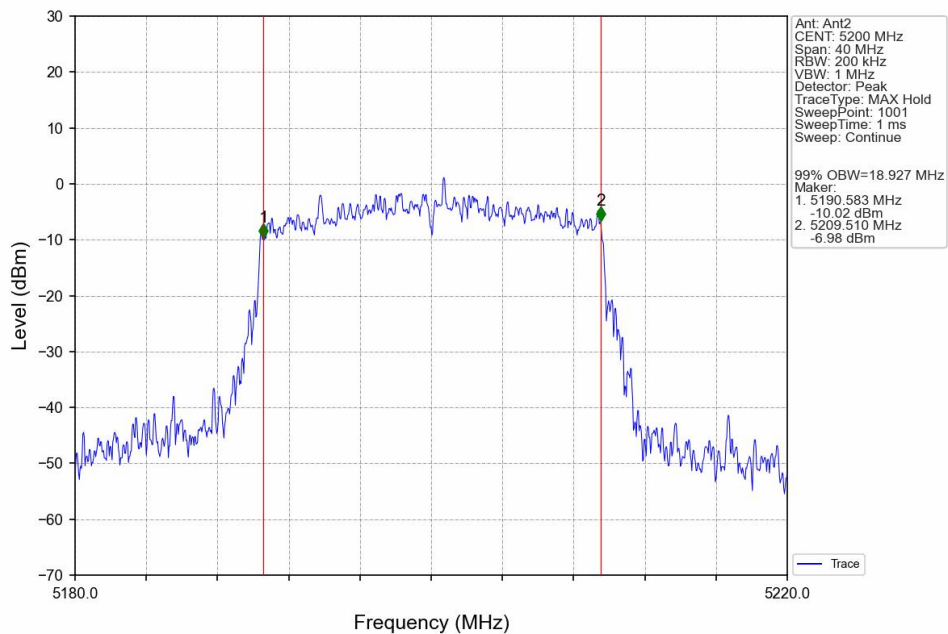
802.11ax(HEW20)_MCH_5200MHz_SU_ / _Ant2_NTNV
