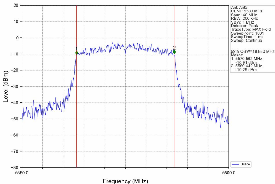
802.11ax(HEW20)_MCH_5580MHz_SU_/_Ant2_NTNV
