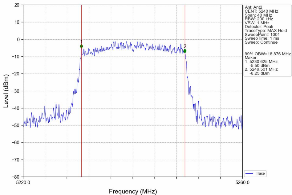
802.11ax(HEW20)_HCH_5240MHz_SU_/_Ant2_NTNV
