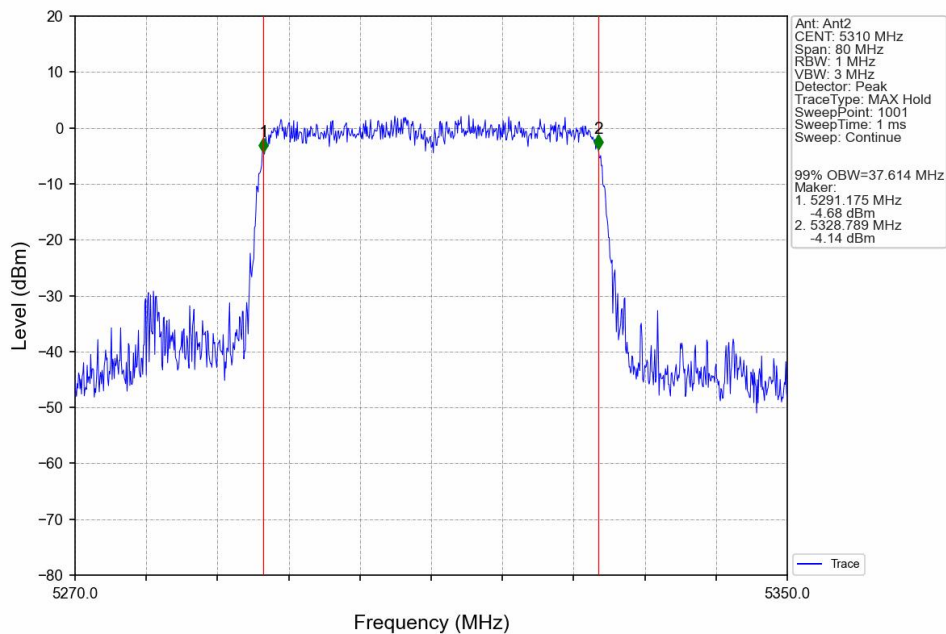
802.11ax(HEW40)_HCH_5310MHz_SU_/_Ant2_NTNV
