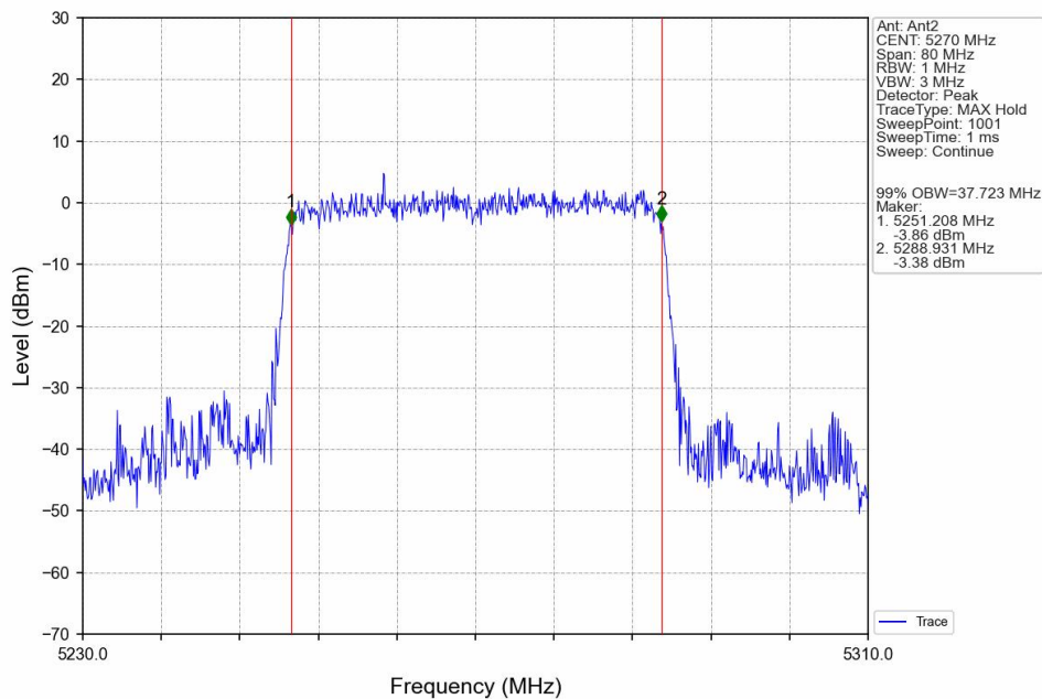
802.11ax(HEW40)_LCH_5270MHz_SU_/_Ant2_NTNV
