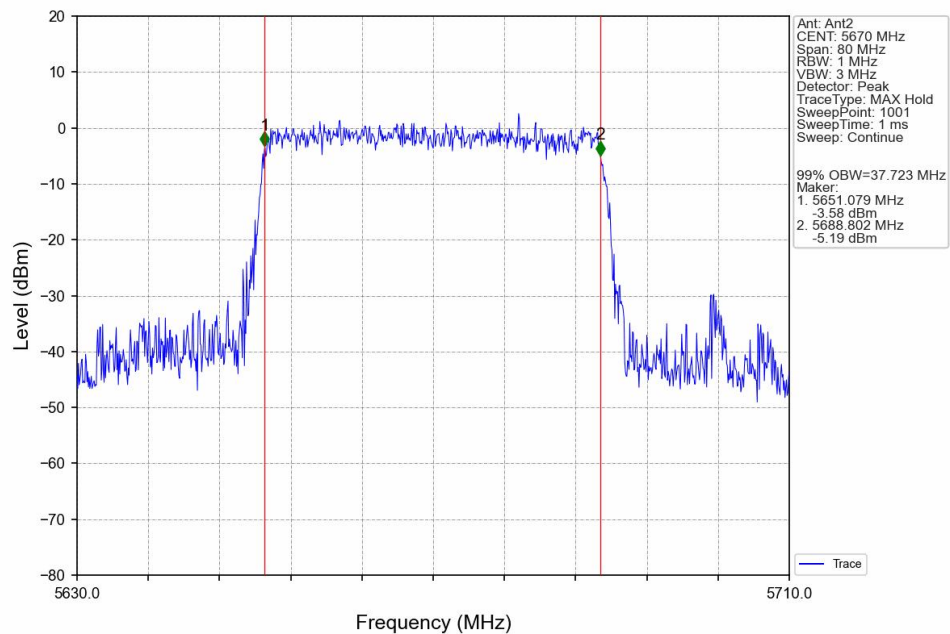
802.11ax(HEW40)_HCH_5670MHz_SU_/_Ant2_NTNV
