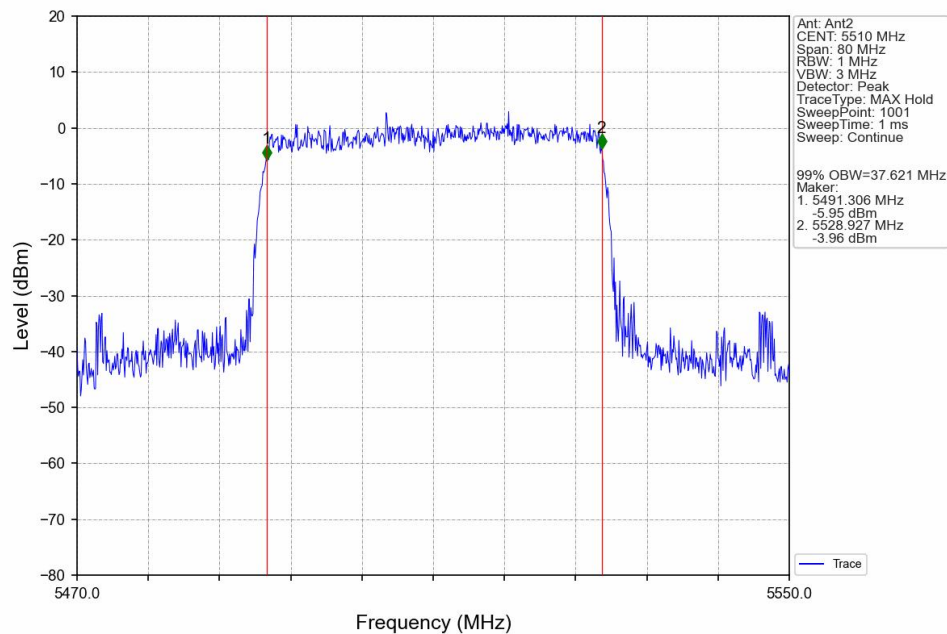
802.11ax(HEW40)_LCH_5510MHz_SU_/_Ant2_NTNV
