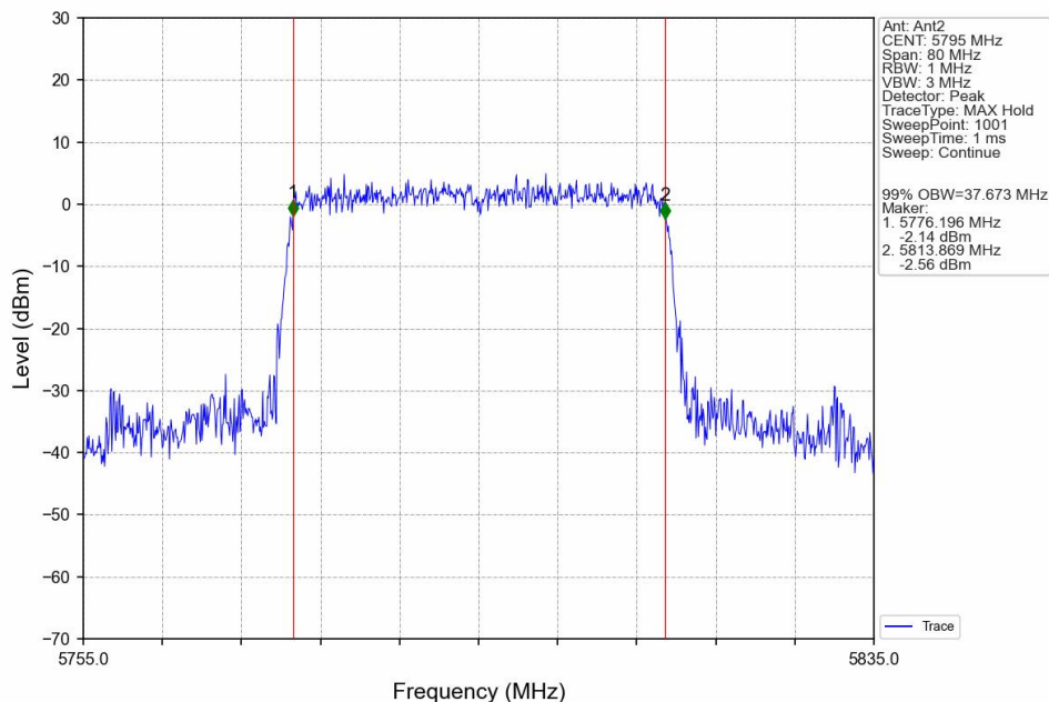
802.11ax(HEW40)_HCH_5795MHz_SU_/_Ant2_NTNV
