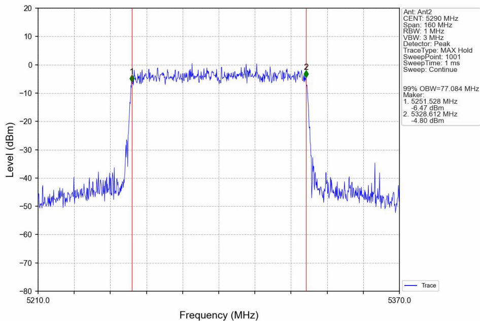
802.11ax(HEW80)_MCH_5290MHz_SU_/_Ant2_NTNV
