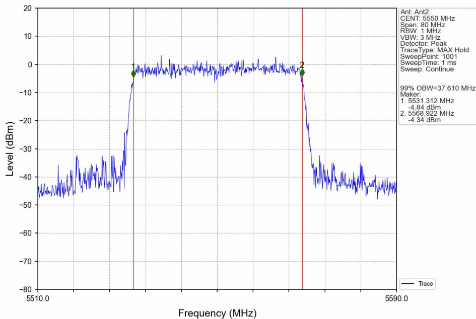
802.11ax(HEW40)_MCH_5550MHz_SU_/_Ant2_NTNV
