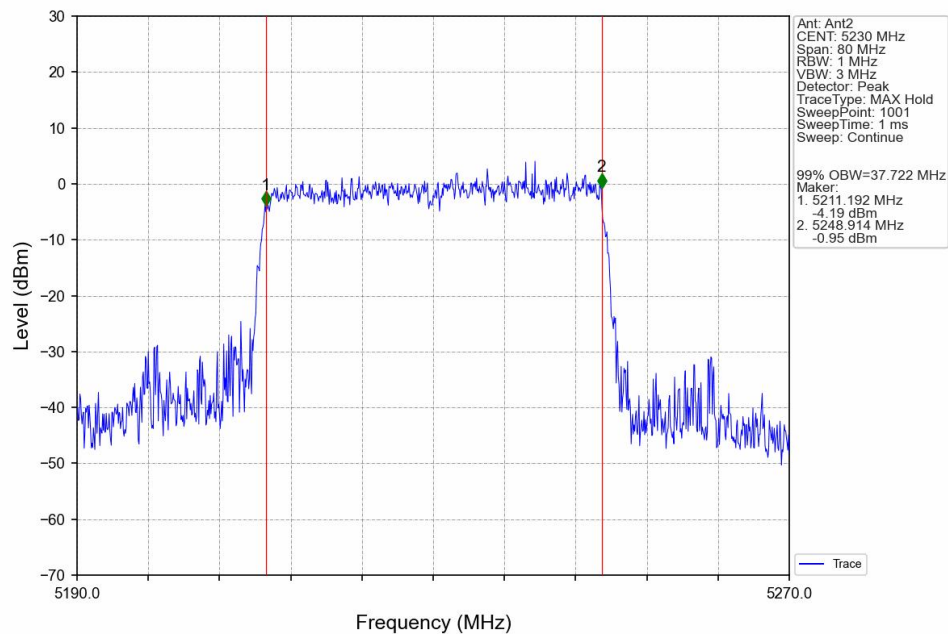
802.11ax(HEW40)_HCH_5230MHz_SU_ / _Ant2_NTNV
