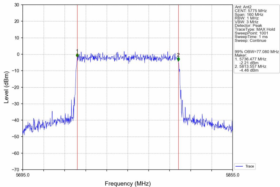
802.11ax(HEW80)_MCH_5775MHz_SU_ / _Ant2_NTNV
