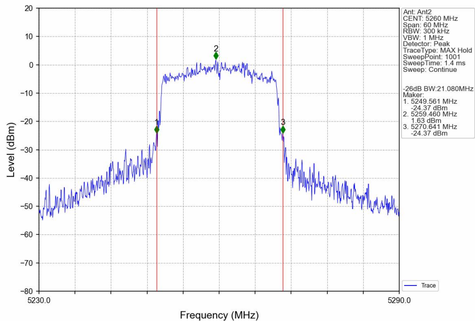
802.11ax(HEW20)_LCH_5260MHz_SU_/_Ant2_NTNV
