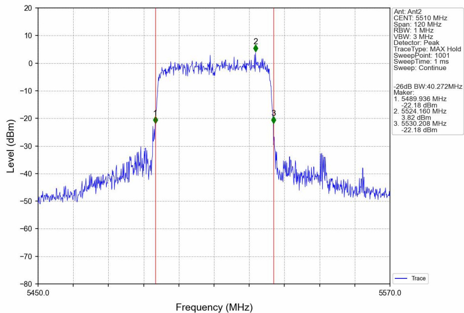
802.11ax(HEW40)_LCH_5510MHz_SU_/_Ant2_NTNV
