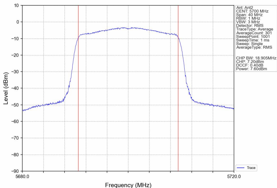
802.11ax(HEW20)_HCH_5700MHz_SU_/_Ant2_NTNV
