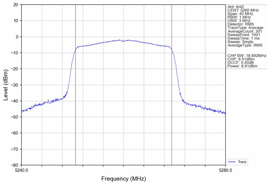
802.11ax(HEW20)_LCH_5260MHz_SU_/_Ant2_NTNV
