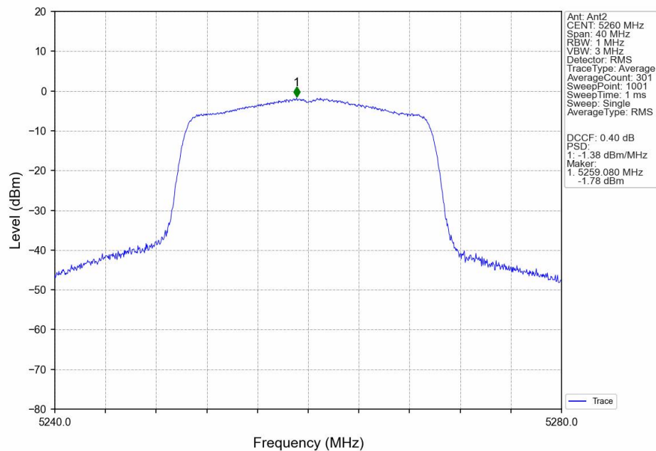
802.11ax(HEW20)_LCH_5260MHz_SU_/_Ant2_NTNV
