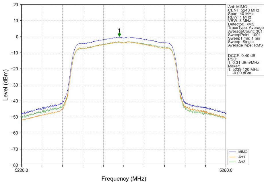
802.11ax(HEW20)_HCH_5240MHz_SU_/_MIMO_NTNV
