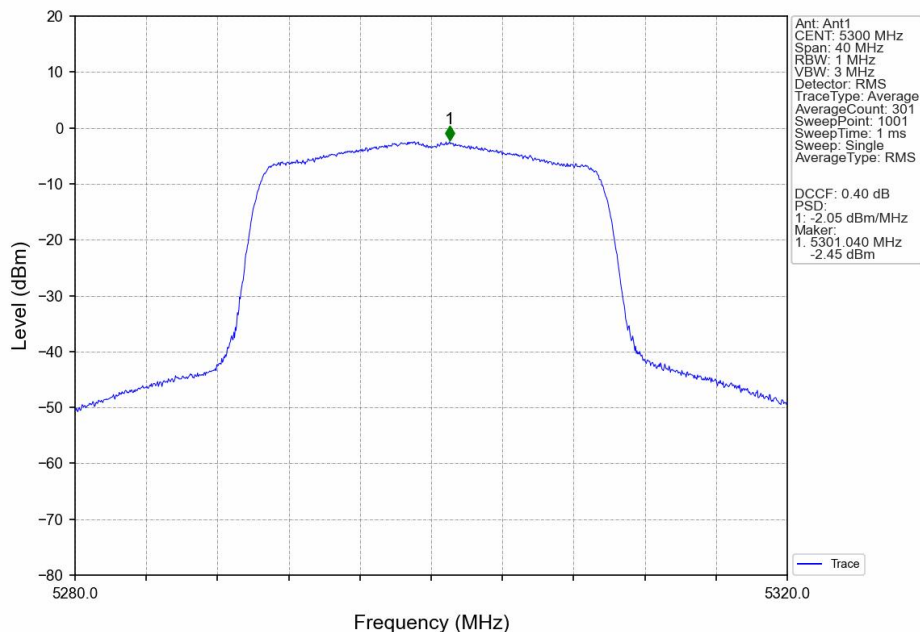
802.11ax(HEW20)_MCH_5300MHz_SU / Ant1_NTNV
