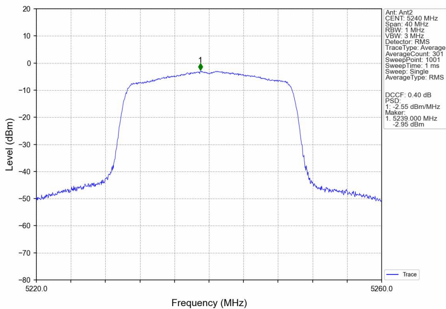
802.11ax(HEW20)_HCH_5240MHz_SU_/_MIMO_NTNV
