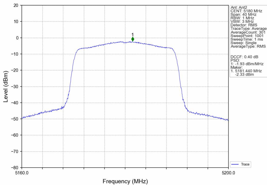
802.11ax(HEW20)_LCH_5180MHz_SU_/_MIMO_NTNV
