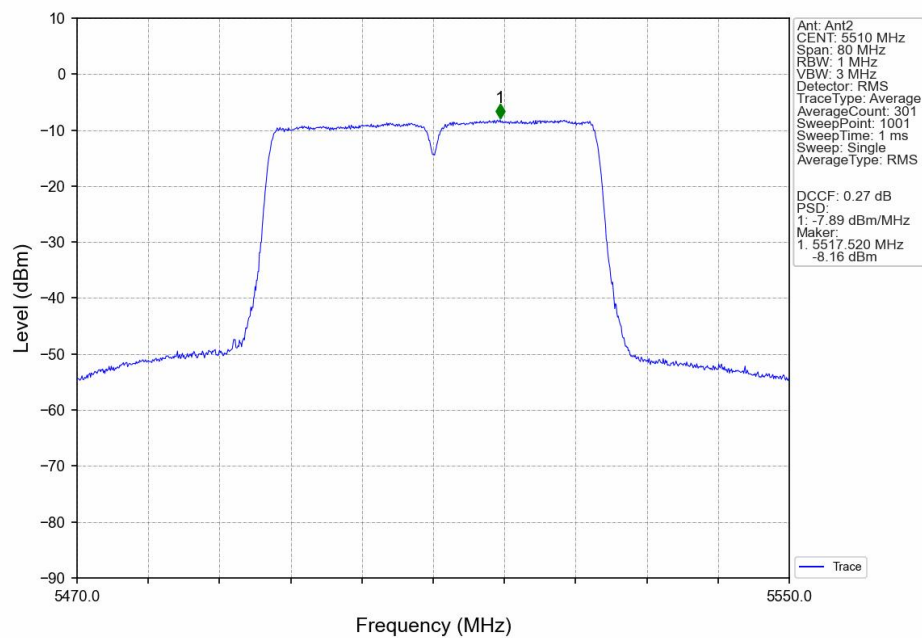
802.11ac(VHT40)_LCH_5510MHz_MIMO_NTNV
