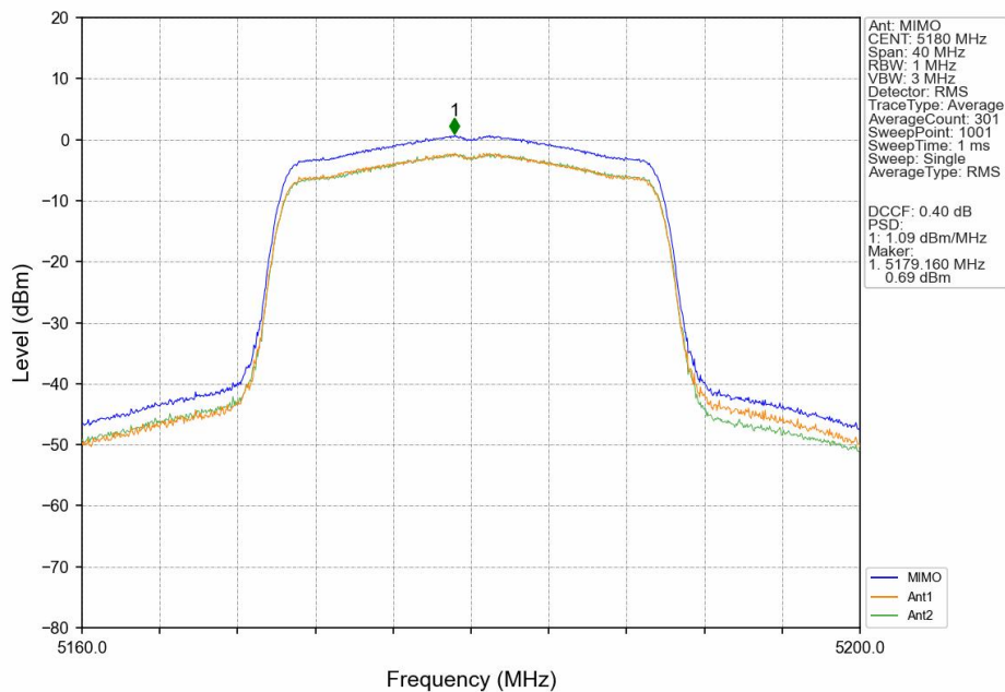
802.11ax(HEW20)_LCH_5180MHz_SU_/_MIMO_NTNV
