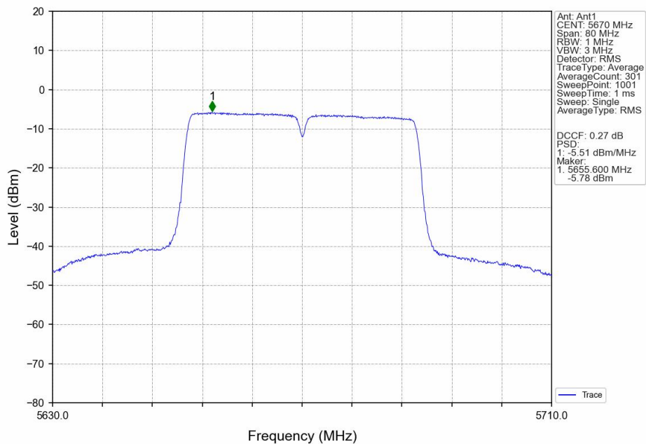
802.11ac(VHT40)_HCH_5670MHz_Ant1_NTNV
