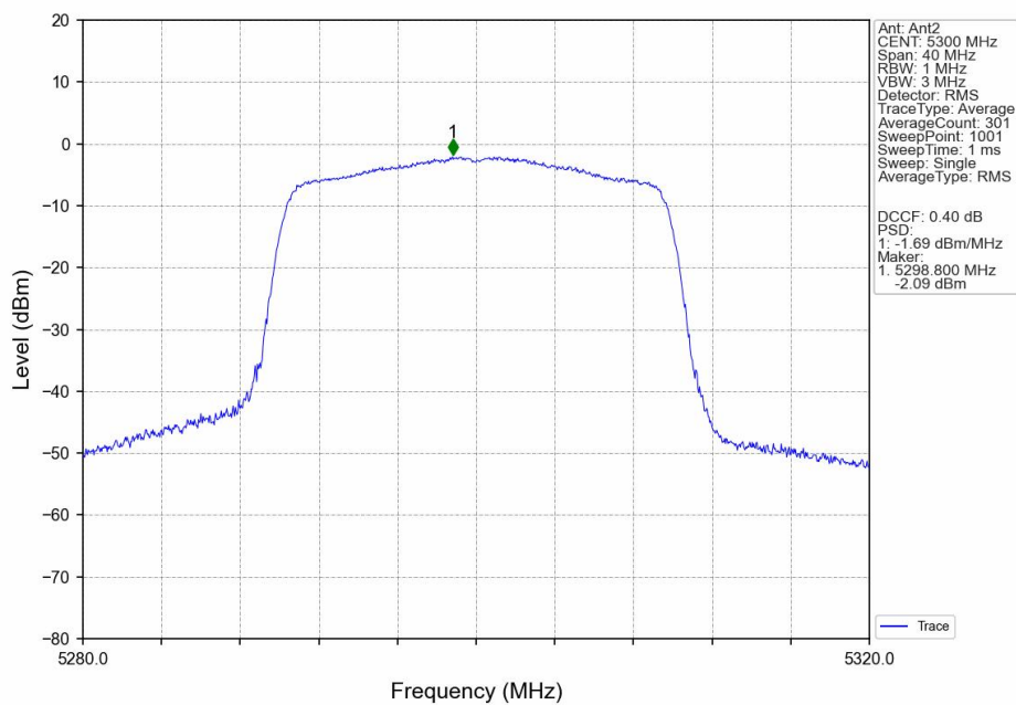
802.11ax(HEW20)_MCH_5300MHz_SU_/_MIMO_NTNV
