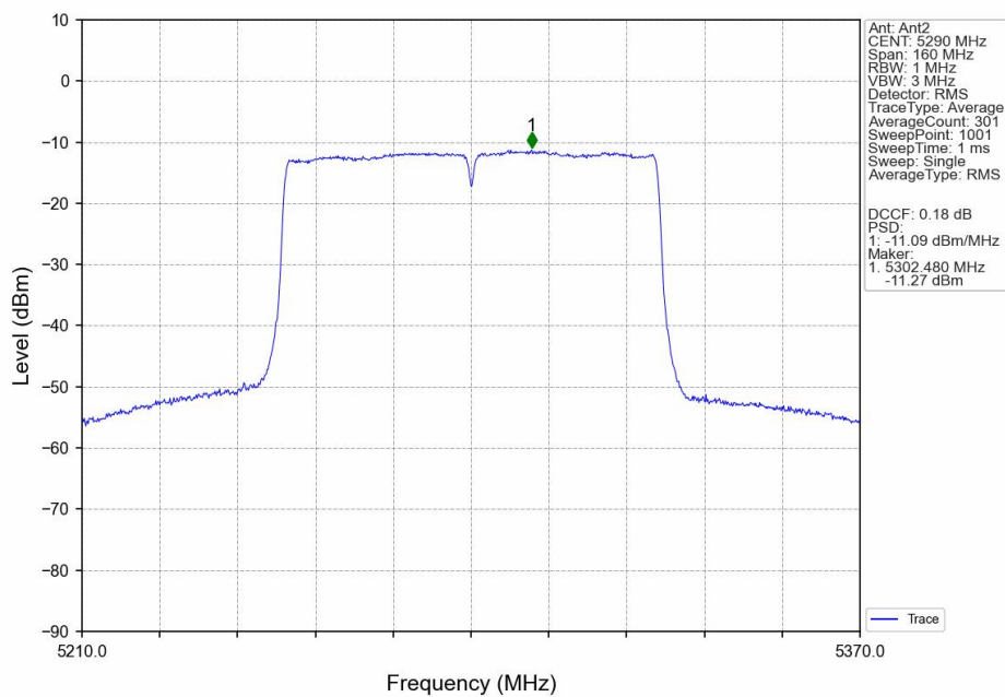
802.11ac(VHT80)_MCH_5290MHz_MIMO_NTNV
