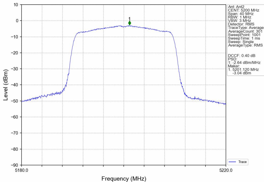
802.11ax(HEW20)_MCH_5200MHz_SU_ / Ant2_NTNV
