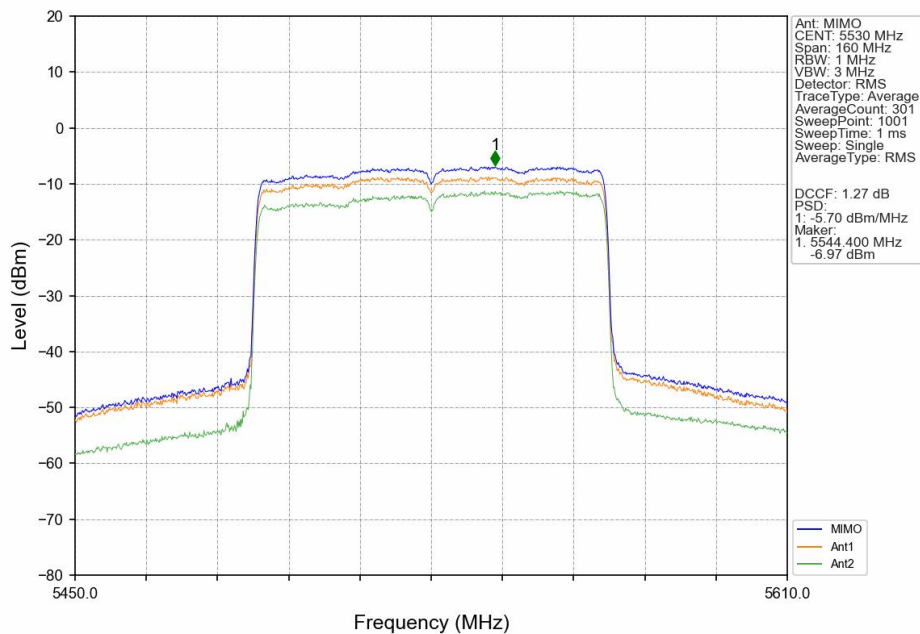
802.11ax(HEW80)_LCH_5530MHz_SU_/_MIMO_NTNV
