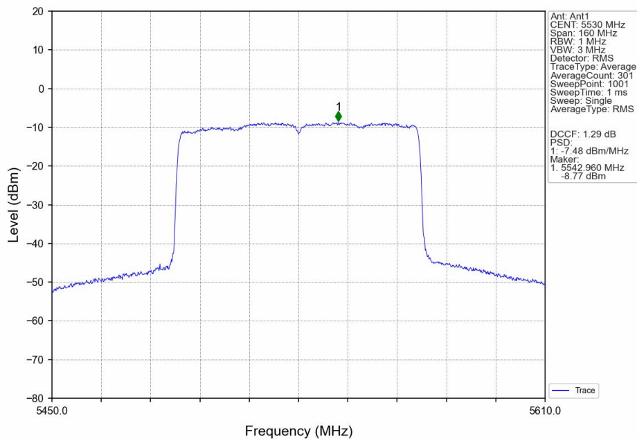
802.11ax(HEW80)_LCH_5530MHz_SU_/_Ant1_NTNV
