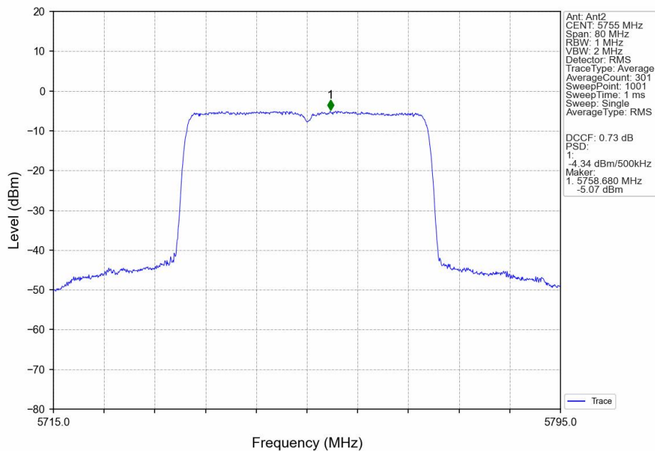
802.11ax(HEW40)_LCH_5755MHz_SU_/_Ant2_NTNV
