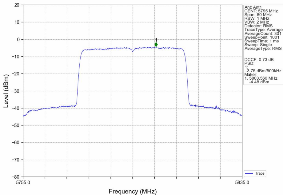
802.11ax(HEW40)_HCH_5795MHz_SU / Ant1_NTNV
