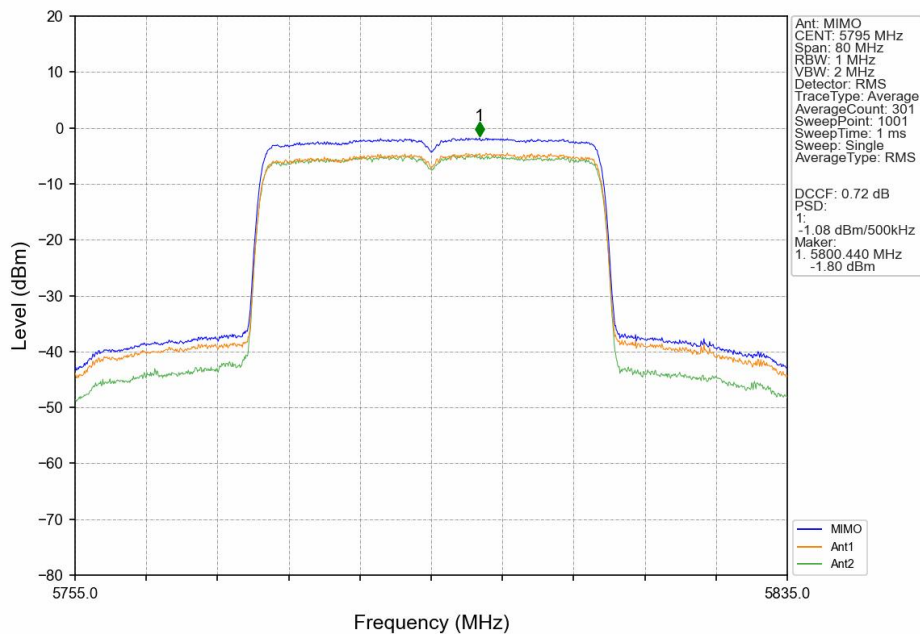
802.11ax(HEW40)_HCH_5795MHz_SU_/_MIMO_NTNV
