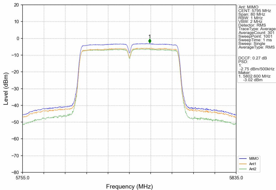
802.11ac(VHT40)_HCH_5795MHz_MIMO_NTNV
