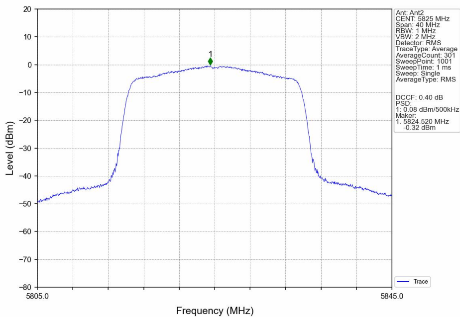
802.11ax(HEW20)_HCH_5825MHz_SU_/_MIMO_NTNV
