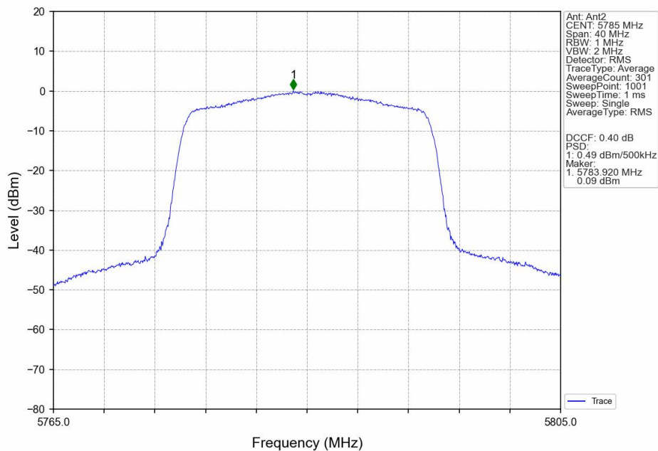
802.11ax(HEW20)_MCH_5785MHz_SU_/_Ant2_NTNV
