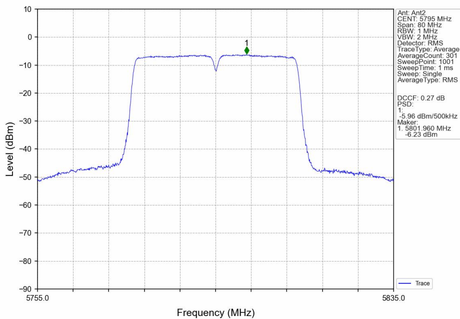
802.11ac(VHT40)_HCH_5795MHz_MIMO_NTNV
