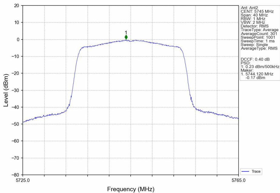
802.11ax(HEW20)_LCH_5745MHz_SU_/_MIMO_NTNV
