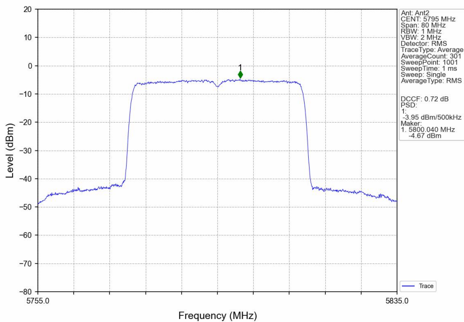
802.11ax(HEW40)_HCH_5795MHz_SU_/_MIMO_NTNV
