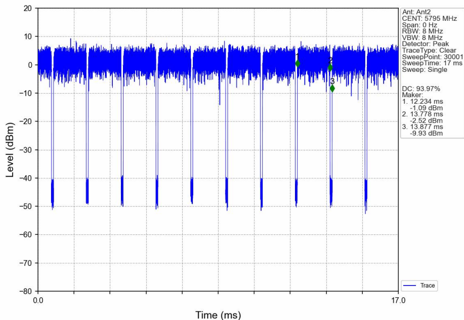
802.11ac(VHT40)_HCH_5795MHz_Ant2_NTNV
