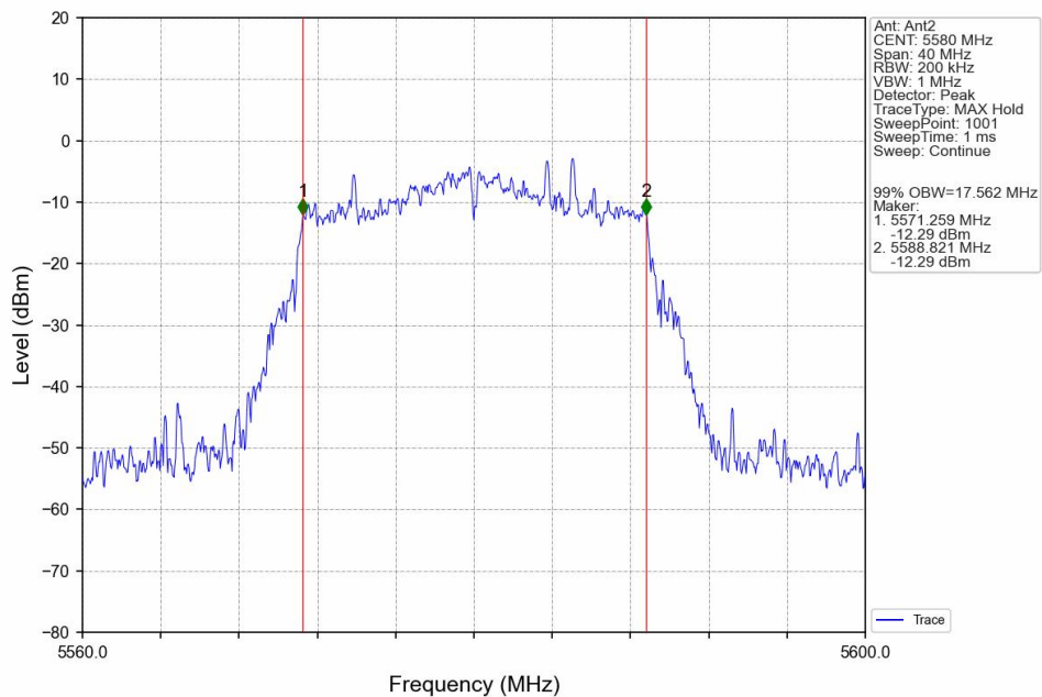
802.11n(HT20)_MCH_5580MHz_Ant2_NTNV
