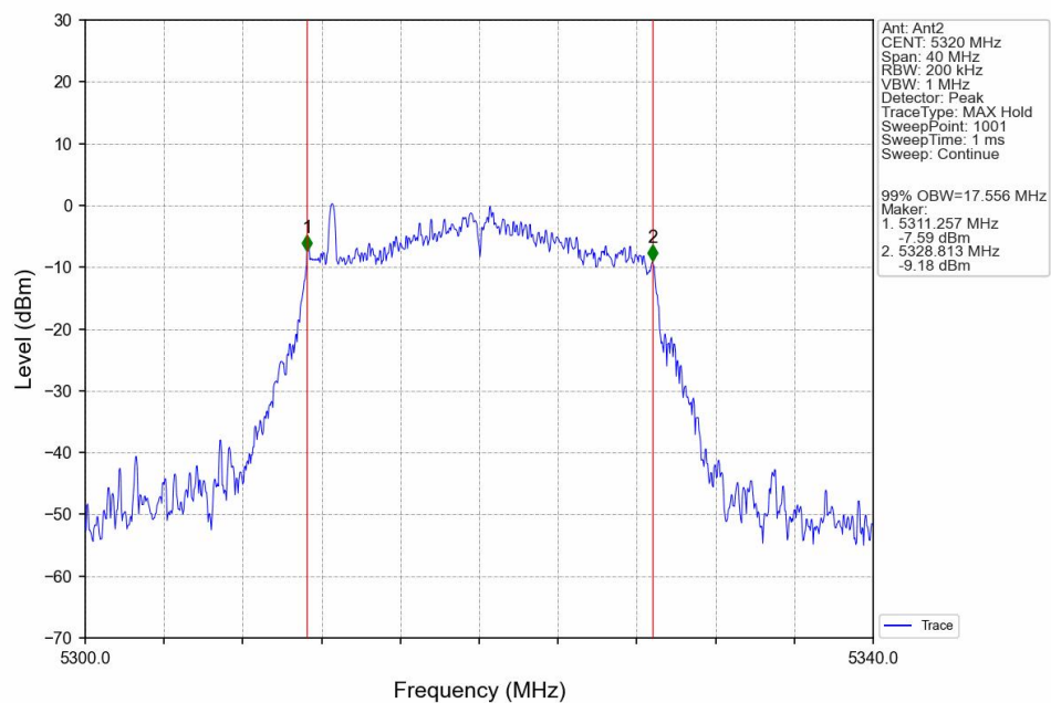
802.11ac(VHT20)_HCH_5320MHz_Ant2_NTNV
