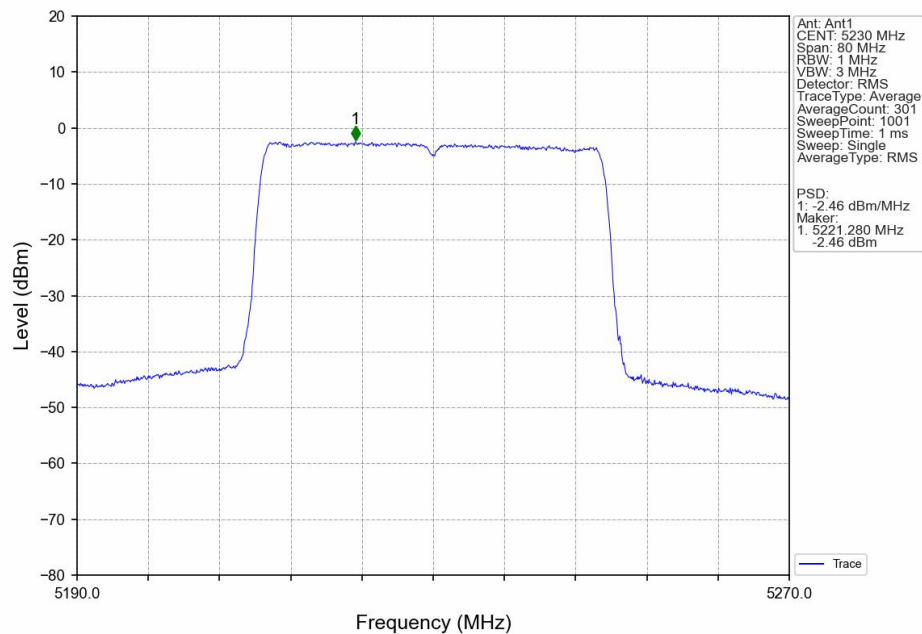
802.11ax(HEW40)_HCH_5230MHz_SU_ / Ant1_NTNV
