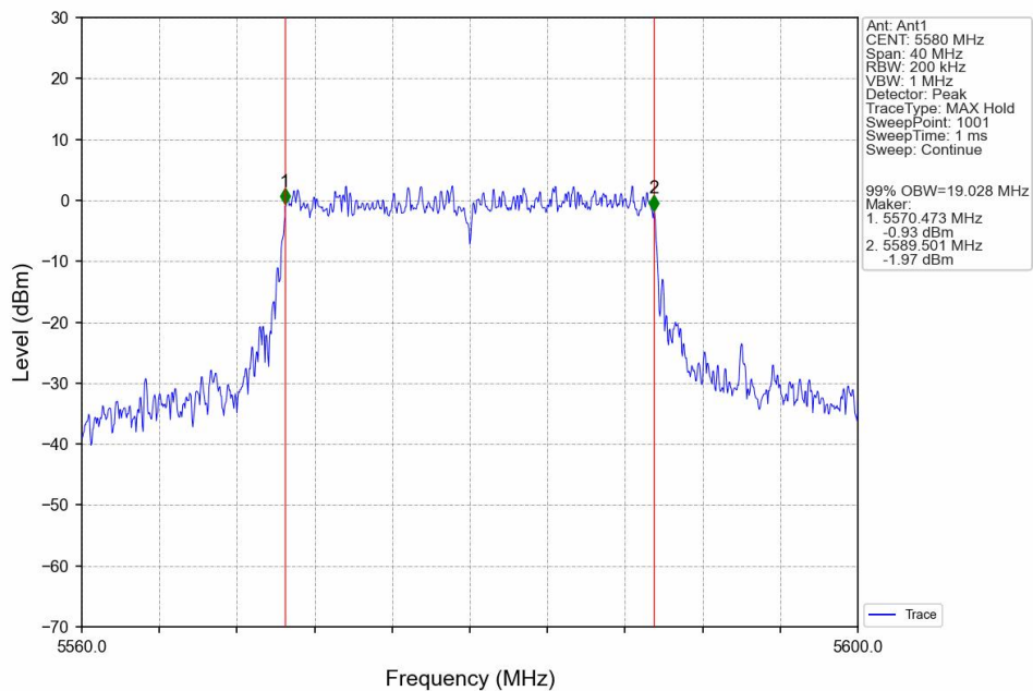
802.11ax(HEW20)_MCH_5580MHz_SU_ / _Ant1_NTNV
