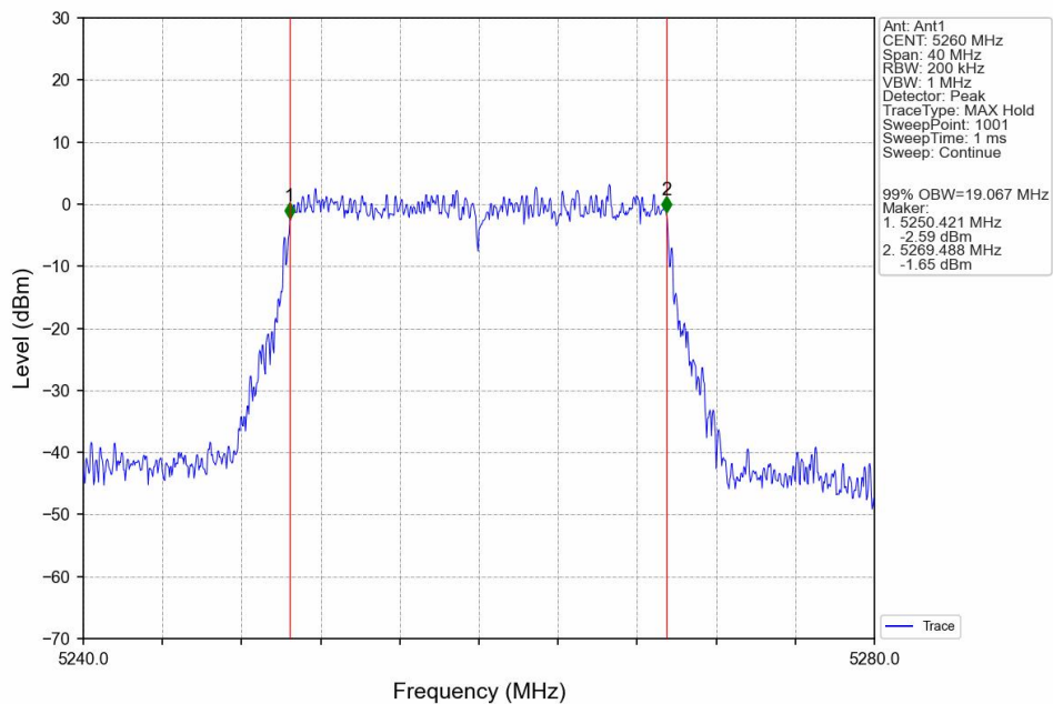
802.11ax(HEW20)_LCH_5260MHz_SU_/_Ant1_NTNV
