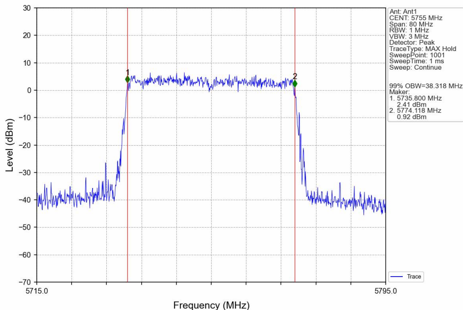
802.11ax(HEW40)_LCH_5755MHz_SU_/_Ant1_NTNV
