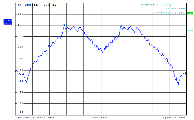
GFSK_Middle 1.000 MHz
