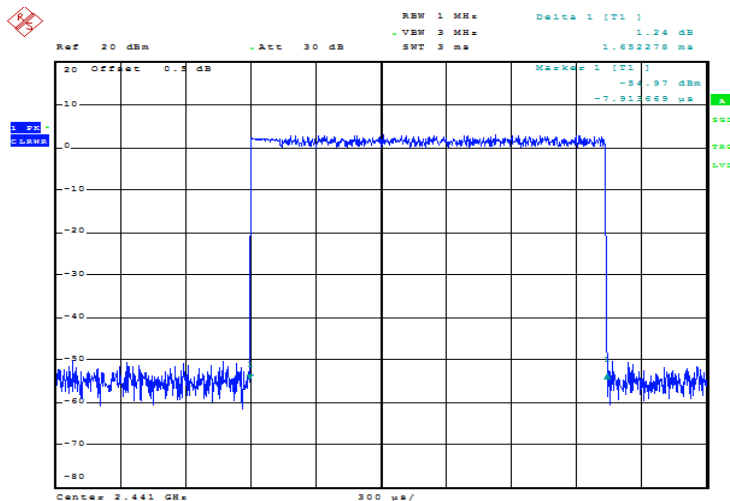
8DPSK_Hopping_3DH3 1.652ms
