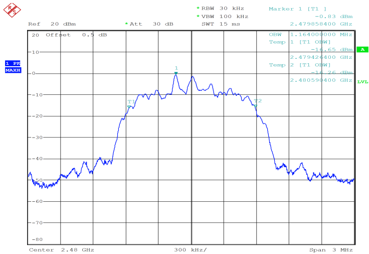
\pi/4 -DQPSK_High 1.164 MHz
