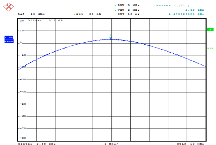
8DPSK_High 2.83 dBm
