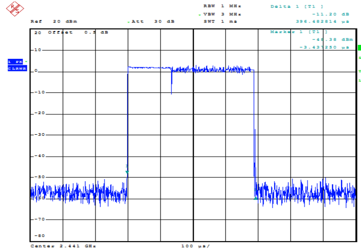
8DPSK_Hopping_3DH1 0.396ms
