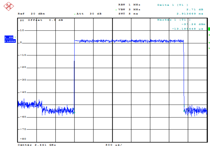
8DPSK_Hopping_3DH5 2.914ms
