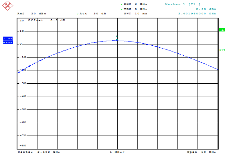
GFSK_Low 2.63 dBm
