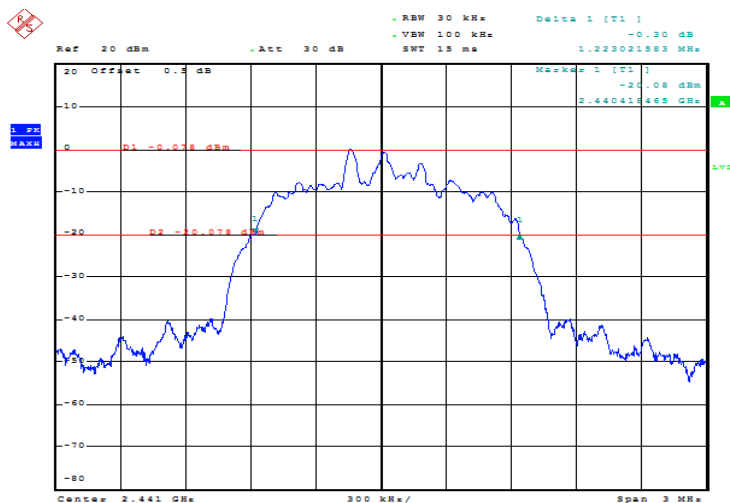
8DPSK_Middle 1.223 MHz
