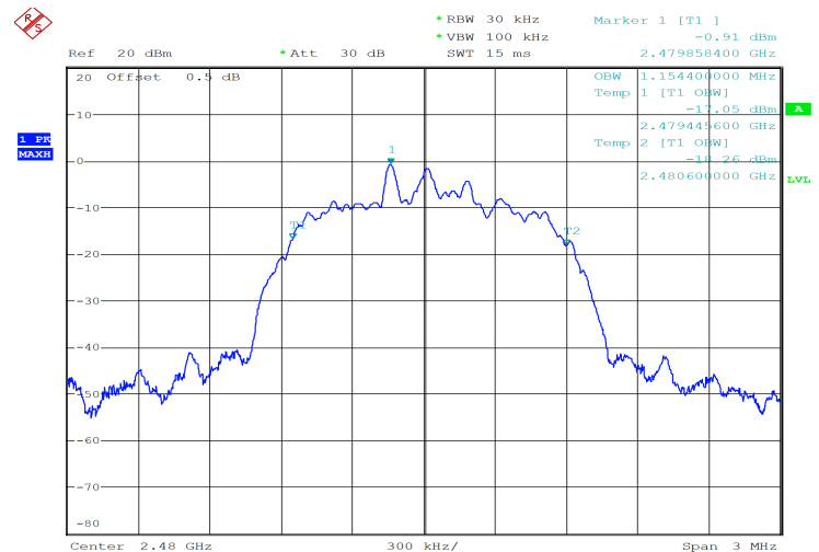
8DPSK_High 1.154 MHz
