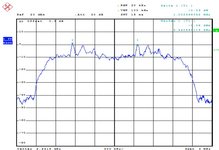
8DPSK_Middle 1.002 MHz
