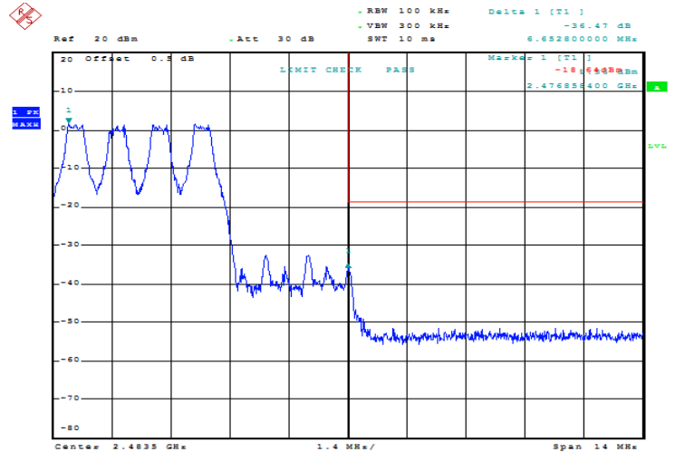
GFSK_Hopping_Upper 36.47 dB
