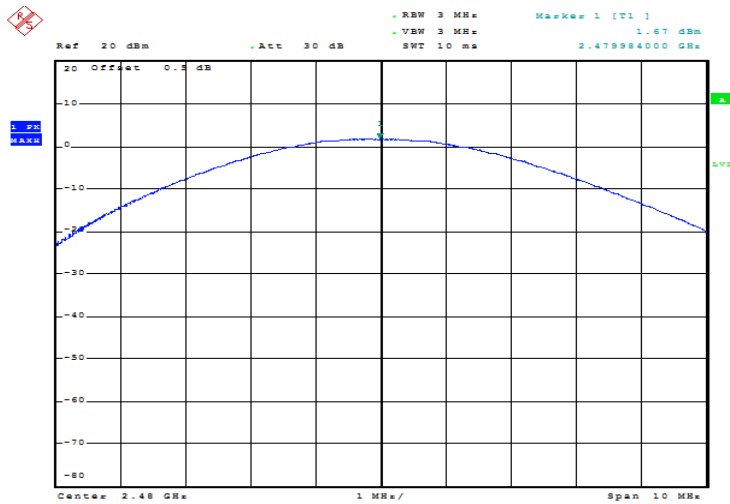
GFSK_High 1.67 dBm
