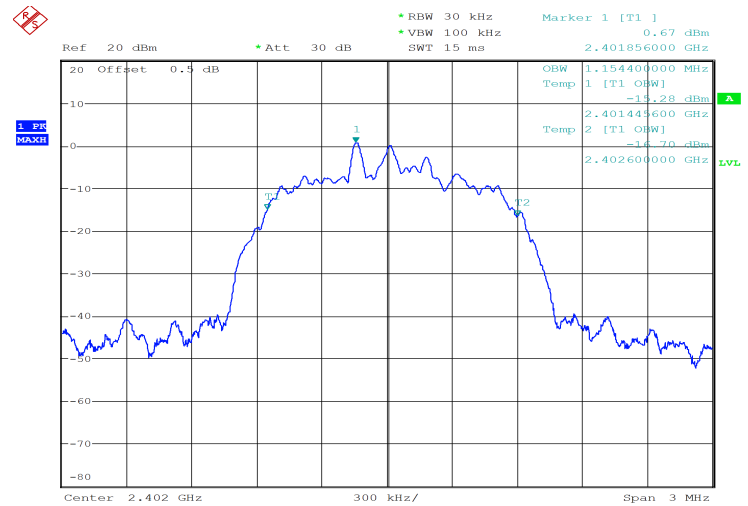
8DPSK_Low 1.154 MHz
