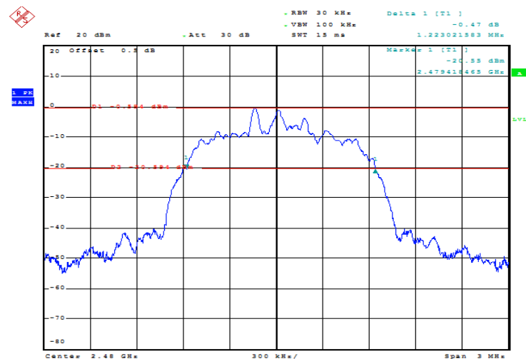
8DPSK_High 1.223 MHz
