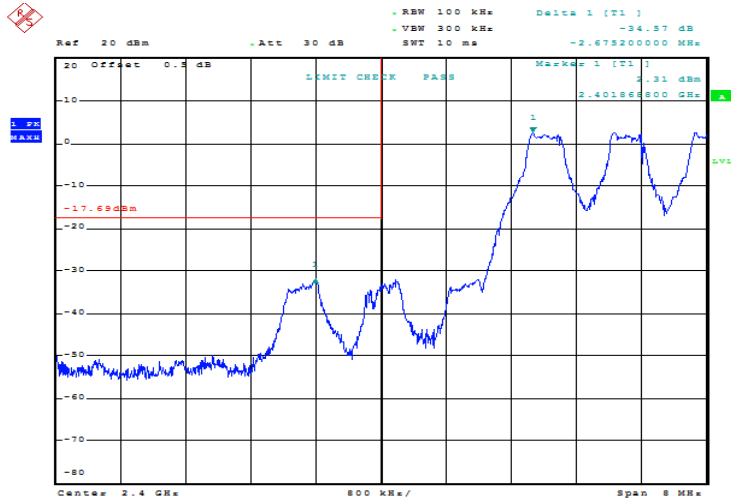
GFSK_Hopping_Lower 34.57 dB
