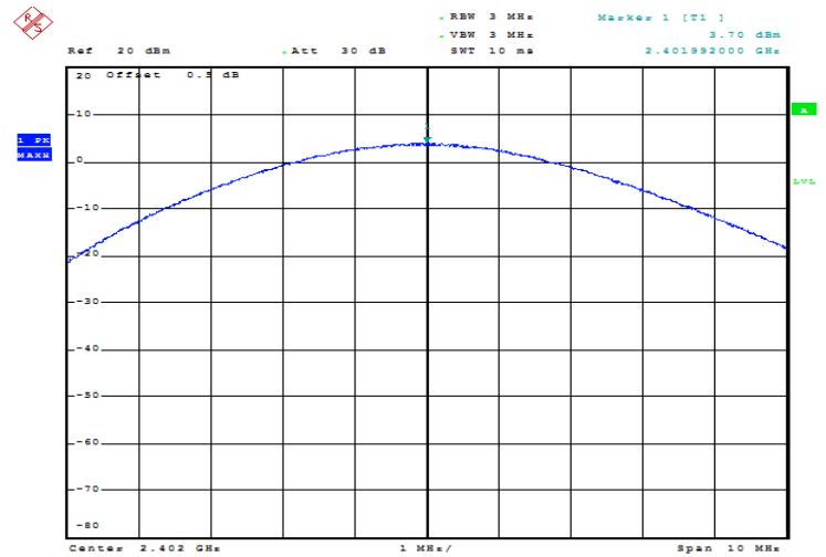
8DPSK_Low 3.70 dBm
