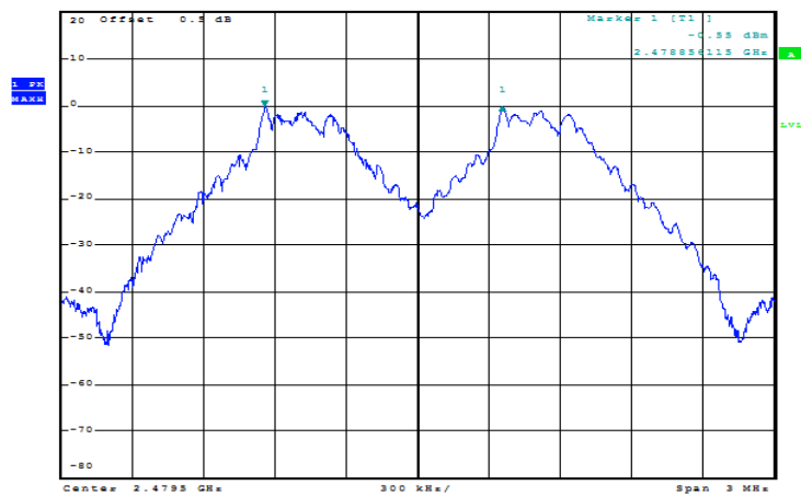
GFSK_High 1.002 MHz
