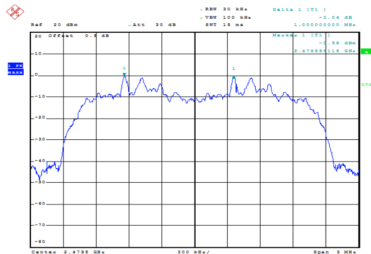
8DPSK_High 1.000 MHz
