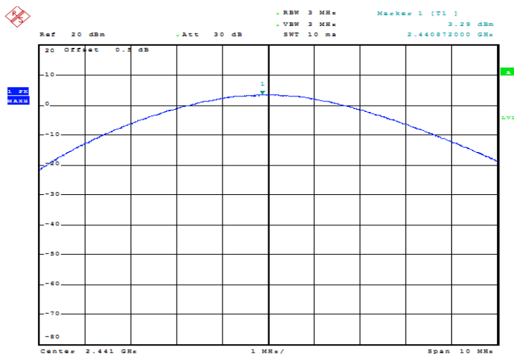
8DPSK_Middle 3.29 dBm
