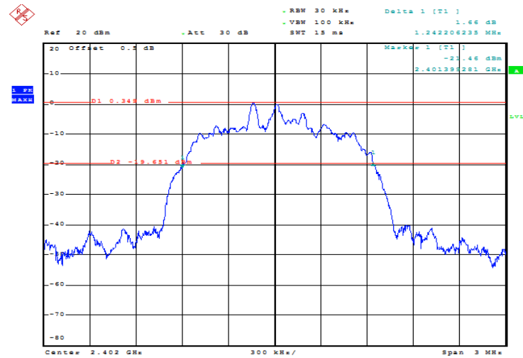
8DPSK_Low 1.242 MHz
