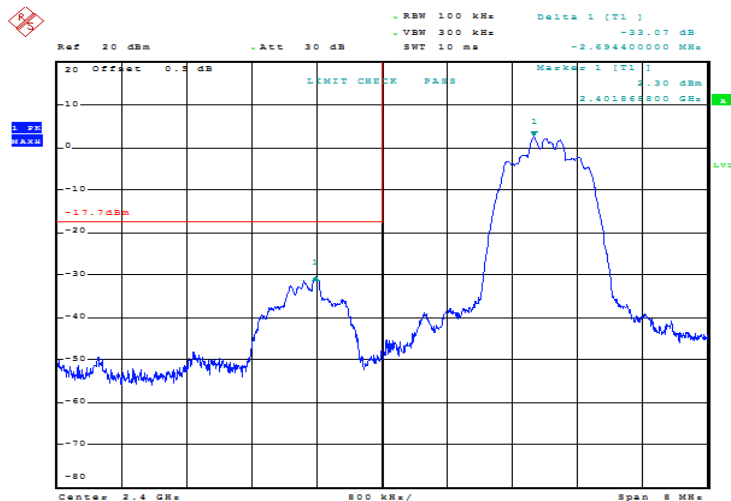
8DPSK_Low 33.07 dB
