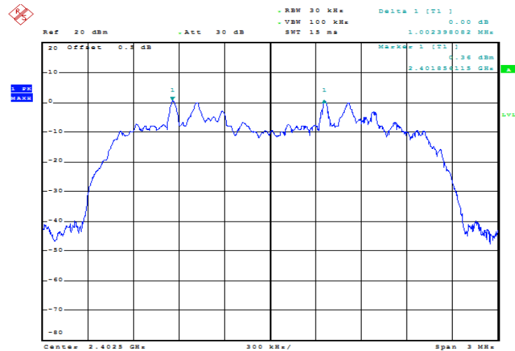
8DPSK_Low 1.002 MHz
