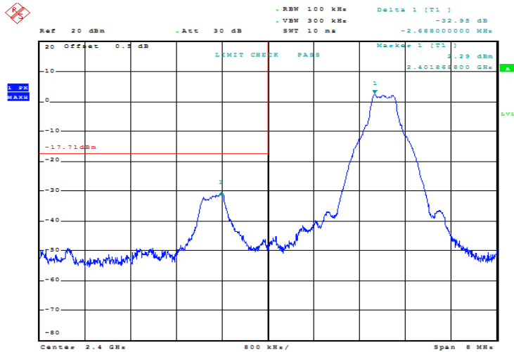
GFSK_Low 32.95 dB
