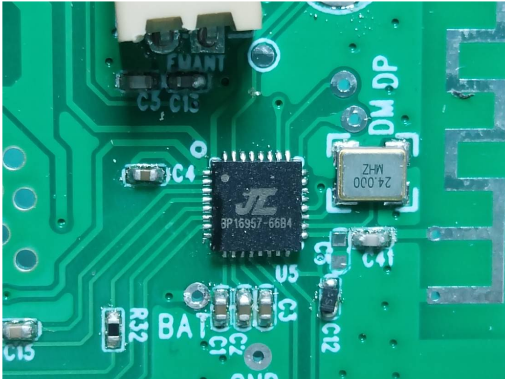
BT/BLE ANT
