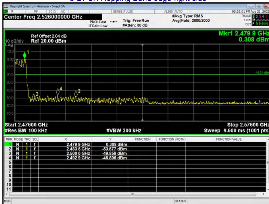
8-DPSK Hopping Band edge-right side
