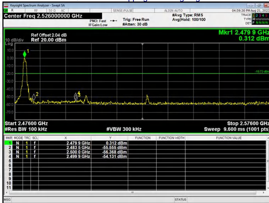
8-DPSK No-hopping Band edge-right side
